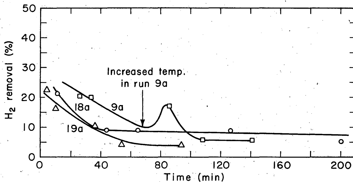
Fig. iv-39. Oxidation of H 2 with iron oxide.
