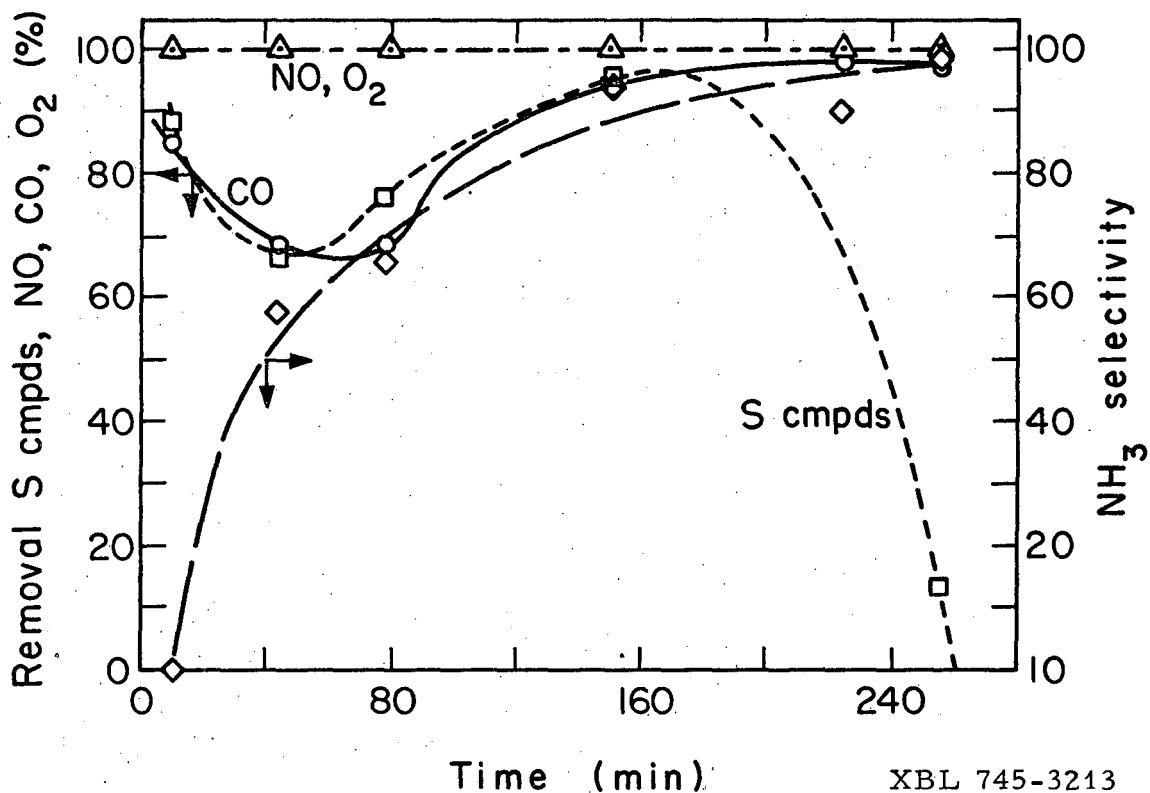
Fig. iv-34. Simultaneous removal of SO 2 , NO, CO, and O 2 over copper oxide catalyst.
