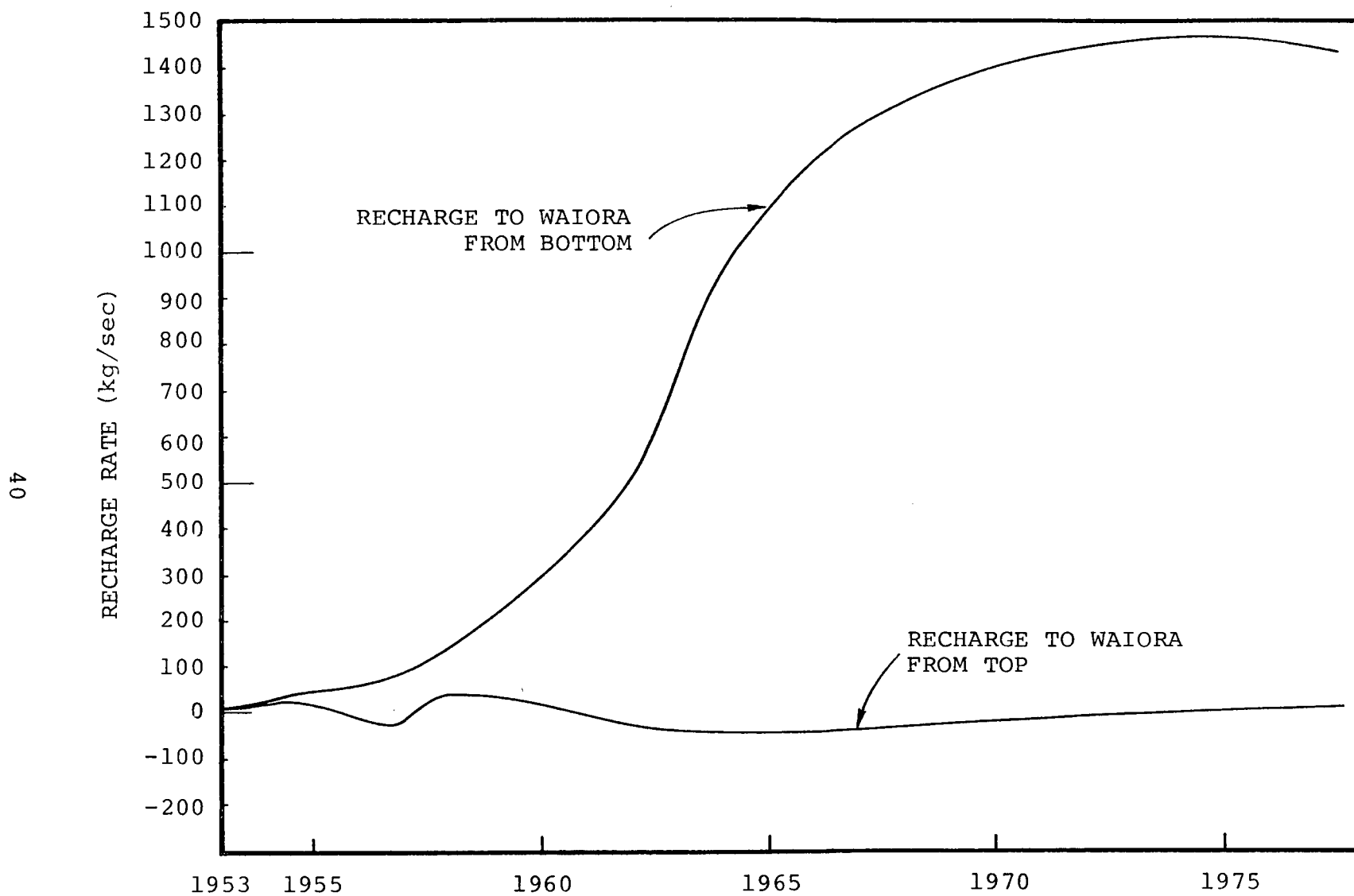
Figure 5.8. Recharge to Waiora Formation From Top (i.e., Huke Falls Formation) and Bottom (i.e., Ignimbrites).
