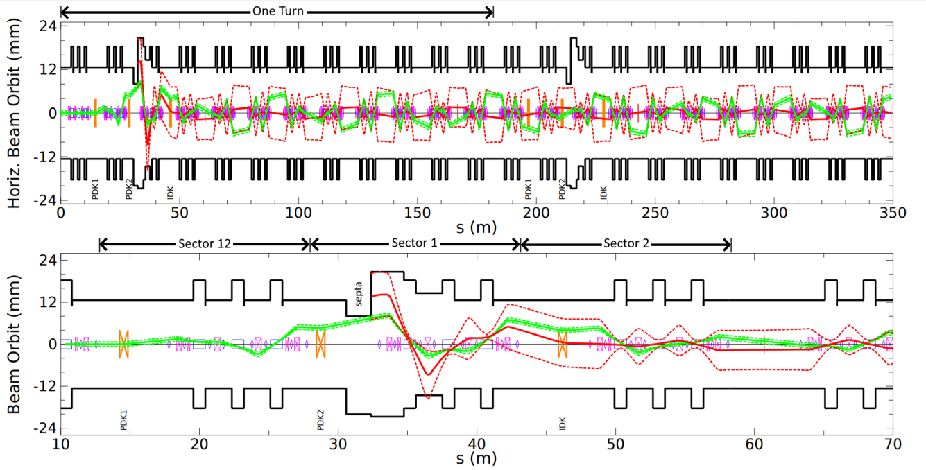
FIG. 4. Trajectories of the stored (green) and injected (red) beams during an injection cycle for the “balanced” mode kicker strength settings, also referred to as “Mode A”. Solid black profile indicates horizontal physical aperture. Dashed lines delineate 3\sigma of the beam size. Kickers are labeled and represented by orange bow-ties. The first pre-kicker is located at the start of sector 12. The second pre-kicker and injection septum are located in sector 1. The main injection kicker in sector 2 kicks both the stored and injected particles.
