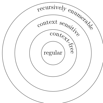
Figure 1.1: The four-level Chomsky Hierarchy
