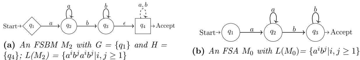
Figure 2.3: An example FSBM and the corresponding FSA for the base language
