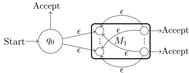
Figure 2.19: The construction used in the star operation
