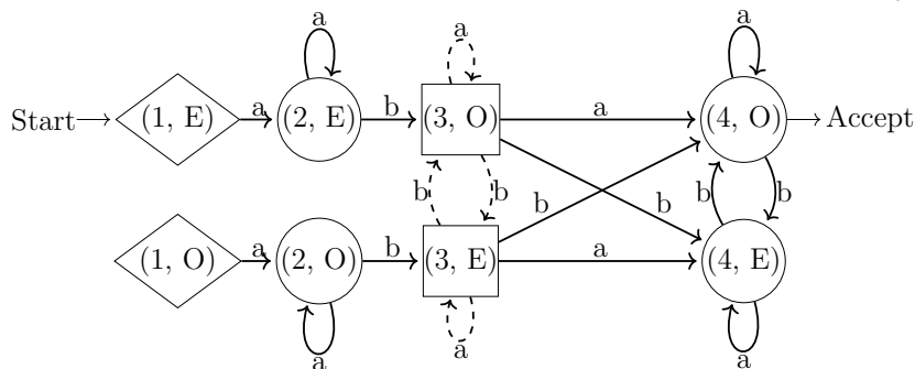
(c) the intersection FSBM after the construction: G = \{(1, E), (1, O)\} , H = \{(3, O), (3, E)\} .
