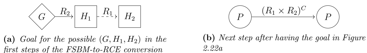
Figure 2.22: The conversion of the copying mechanism in an FSBM to RCE. P represents the plain, non- H , non- G states
