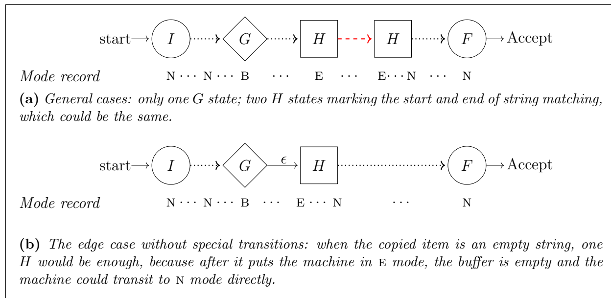
Figure 2.9: The template for the implementation of the copying in FSBMs. Key components: G state, H states, transitions between H states, and strict ordering between G and H . Solid lines represent a transition in one step. Dotted lines represent a sequence of normal transitions. Black dotted lines replace plain non- G non- H states. H states in between H states are replaced by red dashed lines.
