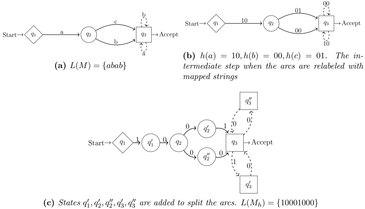
Figure 2.14: Constructions used for the homomorphic language in Theorem 3.
