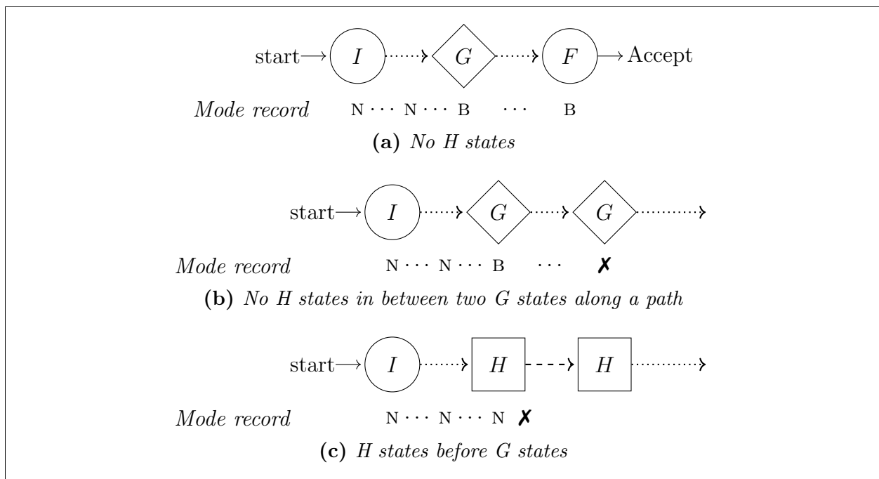
Figure 2.10: Possible paths in a machine failing on the completeness requirement. Dotted lines represent a sequence of normal transitions. Dashed lines are special transitions between H states in one step.
