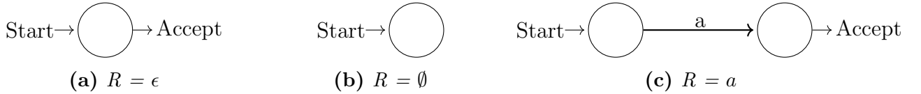
Figure 2.20: FSBMs for the base step in Theorem 5. All have G = \emptyset ; H = \emptyset
