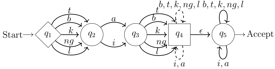
(b) An FSBM M_5 on the alphabet \{b, t, k, ng, l\} such that L(M_4) recovers the pattern of M_2 in Figure 2.6
