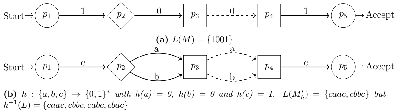
Figure 2.15: Under-generation of the conventional construction of the inverse homomorphic image
