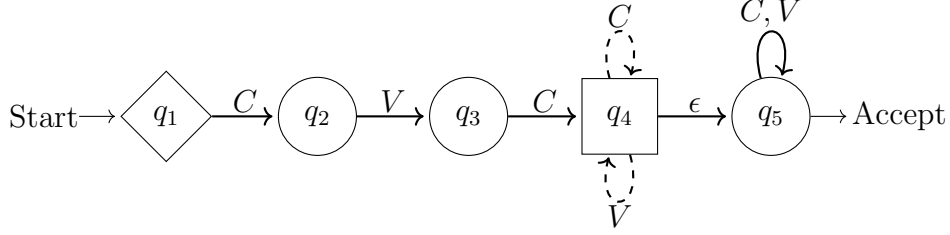
(a) An FSBM M_4 on the alphabet \{C, V\} such that L(M_4) = h(L(M_2)) with M_2 in Figure 2.6
