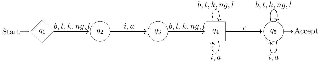
Figure 2.6: An FSBM M_3 for Agta CVC-reduplicated plurals: G = \{q_1\} and H = \{q_4\}
