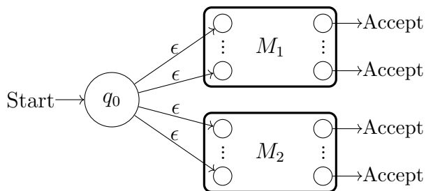
Figure 2.16: The construction used in the union of two FSBMs
