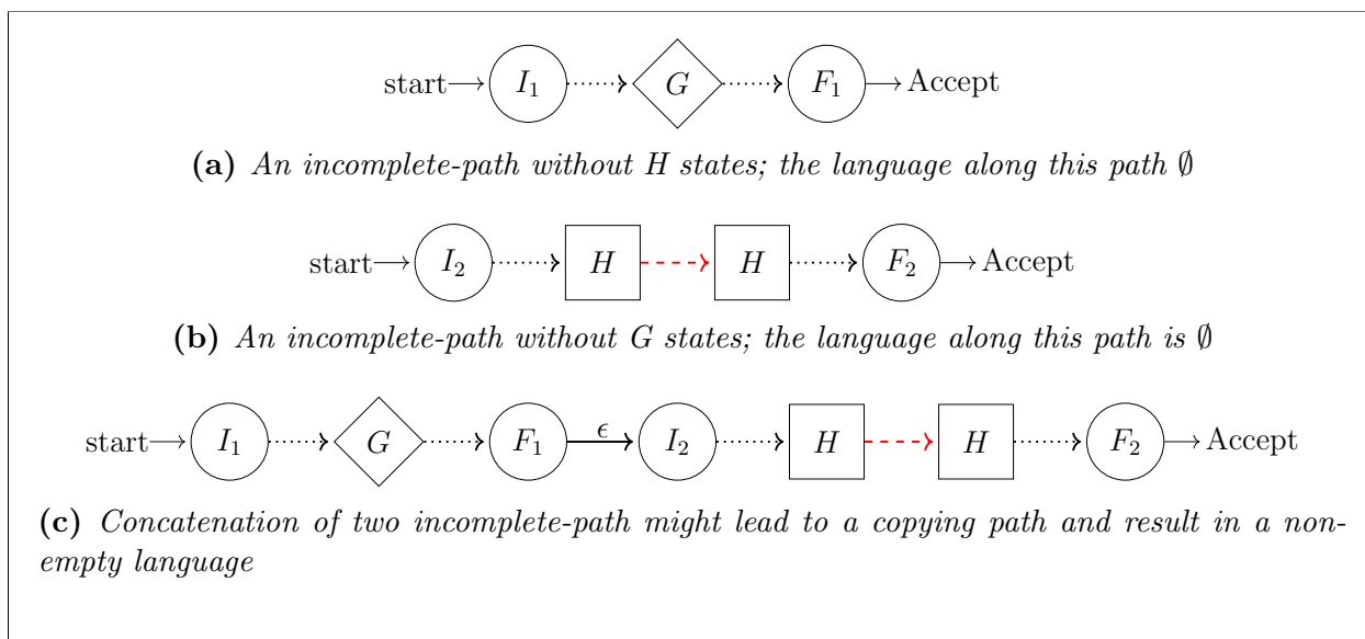
Figure 2.18: Problems arise in the concatenation of two incomplete paths. Dotted lines represent a sequence of normal transitions. Red dashed lines represent a sequence of special transitions
