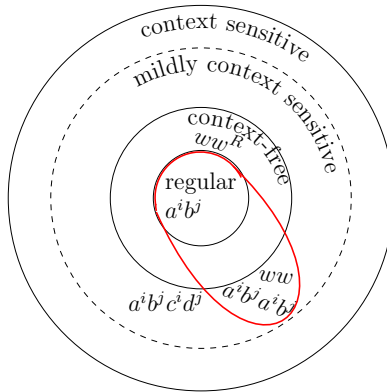
Figure 1.4: The class of regular+copying languages (red oval shape) in the Chomsky Hierarchy.
