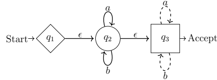
Figure 2.2: An FSBM M_1 with G = \{q_1\} and H = \{q_3\} . L(M_1) = \{ww \mid w \in \{a, b\}^*\}
