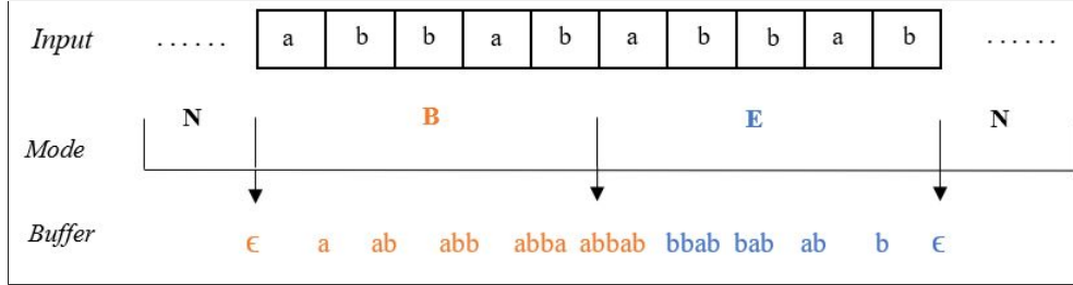
Figure 2.1: Mode changes and input-buffer interaction of an FSBM M on “...abbababbab...”. Assume M is armed with sufficient input consuming and symbol matching apparatus. The machine switches to B mode to temporarily store symbols in queue-like buffer. At the breaking point, it shifts to E mode for symbol matching between what’s in the buffer and what’s in the input. After all symbols matched, the buffer is emptied and the machine further switches to N mode.
