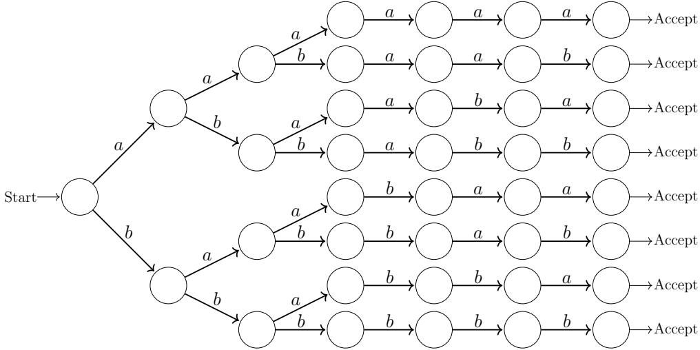
Figure 1.2: A finite-state machine for whole-base copying with the set of bases = \{aaa, aba, aab, abb, baa, bba, bab, bbb\}
