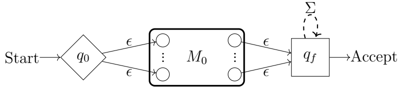
Figure 2.21: The construction used in converting the copy expression R_1^C to a finite state buffered machine. L(M_0) = L(R_1) .
