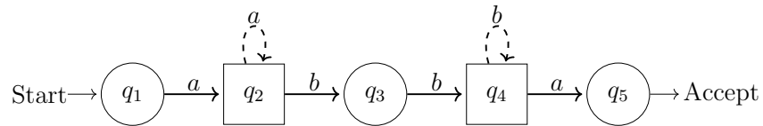
Figure 2.11: An incomplete FSBM M_4 with G = \emptyset and H = \{q_2, q_4\} ; L(M_4) = \{abba\}
