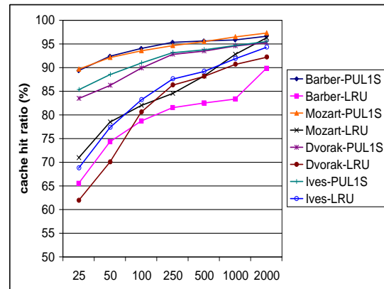
Figure 8. Cache hit ratio of LRU (labelled LRU) and LRU with PUL1S (labelled PUL1S)
