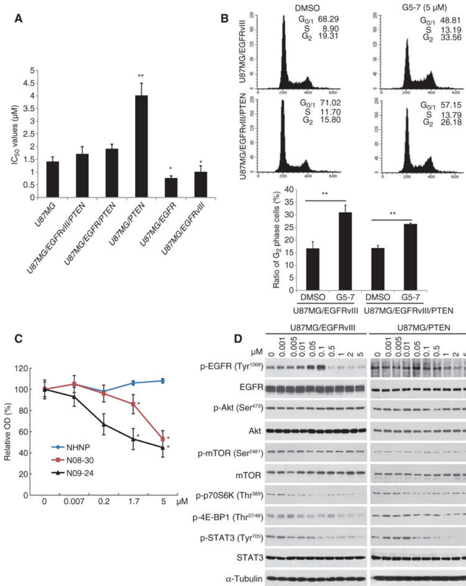
Fig. 2. G5-7 blocks EGFR phosphorylation and cell cycle at G 2 phase to inhibit cell proliferation (A) Proliferation of various U87MG cell lines treated with a range of doses of G5-7. Data are means \pm SEM ( *P < 0.05 , **P < 0.01 , versus IC 50 value of U87MG, one-way ANOVA, n = 3 ). (B) Cell cycle analysis of arrest at G 2 phase. One representative experiment of three is shown. Data are means \pm SEM ( **P < 0.01 , two-tailed Student's t test, n = 3 ). (C) Analysis of the proliferation of human GBM explant neurosphere cultures derived from glioma cell lines NHNP (wild-type PTEN, EGFR-deficient), N08-30 (PTEN-deficient, EGFRvIII amplification), and N09-24 (PTEN-deficient, EGFR amplification). Data are means \pm SEM ( *P < 0.05 , **P < 0.01 , one-way ANOVA, n = 4 ). (D) Western blot analysis of EGFR signaling in U87MG/EGFRvIII and U87MG/PTEN cells treated with different concentrations of G5-7 for 6 hours. Blots are representative of three experiments.
