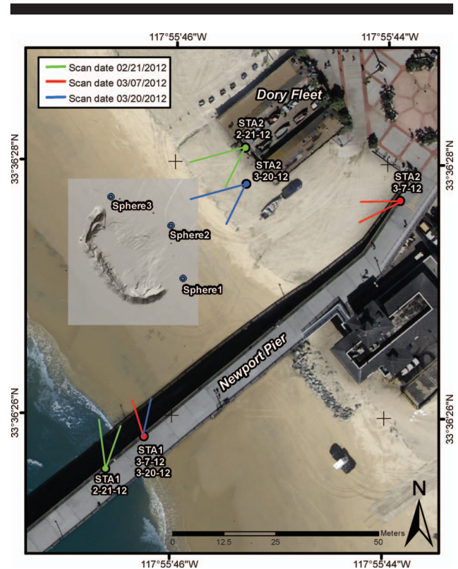
Figure 3. Berms were constructed next to Newport Pier to enable continuous scanning and time-lapse photography with an onshore perspective (front scan). Scans with an offshore perspective (back scans) were also completed to build a three-dimensional point cloud of each berm, and survey spheres (shown) were deployed to merge front and back scans in a postprocessing step. (Color for this figure is available in the online version of this paper.)
