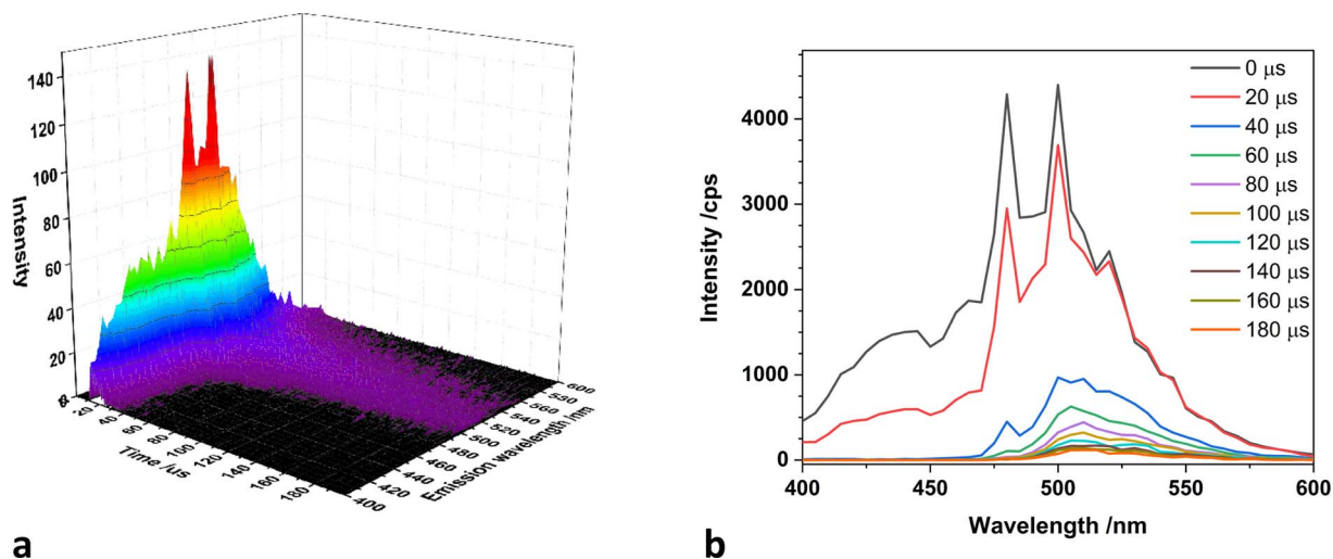
Fig. 4 (a) Time resolved emission spectra map and (b) spectra recorded with increasing time delay ( t ) of 1\text{-NO}_3 in MeCN at room temperature.
