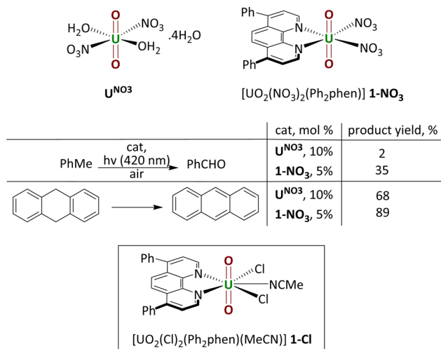
Fig. 1 Uranyl nitrate and the phenylphenanthroline (Ph 2 phen) adduct that we reported previously (upper); a comparison of their capacity as pre-catalysts for hydrocarbon oxidation (center); and the Ph 2 phen adduct of uranyl chloride also studied as a pre-catalyst in this work (lower).
