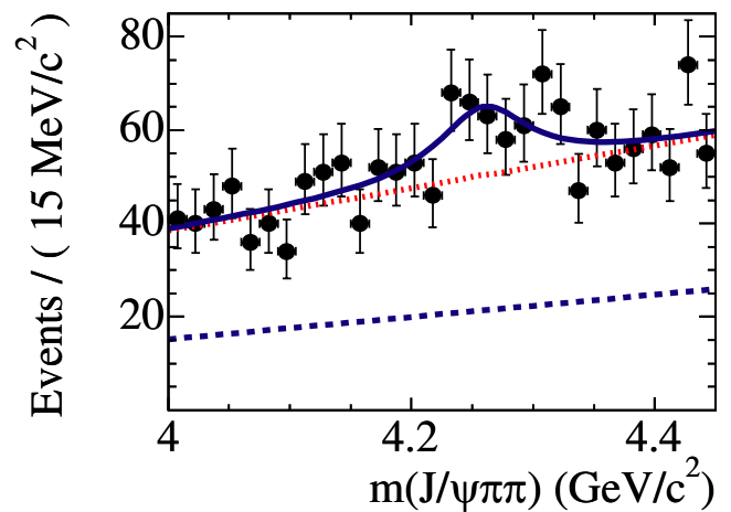
FIG. 2 (color online). Projection of the two-dimensional fit for the mass region above 4 \text{ GeV}/c^2 for events within the m_{\text{ES}} signal region in B^- \rightarrow J/\psi \pi^+ \pi^- K^- . The lines represent the same event types as in Fig. 1.
