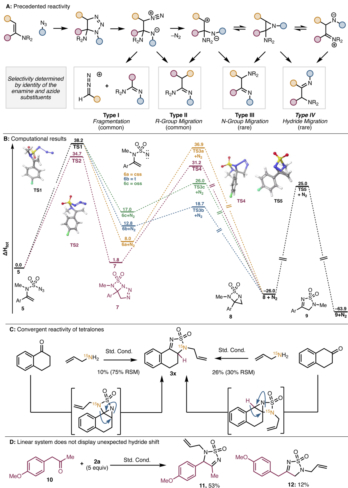
Fig. 2 (A) Rearrangements of amino-triazolones. (B) DFT investigation of possible reaction pathways (values given in kcal mol -1 ). (C) Reactivity of tetralone substrates (css: closed shell singlet. oss: open shell singlet. t: triplet).
