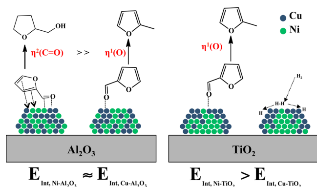
Figure 10. Schematic diagram of the proposed operating states of Cu–Ni bimetallic catalysts on \text{Al}_2\text{O}_3 and \text{TiO}_2 . For Cu–Ni/ \text{Al}_2\text{O}_3 , significant exposure of extended Ni domains drives efficient ring hydrogenation to form THFOL, whereas the segregated structure of Cu–Ni on \text{TiO}_2 facilitates MF formation. E_{\text{INT}} : Energy of interaction between metal (either Ni or Cu) and support ( \text{Al}_2\text{O}_3 and \text{TiO}_2 ).
