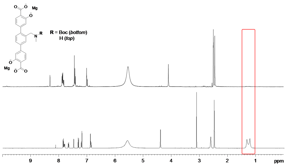
Figure S9. Comparison of ^1\text{H} NMR spectra for digested secondary amine functionalized IRMOF-74-III samples in 50 mM DCl/DMSO- d_6 /D _2 O mixture: IRMOF-74-III-CH _2 NMeBoc (bottom) and IRMOF-74-III-CH _2 NHMe (top); before and after microwave deprotection respectively.
