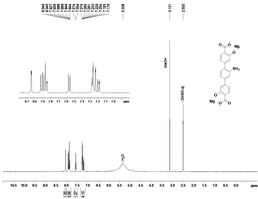
Figure S5. 1 H NMR spectra of IRMOF-74-III-NH 2 digested sample in 50 mM DCl/DMSO- d 6 /D 2 O mixture. Inset, expanded aromatic region in the spectra.
