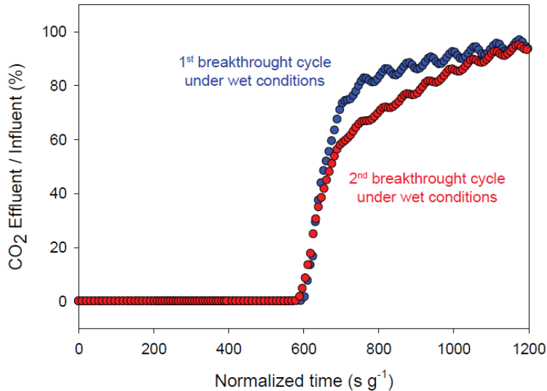
Figure S22. Breakthrough curves of IRMOF-74-III-CH 2 NH 2 in the presence of water after vapor saturation (i.e. first cycle, blue) and after recovery of the material by passing through nitrogen and heating at 90 °C for 30 minutes (second cycle, red). The breakthrough times are nearly identical.
