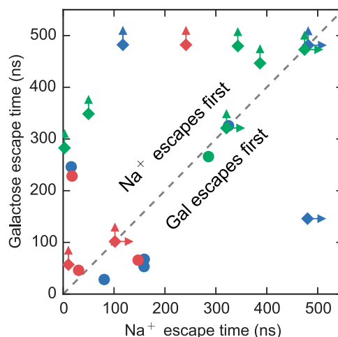
Fig. 2. Lifetimes of bound states for galactose and Na + . Scatter plot of time of release of galactose and Na + from the sugar and Na2 binding sites, respectively, for each simulation. Trajectories originating from the same initial model of vSGLT (as described in ref. 21) are shown as distinct colors. Simulations that were terminated before full unloading of sugar and/or Na + are represented by diamonds with one or two arrows indicating that Na + (right arrow) and/or galactose (up arrow) is still bound. We posit that galactose failing to exit before the simulations ended is a function of the simulation timescale and not due to any structural constraints. All other trajectories are shown as circles.
