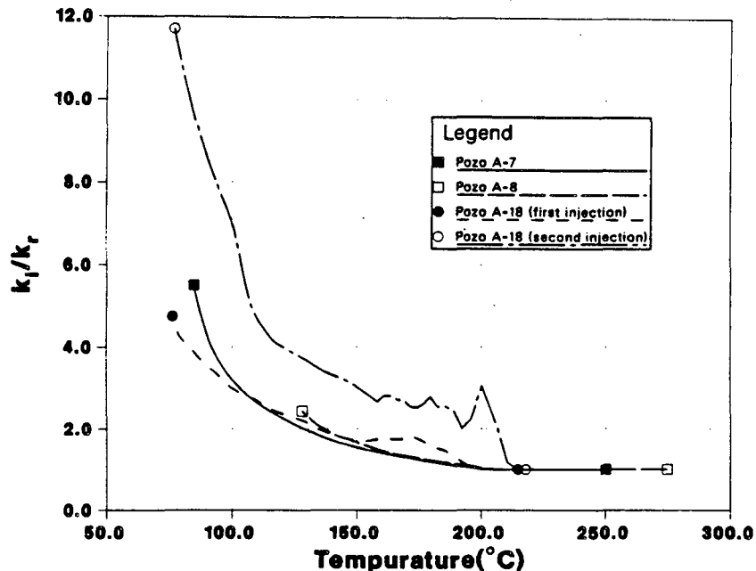
Figure 9. Permeability enhancement plotted as a function of the sandface injection temperature for four injection tests.
