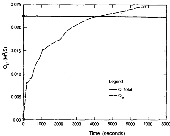
Figure 2. Sandface flowrate during the well A-7 injection test.
