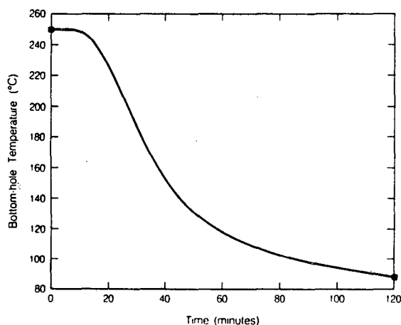
Figure 3. Simulated sandface temperature during the well A-7 injection test.
