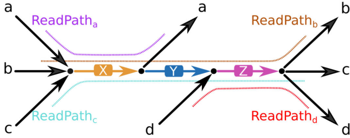
(c) Superbubble
