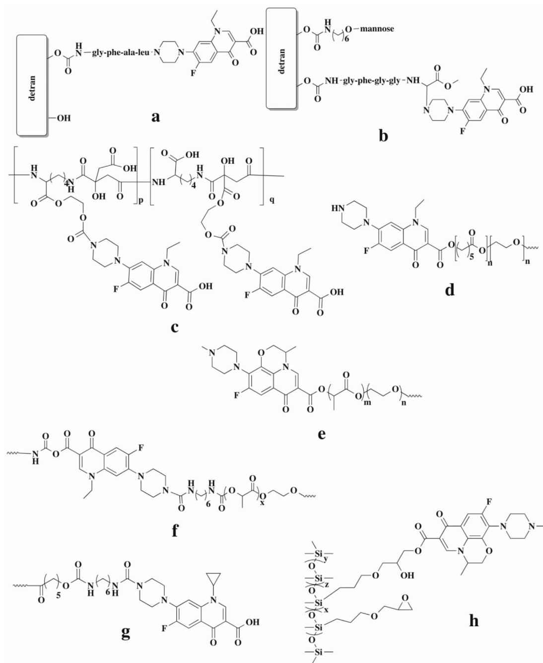
Figure 2. Dextran-peptide norfloroxacin conjugate (a), mannosylated dextran-peptide norfloroxacin conjugate (b), poly(L-lysine citramide imide) derivative with carbamate linking norfloroxacin (c), PEG-PCL-norfloroxacin polyester fragment (d), PEG-PLA-ofloxacin polyester fragment (e), PEG-PLA-norfloroxacin polyurethane fragment (f), PCL-ciprofloxacin polyurethane (g), polydimethylsiloxane-epoxy-levofloxacin conjugate (h)
