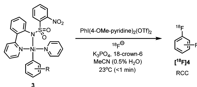
Scheme 5. Oxidative Fluorination of Nickel(II) \sigma -Aryl Complexes a
