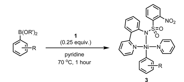
Scheme 4. Synthesis of Nickel(II) \sigma -Aryl Complexes by Transmetalation from Boronic Acids and Esters a
