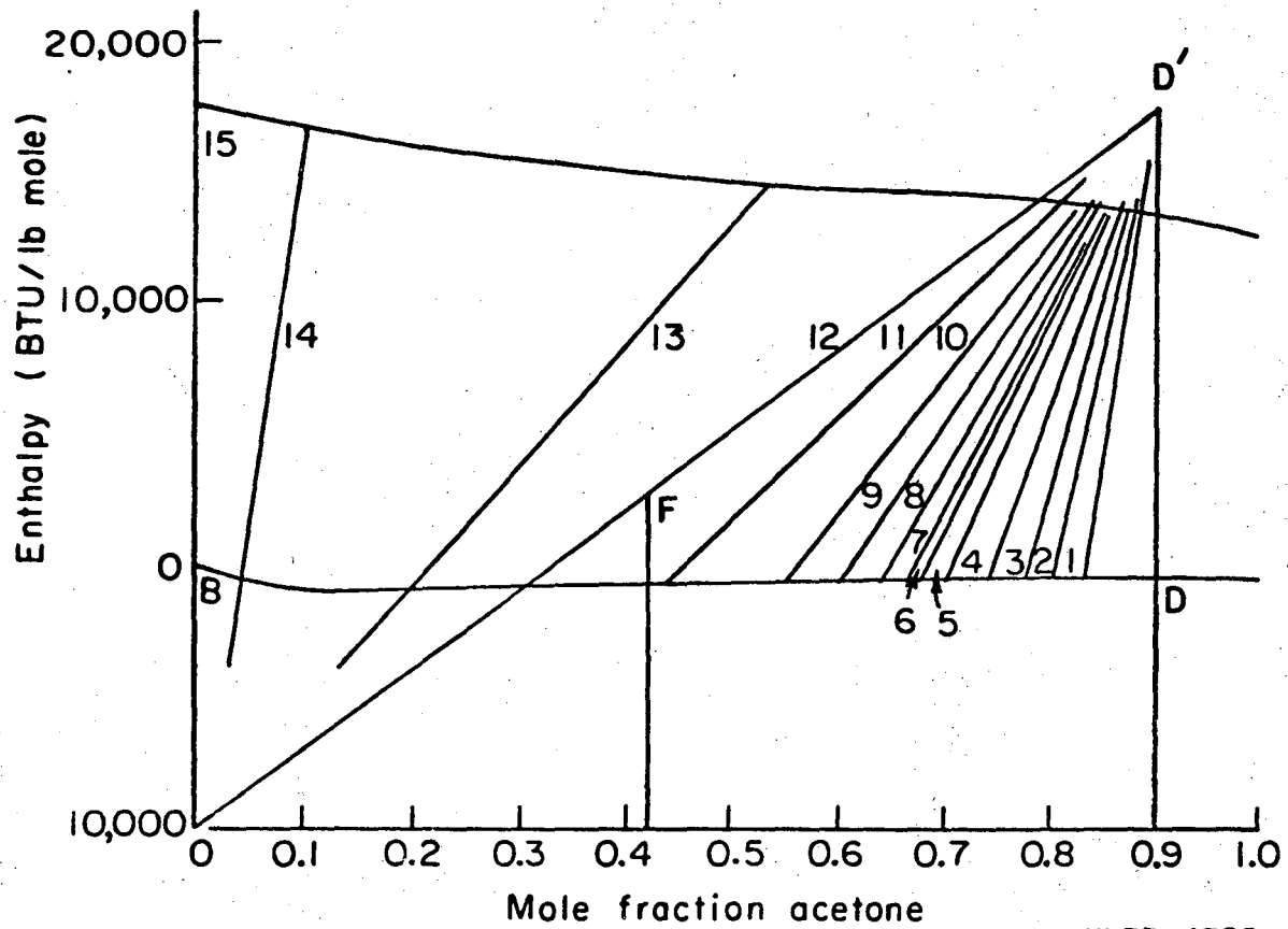
Fig. 38. Enthalpy-concentration diagram for acetone-water system.
