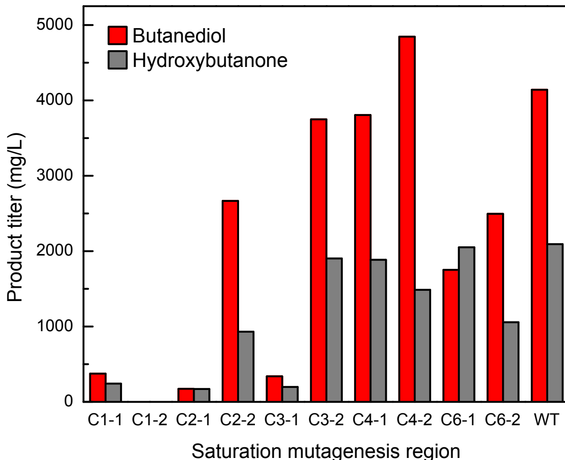
Figure 4.17 ALDH saturation mutagenesis improves butanediol titer and product mixture Aldh7 mutant libraries were produced with saturation mutagenesis and selected through anaerobic growth. Titters at the endpoint of selection were highly variable and some cultures had lost all productivity. However, culture C4-2, containing a library targeting residues 445-447 (Thr-Phe-Thr, see Figure 4.16, blue region), produced 5 g/L butanediol and 1.5 g/L hydroxybutanone. This compares favorably to the wild type, which produced 4 g/L butanediol and 2 g/L hydroxybutanone, and the combined titer of 6.5 g/L is our highest achieved to date. Upon sequencing, clones in this culture were found to contain Thr445 mutated to serine or glycine. In the wild type structure Thr445 is 7.7 Å from the active site Cys279 and forms the opposite wall of the active site. Thr445 makes close contacts with two other loops that further define the active site cavity opposite the catalytic cysteine.
