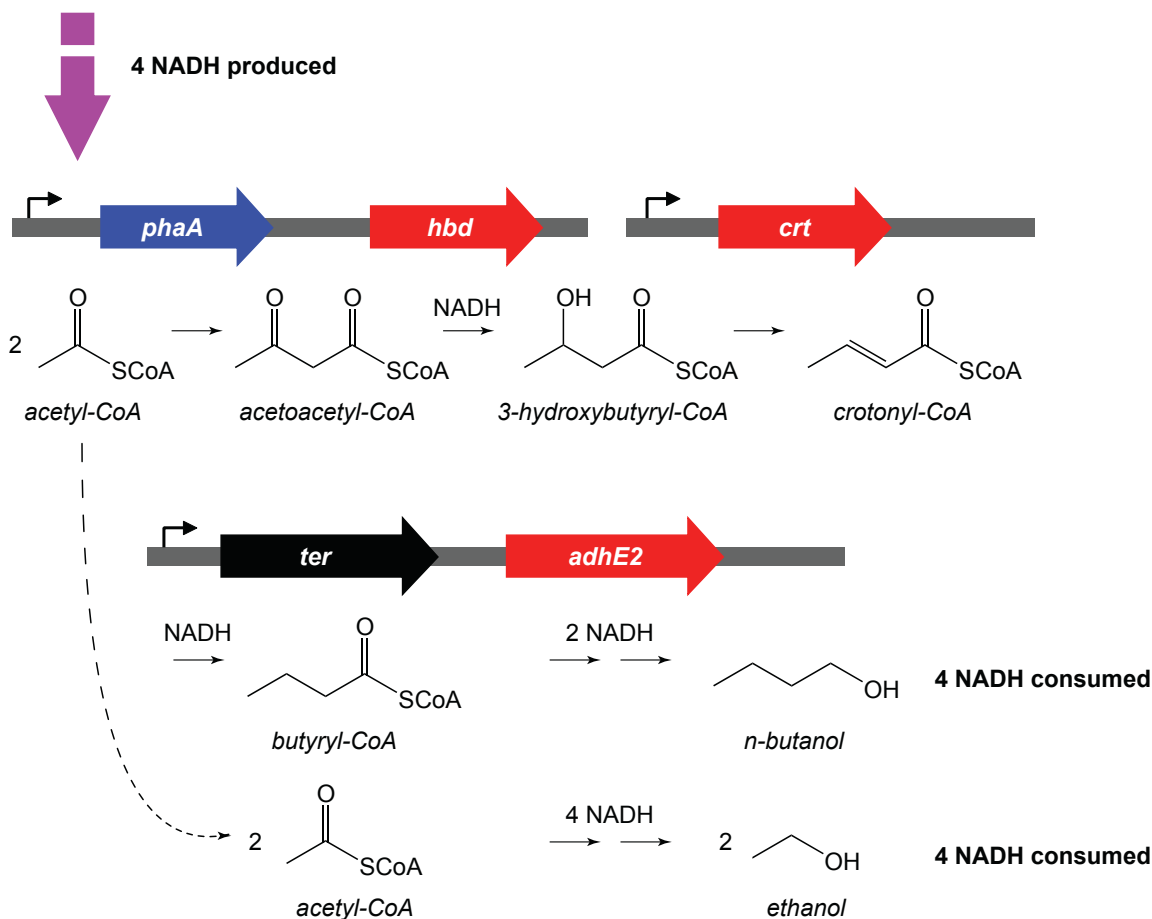
Figure 2.9 Pathway side products due to low substrate specificity
