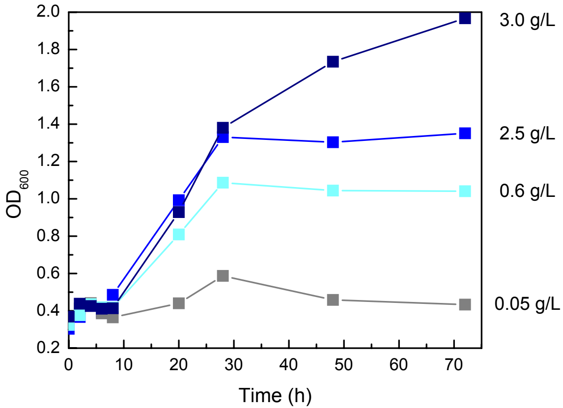
Figure 3.9 Butanol production rescues growth in fermentation deficient cells
