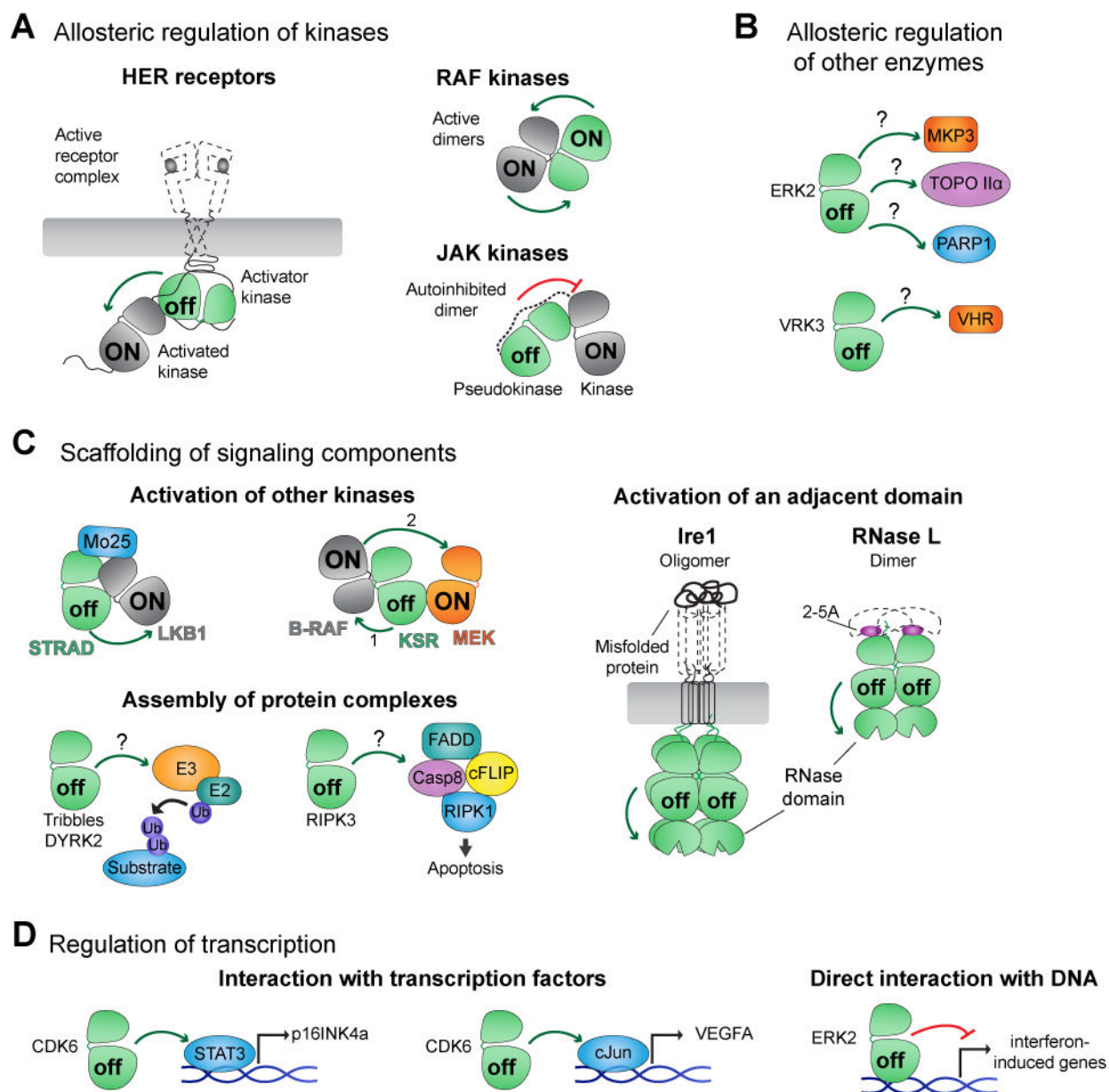
Figure 2. Non-catalytic functions of protein kinases
