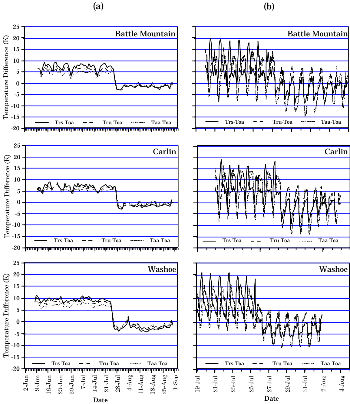
Figure 11. Daily average [a] and hourly [b] rises of roof surface temperature Trs, roof under-surface temperature Tru, and attic air temperature Taa above outside air temperature Toa. Hourly plots include a week before and after the roof was coated.
