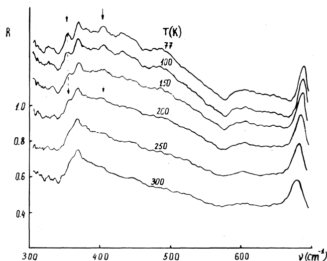
FIG. 7. Temperature dependence of the reflectivity spectrum from the basal plane of \text{La}_2\text{CuO}_{4+x} . The R axis corresponds to curve measured at 300 K. Other curves are shifted along R axis by step \sim 0.1 .
