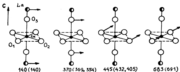
FIG. 6. Schematic presentation of the E_u symmetry vibrations in the tetragonal \text{La}_2\text{CuO}_{4+x} and the corresponding frequencies at T=300\text{ K} , in parentheses at T=77\text{ K} .
