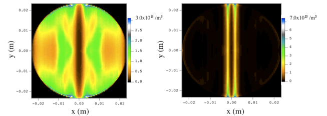
Figure 2: Density distribution for a resonant (0.07T) and non-resonant (0.08T) case. Vacuum chamber is circular and fits exactly within the plot.
