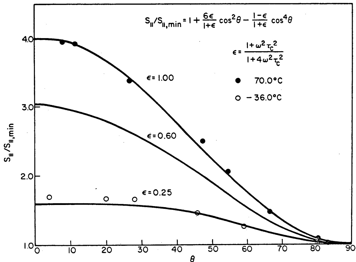
Fig. VIII.3 The angular dependence of the spin-lattice relaxation rate at two temperatures ( -36^\circ\text{C} and 70^\circ\text{C} ) is shown along with the theoretical fit (solid line) for three different values of the parameter \epsilon defined in the figure. \epsilon = 0.25 corresponds to the low temperature limit (i.e. \omega^2 \tau_c^2 \gg 1 ) and \epsilon = 1.00 corresponds to the high temperature limit (i.e. \omega^2 \tau_c^2 \ll 1 ).
