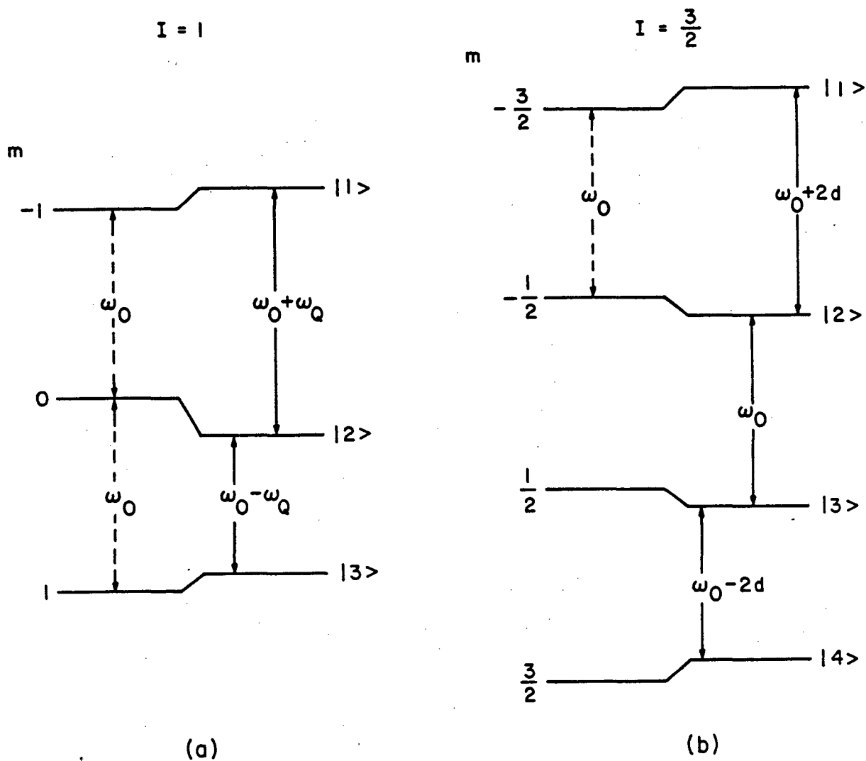
Figure III.5 Energy level diagrams of spin-1 and spin-3/2 particles.
