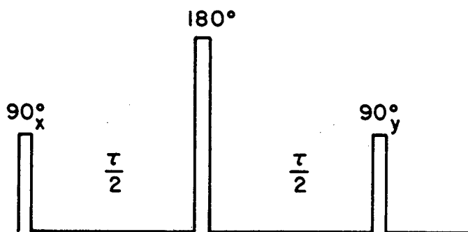
Figure III.4 Pulse sequence for selective excitation of even-quantum and odd-quantum coherence. The phase of the 180^\circ pulse is arbitrary.
