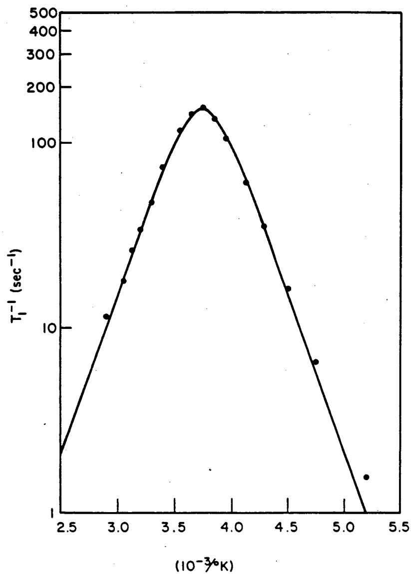
Figure VIII.4 The temperature dependence of the spin-lattice relaxation rate for the HMB- \text{d}_{18} single crystal oriented with all molecular \text{C}_6 axes parallel to the magnetic field. The solid curve is the best fit of equation VIII.7 to the data.
