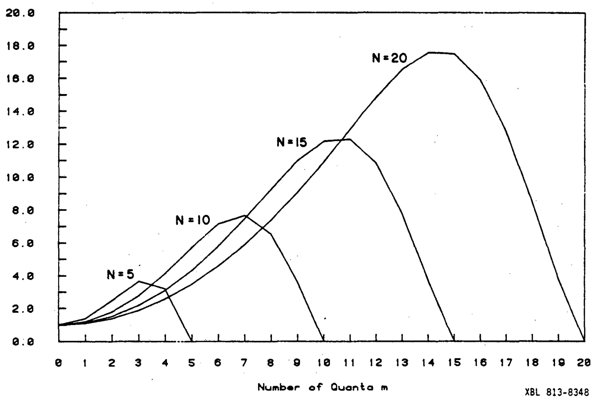
Figure VI.10 Normalized dependence of \langle \Omega^2 \rangle_m on m for N = 5 , 10, 15, and 20.
