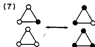
Figure V.4 Allowed 4-quantum transitions for the case of correlated motion. Seven 4-quantum transitions are expected. Since there are two intermethyl couplings, the configuration in (2) is different from the configuration in (3).
