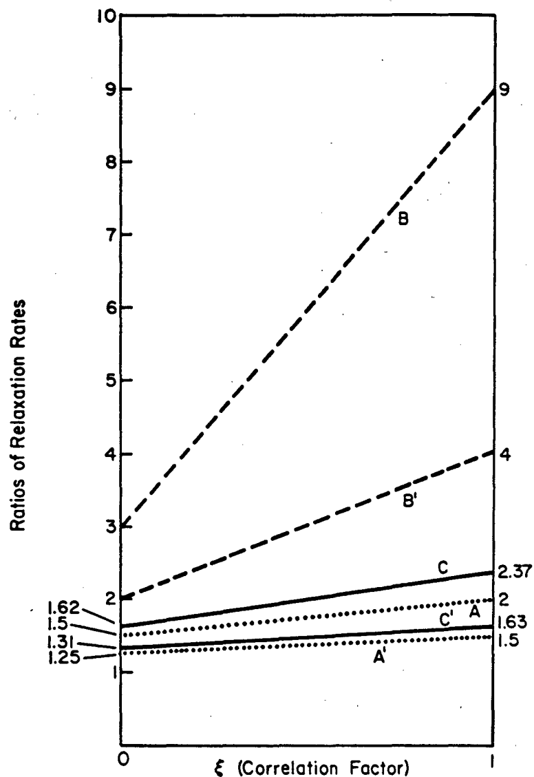
Fig. IV.6 The ratios of relaxation rates of double and triple quantum coherences to single quantum \Gamma_{13}/\Gamma_{12} and \Gamma_{14}/\Gamma_{12} depends on the correlation factor \xi and the correlation time \tau_c . Curves A and A' show the case of short correlation time limit, \omega_s^2 \tau_c^2 \ll 1 . Lines B and B' show the case of long correlation time limit, \omega_I^2 \tau_c^2 \gg 1 . The intermediate case, \omega_I^2 \tau_c^2 \ll 1 , \omega_s^2 \tau_c^2 \gg 1 , is shown by curves C and C'.
