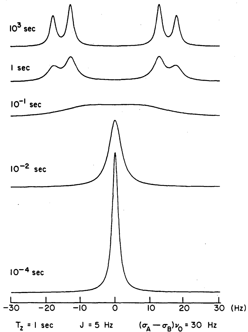
Figure V.12 Theoretical spectra of a J-coupled AB system. The molecule undergoes chemical exchange with a correlation time \tau_c from 10^3 sec to 10^{-4} sec.
