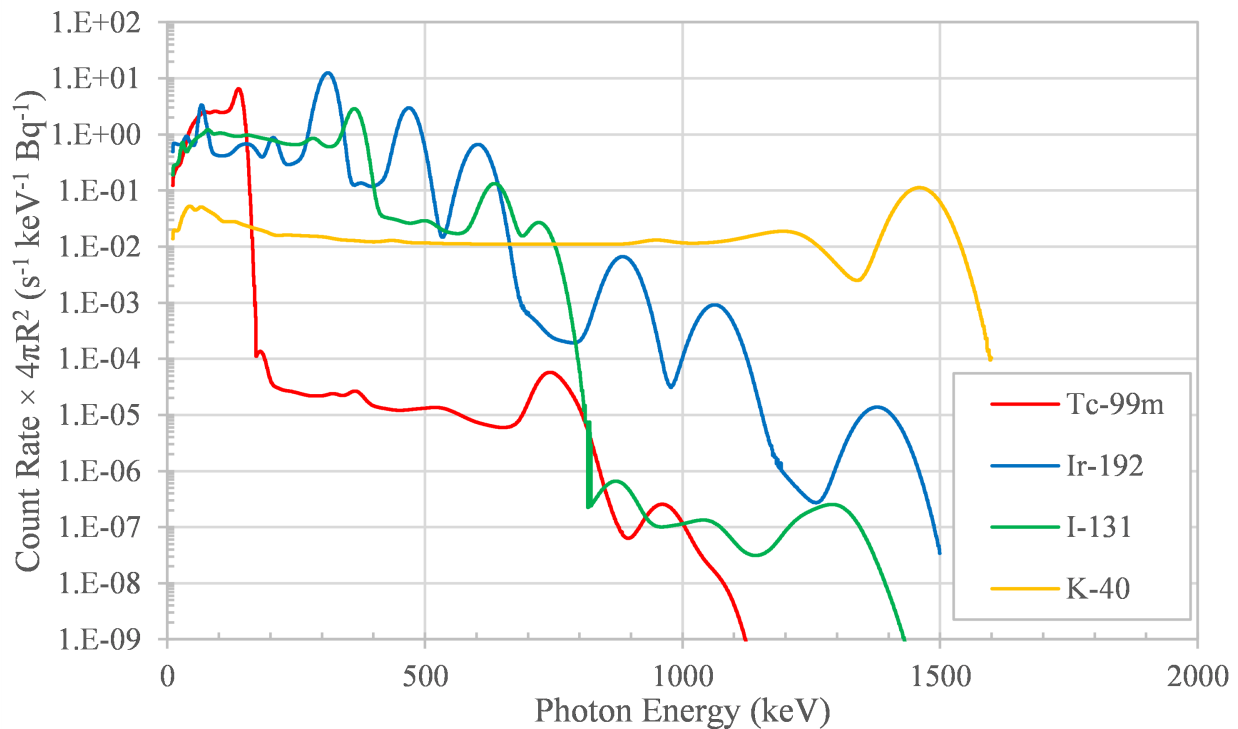
Figure 9: Simulated 2'' \times 4'' \times 16'' NaI(Tl) responses for point sources of ^{99\text{m}}\text{Tc} , ^{192}\text{Ir} , ^{131}\text{I} and ^{40}\text{K} .
