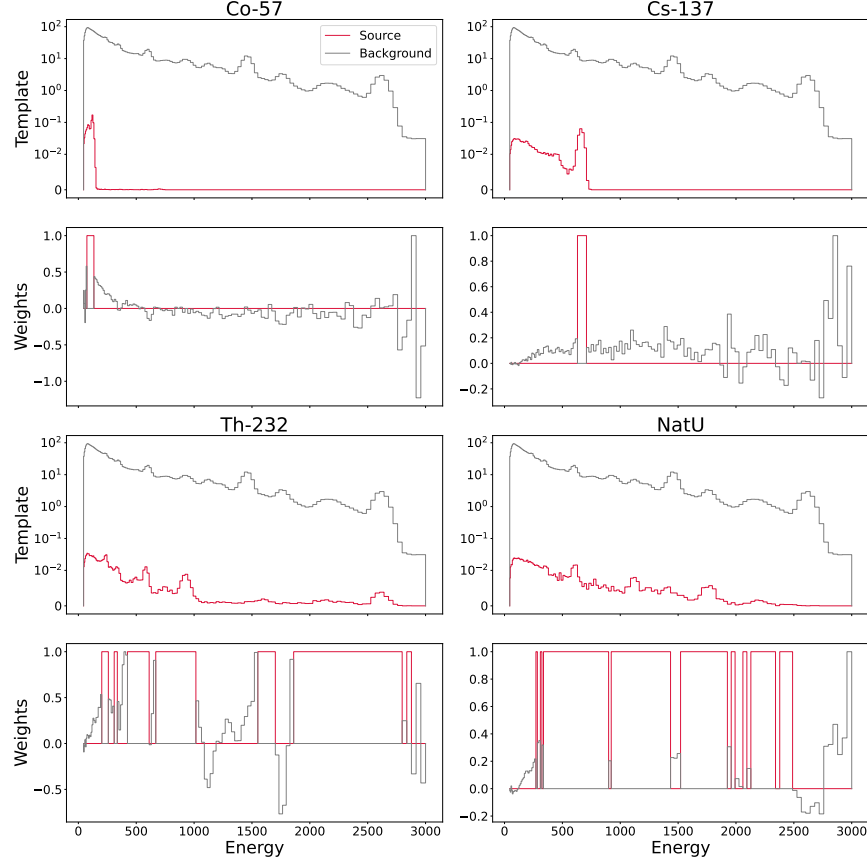
Figure 16: Examples of windows determined by assigning weights to regions of the spectrum that are associated with sources (red) or background (black), found using multiplexed censored energy window (mCEW). The windows for ^{137}\text{Cs} and ^{57}\text{Co} are narrow and well-defined whereas those found for ^{232}\text{Th} and natural Uranium span nearly the entire range of energies.
