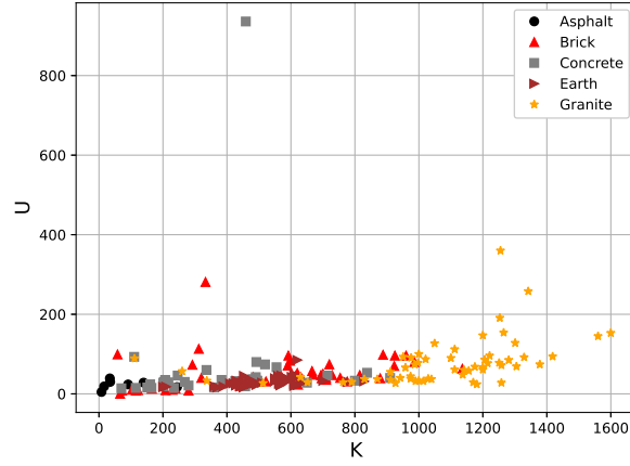
(a) K vs U
