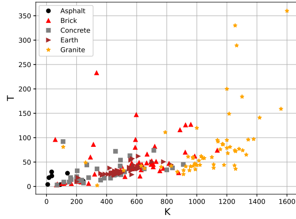
(b) K vs Th
