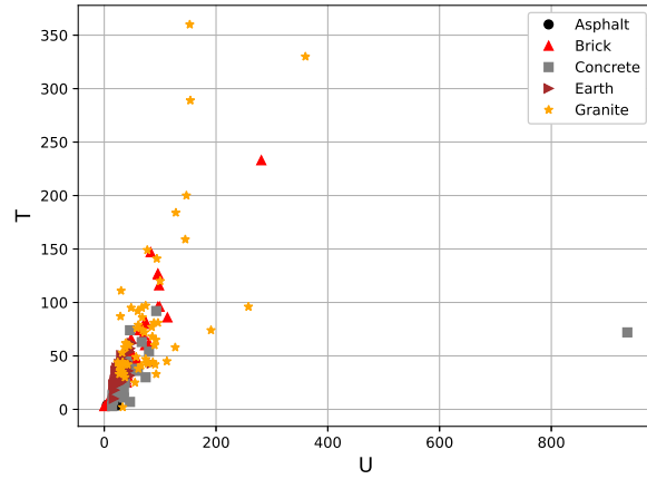
(c) U vs Th
