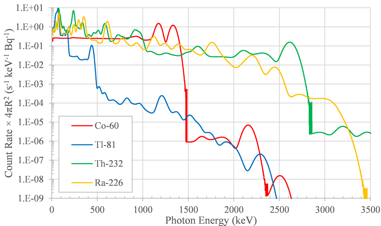
Figure 10: Simulated 2'' \times 4'' \times 16'' NaI(Tl) responses for point sources of ^{60}\text{Co} , ^{201}\text{Tl} , ^{232}\text{Th} , and ^{226}\text{Ra} .
