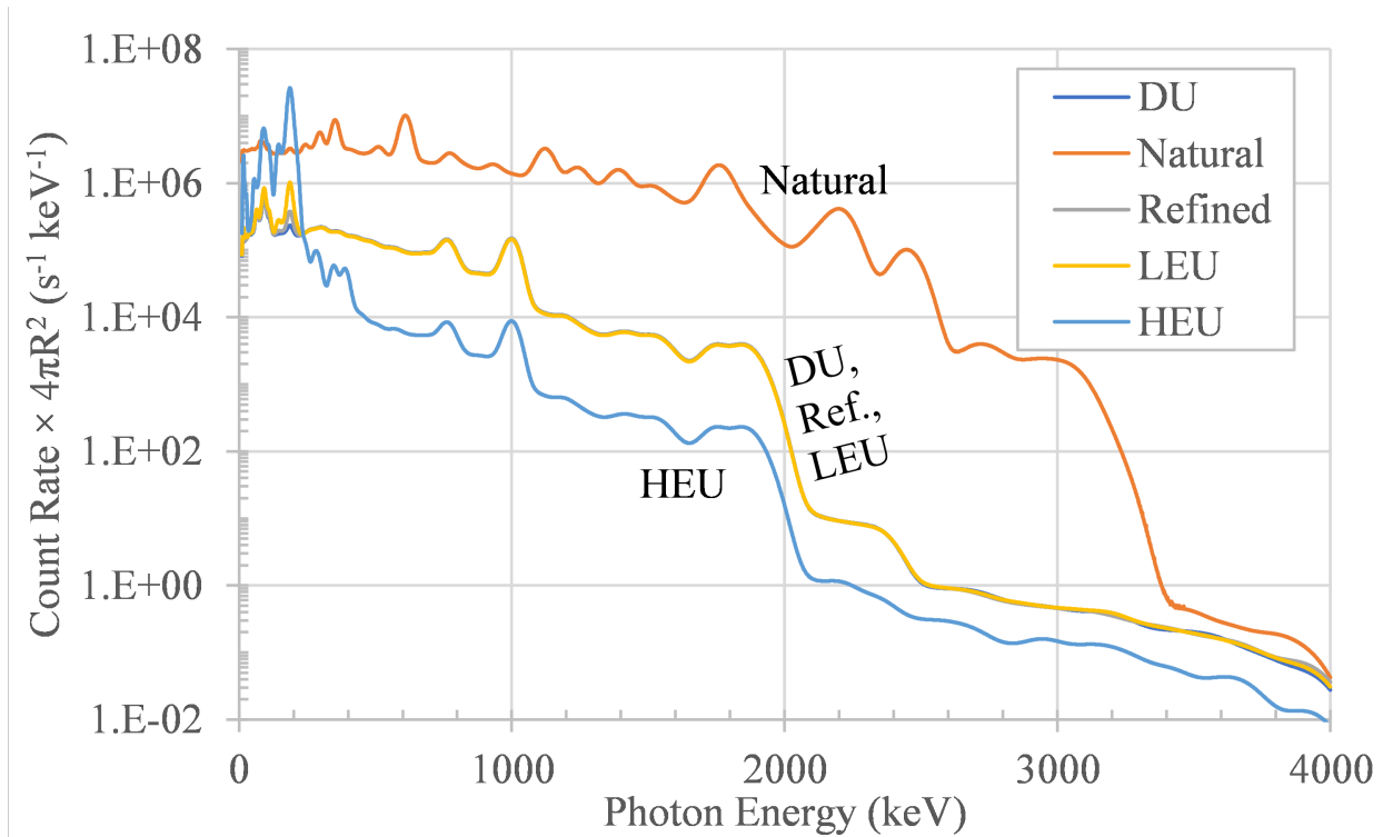
Figure 12: Simulated 2'' \times 4'' \times 16'' NaI(Tl) responses 5kg of different types of uranium. Note, depleted-, refined-, and low-enriched-uranium spectra are nearly overlapping.
