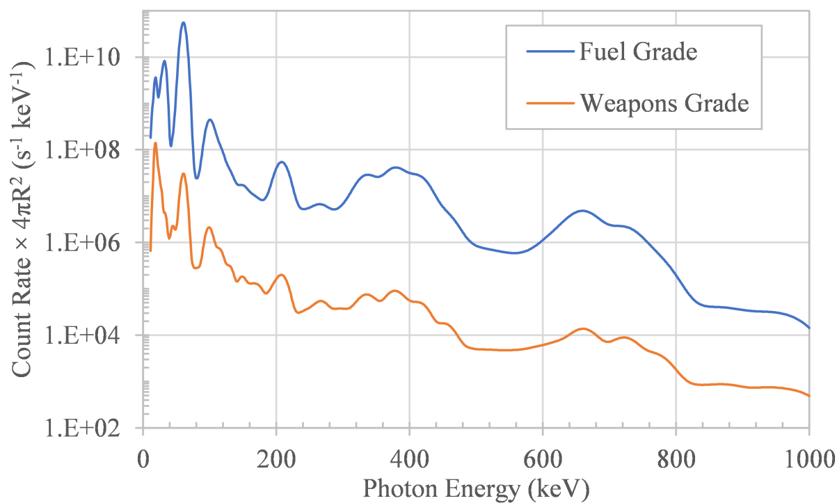
Figure 11: Simulated 2'' \times 4'' \times 16'' NaI(Tl) responses 2 kg of fuel grade and 2 kg of weapons grade plutonium.
