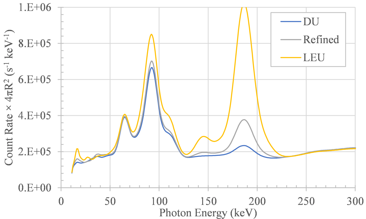
Figure 13: Simulated 2'' \times 4'' \times 16'' NaI(Tl) responses 5kg of low-enriched uranium zoomed-in on lower energies.
