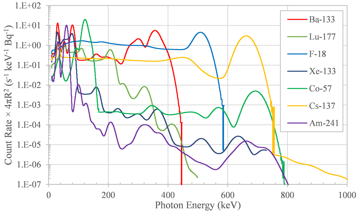
Figure 8: Simulated 2'' \times 4'' \times 16'' NaI(Tl) responses for point sources of ^{133}\text{Ba} , ^{18}\text{F} , ^{57}\text{Co} , ^{137}\text{Cs} and ^{241}\text{Am} .
