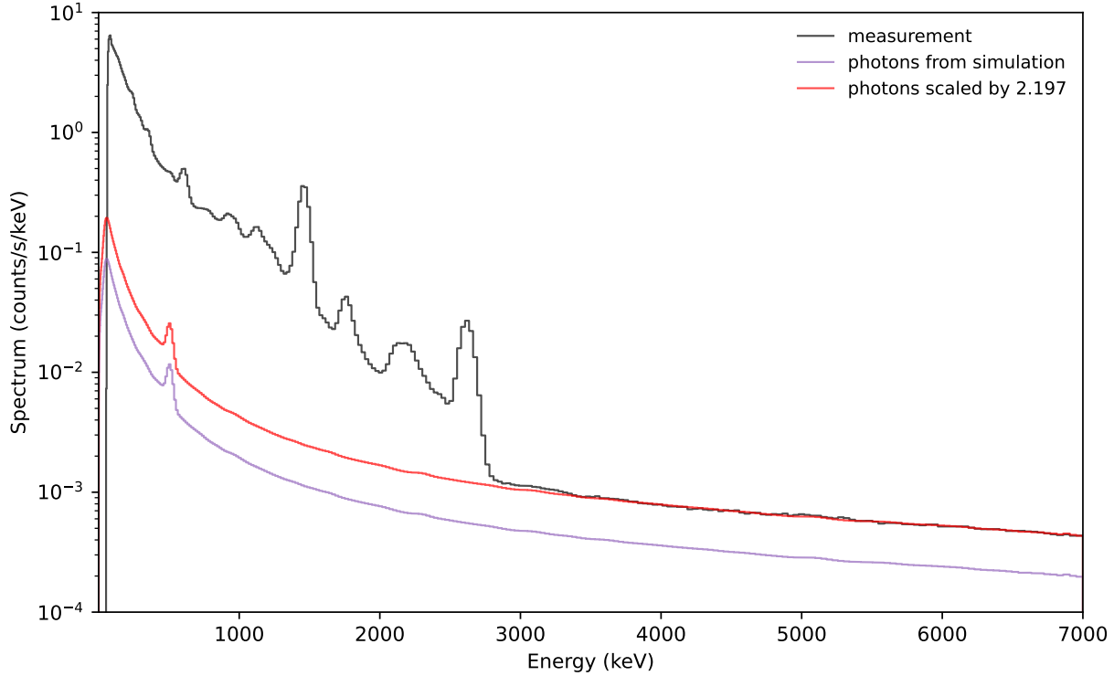
Figure 5: Measured 2'' \times 4'' \times 16'' NaI(Tl) data from the roof of LBNL Building 50B, shown with the results of the cosmic-ray secondary photon simulations (magenta) and the scaled photon spectrum (red). Detector energy resolution has been applied to the simulation.
