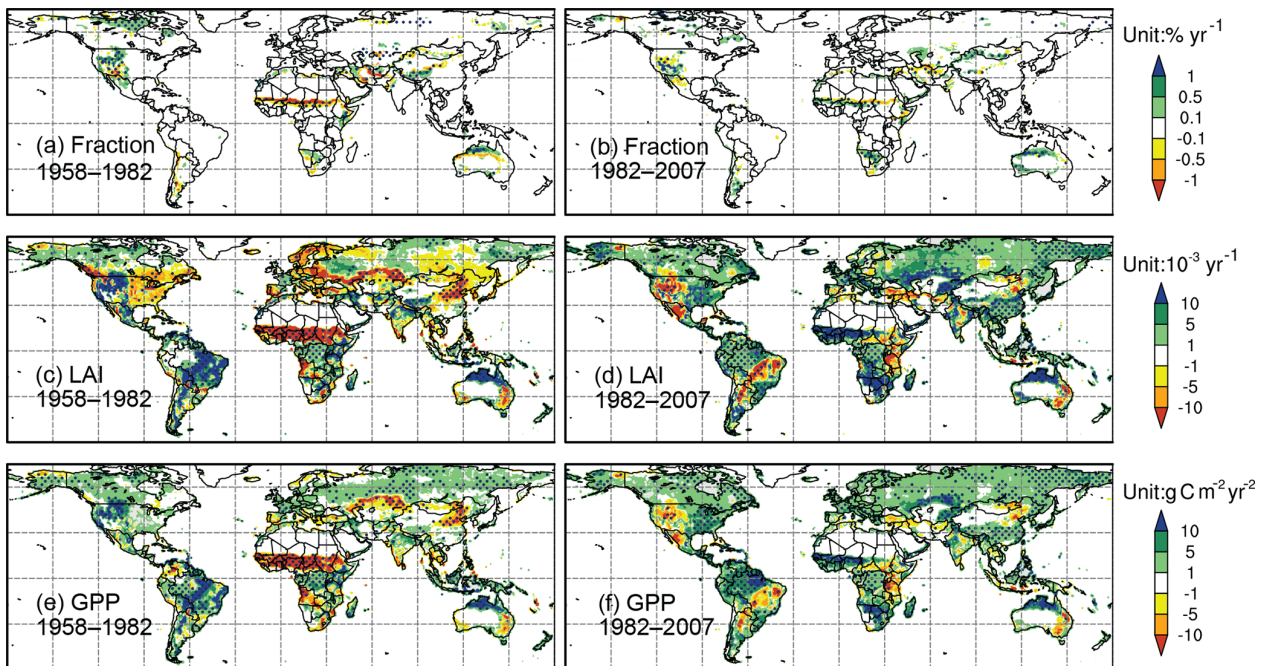
Figure 7. Trends (shaded) of (a, b) fractional coverage (units: % yr -1 ), (c, d) LAI (units: 10 -3 yr -1 ), and (e, f) GPP (units: g C m -2 yr -2 ). Panels (a, c, e) are for 1958–1982 and (b, d, f) are for 1982–2007. The dots indicate the areas with significance level at P < 0.05 (Mann–Kendall test).
