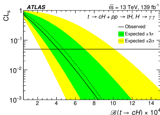
Figure 10. Evolution of the signal confidence level, CL_s , as a function of the t \rightarrow cH branching ratio B for the observation (full line) and the expectation in the absence of signal (dashed line). The bands at \pm 1\sigma and \pm 2\sigma around the expected curve are also shown.
