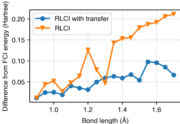
Figure 6. Symmetric dissociation of a \text{H}_8 ring using the STO-6G basis, with and without transferring the wave function and associated weights. In this case, the dimension of the subspace k = 120 determinants, approximately 2.5% of the full Hilbert space. The RLCI method with transfer is able to achieve smaller error with respect to FCI energies with fewer iterations for the majority of the points considered. Both dissociation curves begin at the same bond length of 0.9 Å, which is run for 30 episodes. For subsequent points along the potential energy curve, the geometry is incremented in steps of 0.05 Å and the RLCI method is run for 15 episodes. For RLCI with transfer, the wave function and learned weights from the previous geometry are used to initialize the algorithm. Otherwise, all other initializations, including the initial wave function for RLCI transfer, used a single iteration of the greedy algorithm. All other parameters are the same as those used elsewhere in the text.
