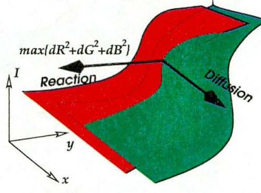
Figure 3: The Red and Green components painted as surfaces in x, y, I with the inverse diffusion (across the edge) and diffusion (along the edge) directions.
