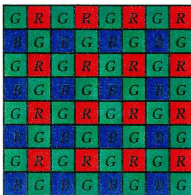
Figure 1: Bayer CFA (color filter array) pattern (US Patent 3,971,065, 1976).
