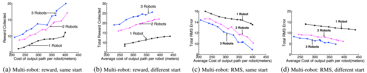
Figure 4: Experiments using multiple robots on the lake dataset.
