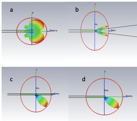
Figure 3: Farfield radiation angular distribution (a): metal horn structure, (b): uncut structure, (c): offset structure, (d): Vlasov cut structure.
