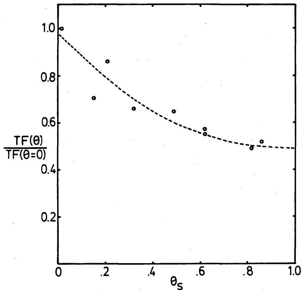
Fig. 5.14 Rate of thiophene HDS vs. initial sulfur coverage of the Mo(100) surface. Rates are given relative to those on the clean surface. P(\text{H}_2) = 780\text{ torr} , P(\text{Th}) = 2.5\text{ torr} , T = 340^\circ\text{C} .
