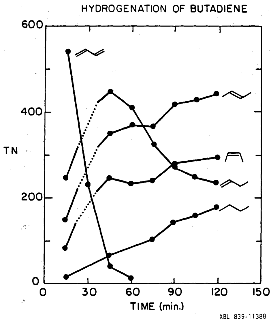
Fig. 5.8 The disappearance of butadiene and appearance of butenes and butane in the reactor during the hydrogenation of butadiene over a sulfided Mo(100) surface.
