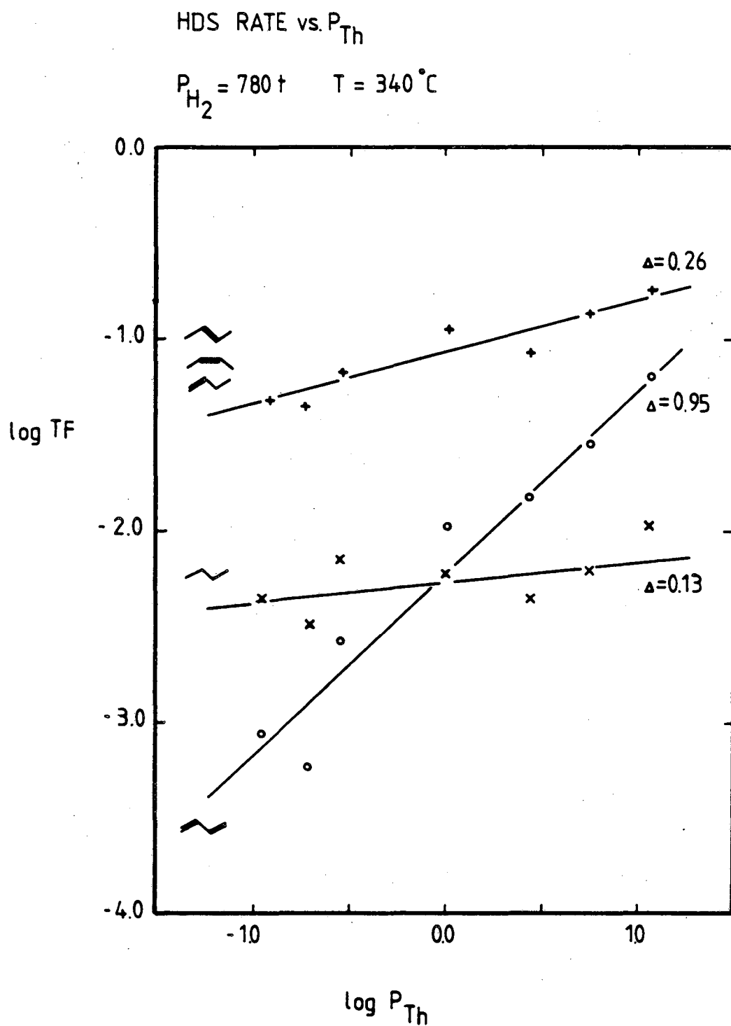
Fig. 5.13 Thiophene pressure dependence of the product rates of appearance during thiophene HDS over the clean Mo(100) surface. P(H_2) = 780 \text{ torr} , T = 340^\circ\text{C} .
