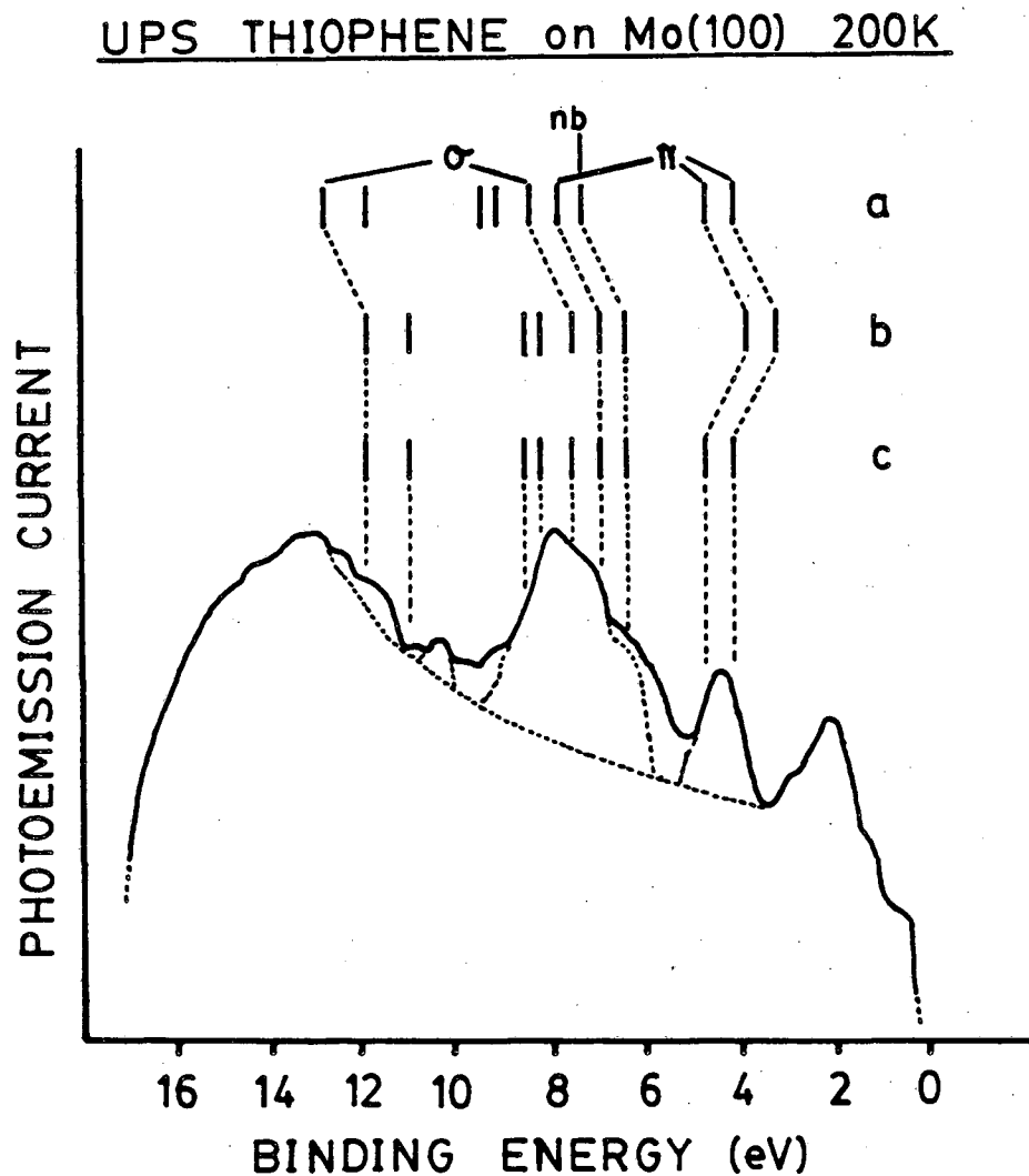
Fig. 4.10 He I UP spectra of chemisorbed thiophene on the Mo(100) surface after heating to 200K. a) Orbital energy levels of the condensed multilayer phase. b) Orbital energy levels shifted to lower binding energy due to increased screening by the metal after desorbing the multilayer. c) Stabilization of the highest lying \pi -orbitals resulting from bonding interactions with the metal.
