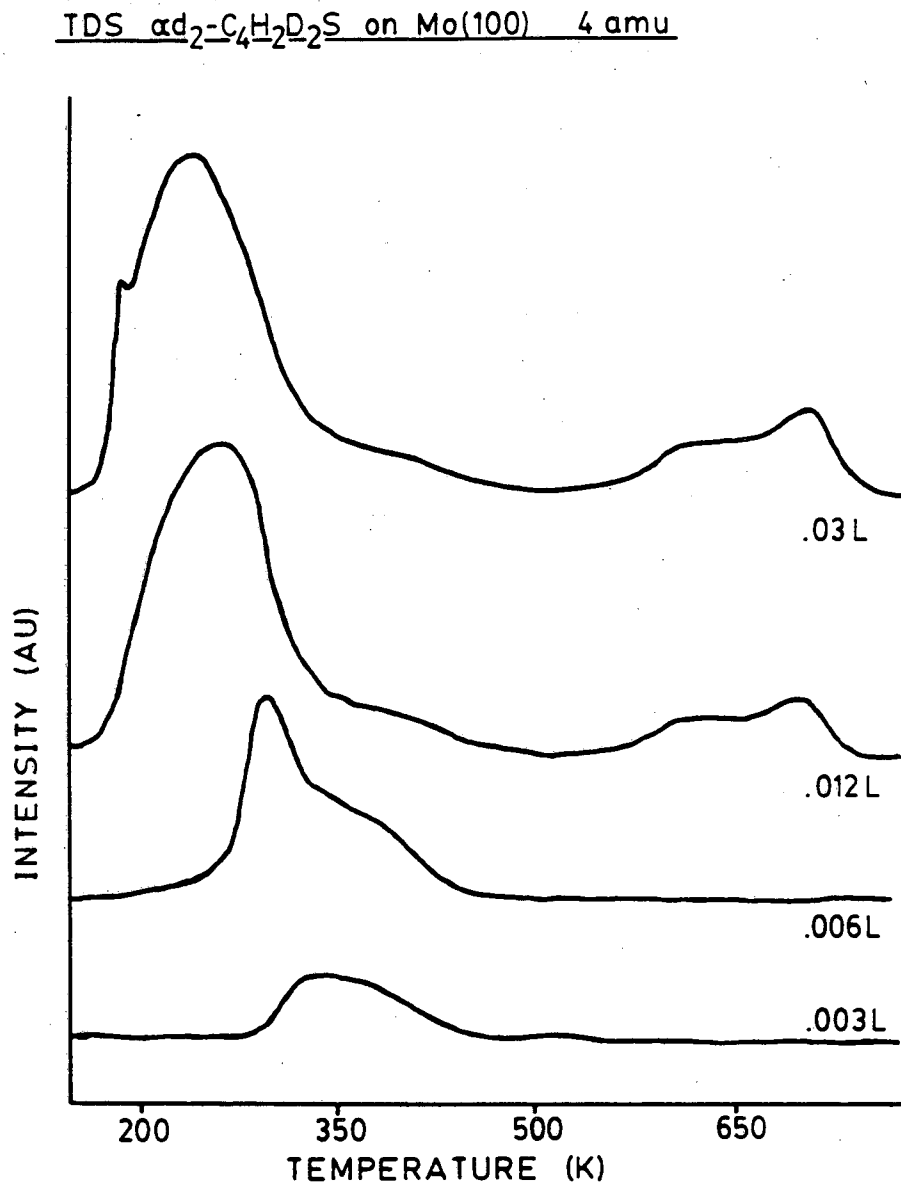
Fig. 4.6 The D 2 desorption spectra resulting from the decomposition of \alpha -C 4 D 2 H 2 S on the clean Mo(100) surface.
