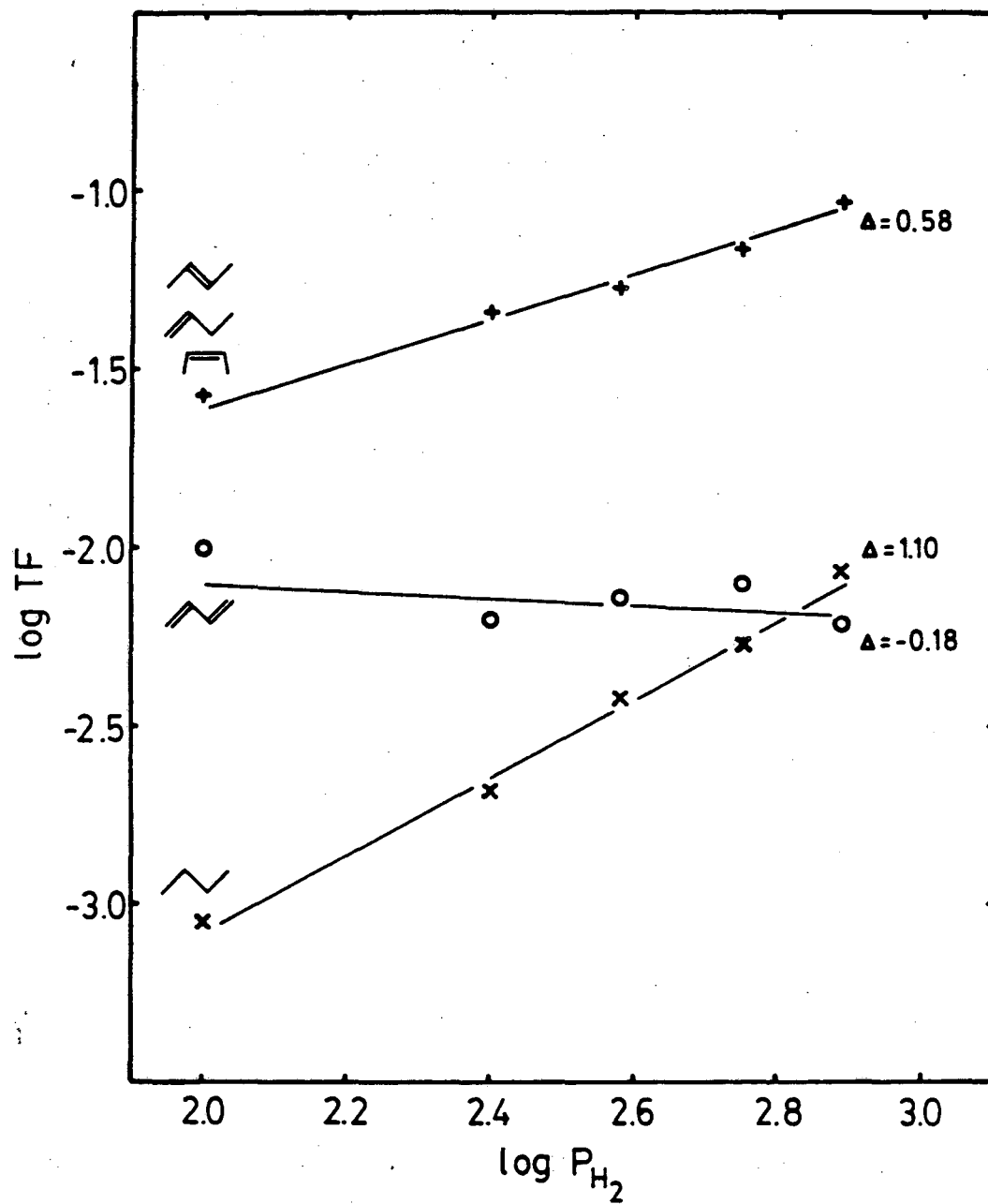
Fig. 5.12 Hydrogen pressure dependence of the product rates of appearance during thiophene HDS over the clean Mo(100) surface. P(\text{Th}) = 2.5 \text{ torr} , T = 340^{\circ}\text{C} .
