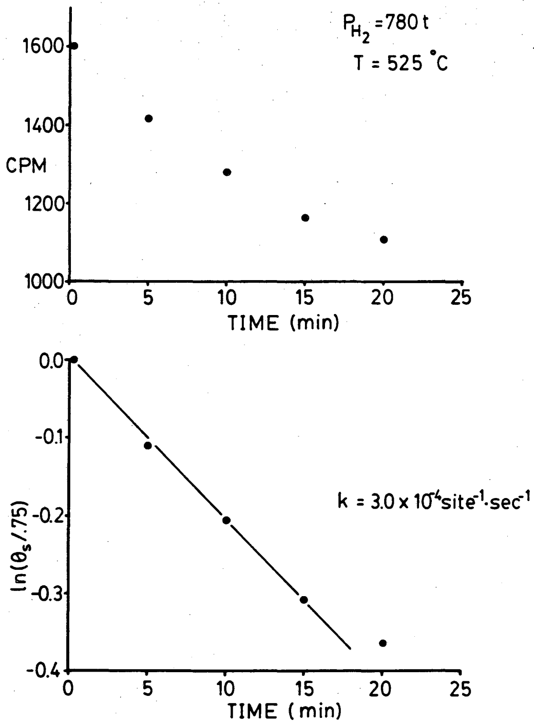
Fig. 6.1 A) Decrease in ^{35}\text{S} signal with time during reduction in \text{H}_2 . Initial coverage was \theta_s = 0.75 , T = 525^\circ \text{C} , P(\text{H}_2) = 780 \text{ torr} . B) Plot of \ln(\theta_s/0.75) vs. t shows first order kinetics.
