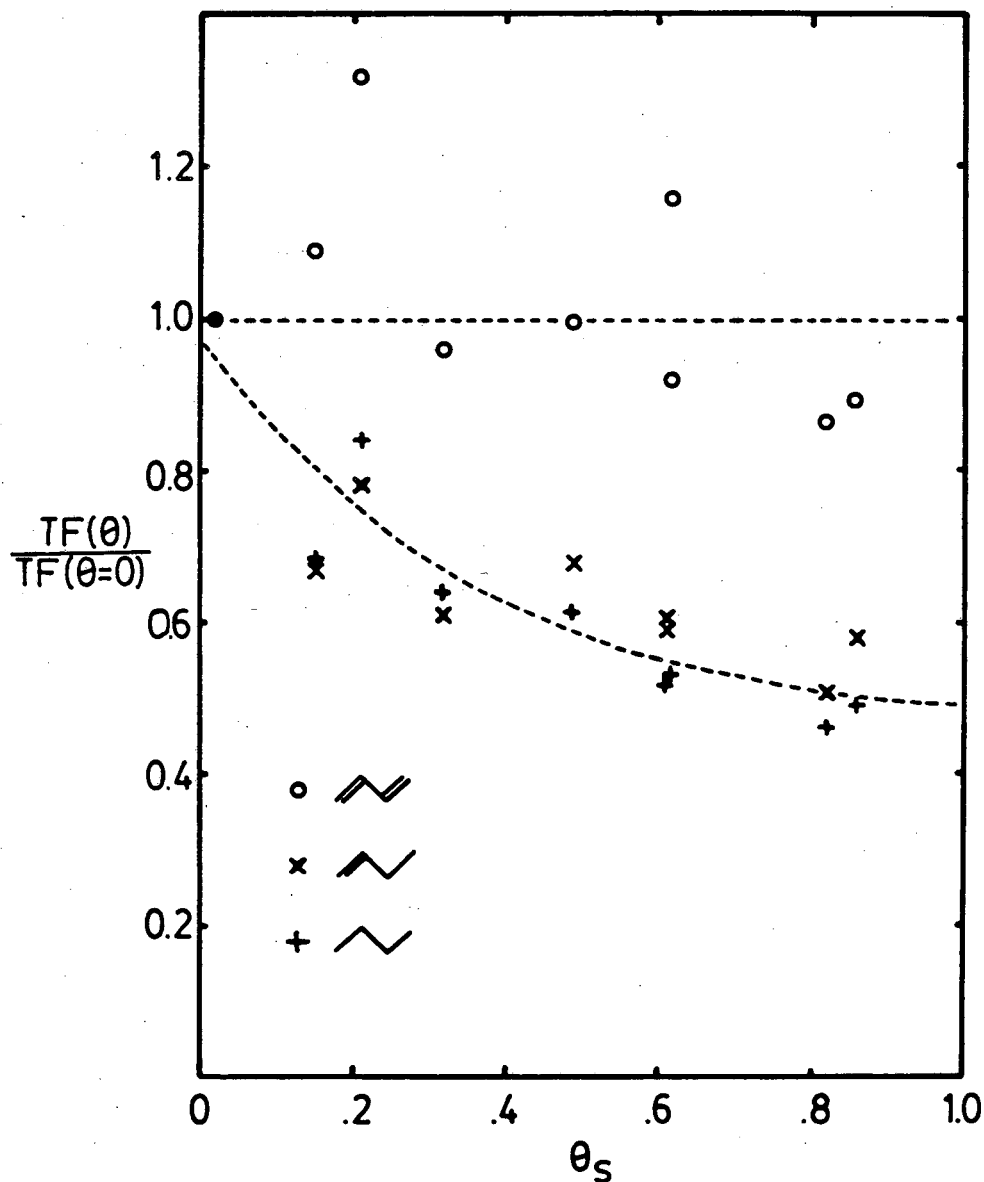
Fig. 5.15 Product rates of appearance vs. initial sulfur coverage of the Mo(100) surface. Rates are given relative to those on the clean surface. P(H_2) = 780 torr, P(Th) = 2.5 torr, T = 340^\circ C .
