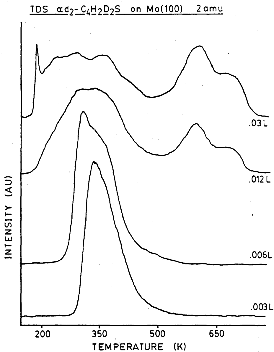
Fig. 4.4 The \text{H}_2 desorption spectra resulting from the decomposition of \alpha - \text{C}_4\text{D}_2\text{H}_2\text{S} on the clean Mo(100) surface.
