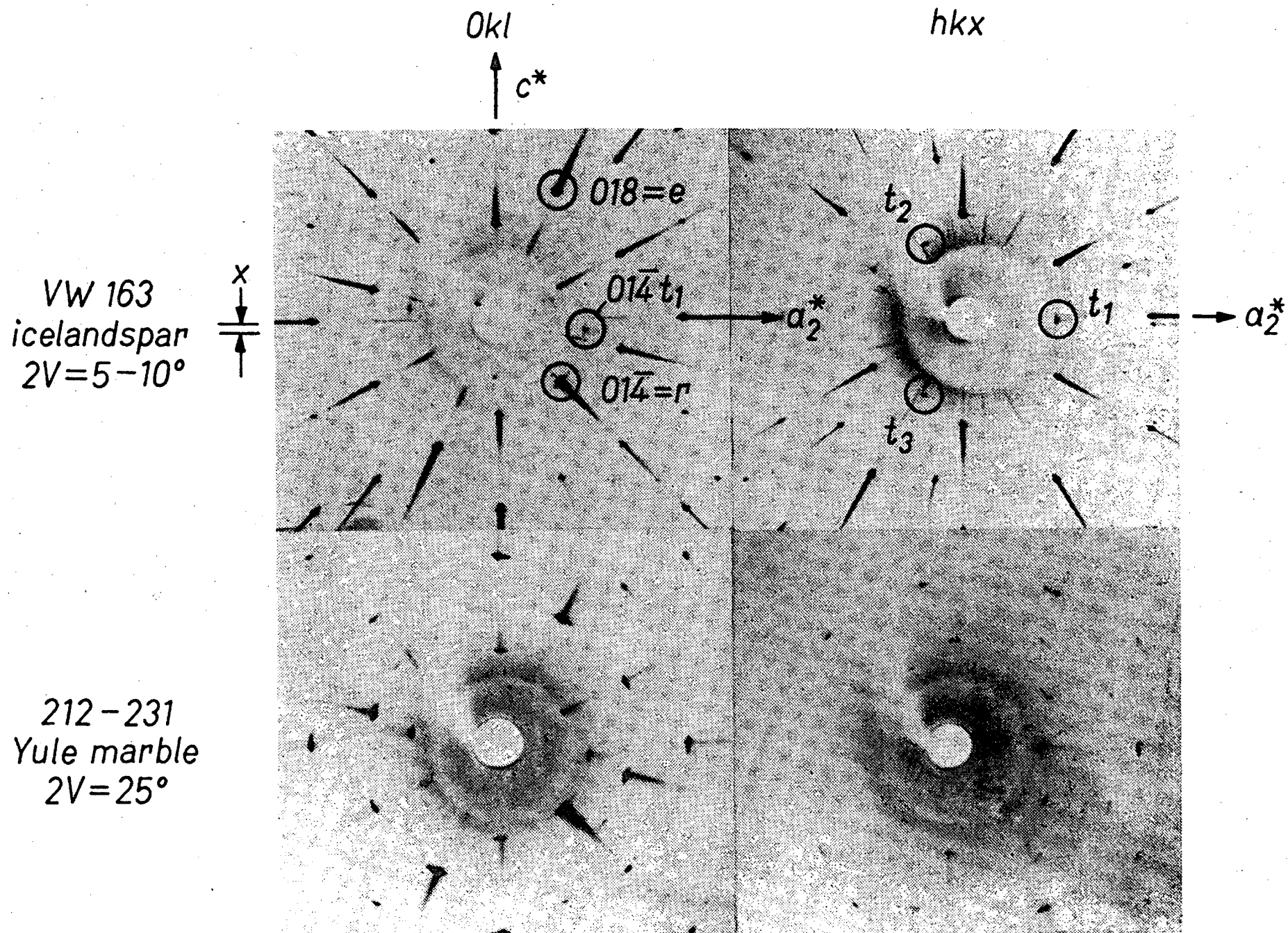
Figure (V.2). Precession photographs showing twinning on \{018\} = e . Mo radiation, Zr filter.
