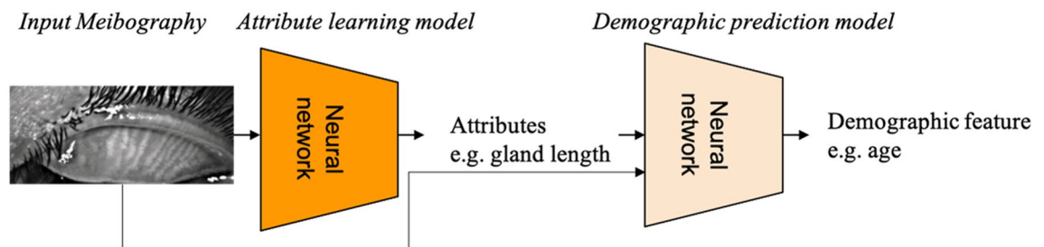
Figure 3. Overall pipeline of the interpretable deep learning model for predicting demographics from images.
