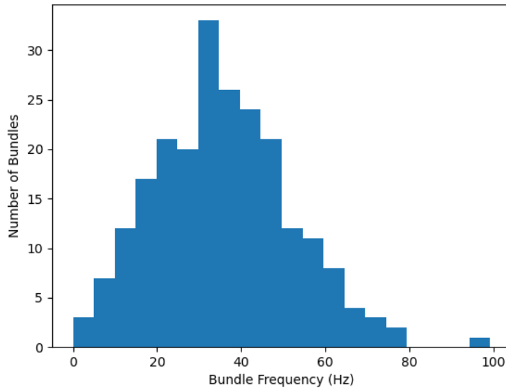
Figure 2: Frequency distribution of 15 x 15 uncoupled hair bundles. The a_0 , S , and f_{\max} values were randomly selected for each hair bundle.
