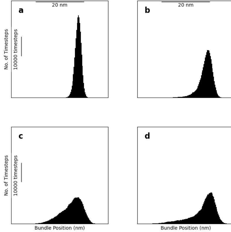
Figure 4: (a-d) Histograms of position of a bundle under damaged conditions for K_d = K, K/5, K/10 , and K/15 , respectively. The traces used to generate these histograms are plotted in black in Fig. 3. Each histogram was produced using a trace from a simulation of 500,000 timesteps representing 10 seconds.
