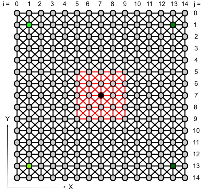
Figure 1: Grid of 15 x 15 coupled hair bundles, each represented by a circle. The black lines represent springs with coupling constant, K , and red lines represent springs with coupling constant, K_d , which are varied to simulate damage to the membrane. Green circles represent the bundles used to compare the dynamics of bundles under normal coupling conditions to those with a damaged membrane. The black circle represents the bundle in the damaged region that will be examined.
