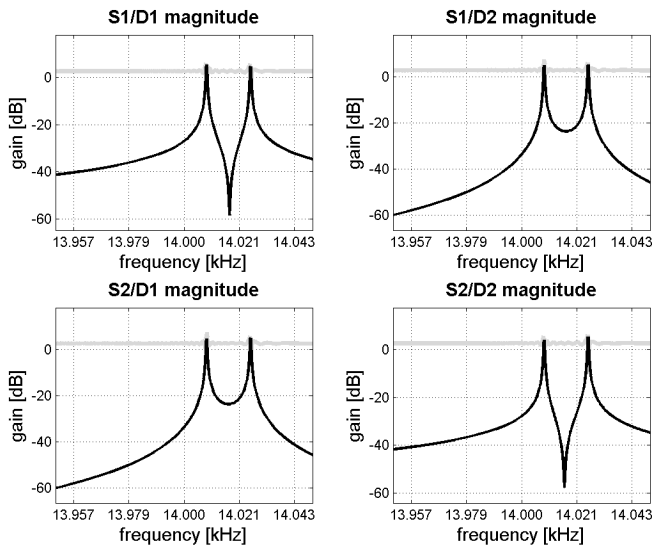
Fig. 2. Frequency response plots associated with the n=2 modes of a URES having excessive parasitic coupling between drivers and pick-offs. The nearly flat gray traces correspond to an FFT-based chirp analysis and offer almost no insight into the modes. The black traces, on the other hand, are based off the parametric model and unambiguously convey the modal characteristics.
