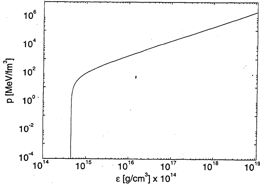
Figure 5: Pressure isotherms versus mass density of electrically charge neutral quark-star matter. The impact of temperatures T \leq 50 MeV, which is significant at low nuclear densities only, is exhibited in Fig. 6.
