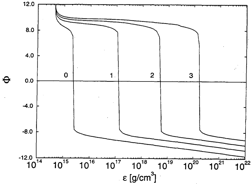
Figure 17: Pulsation frequencies of the lowest four ( n = 0, 1, 2 , and 3 ) normal radial modes of quark matter stars as a function of central star density. For convenience, on the y-axis the quantity \Phi(a) \equiv \text{sign}(a) \log(1 + \text{abs}(a)) with a \equiv (\omega_n/\text{sec}^{-1})^2 is plotted instead of \omega_n^2 itself.
