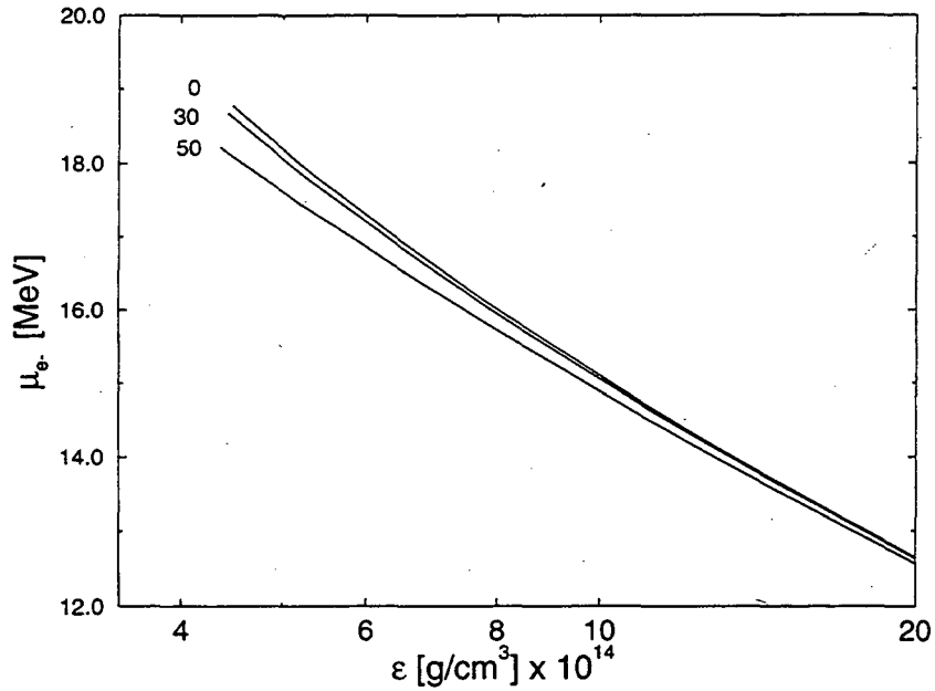
Figure 8: Chemical potential of electrons, \mu_{e-} , versus energy density in electrically charge neutral quark-star matter at temperatures T = 0, 30 , and 50 \text{ MeV} , which are constant along these curves.
