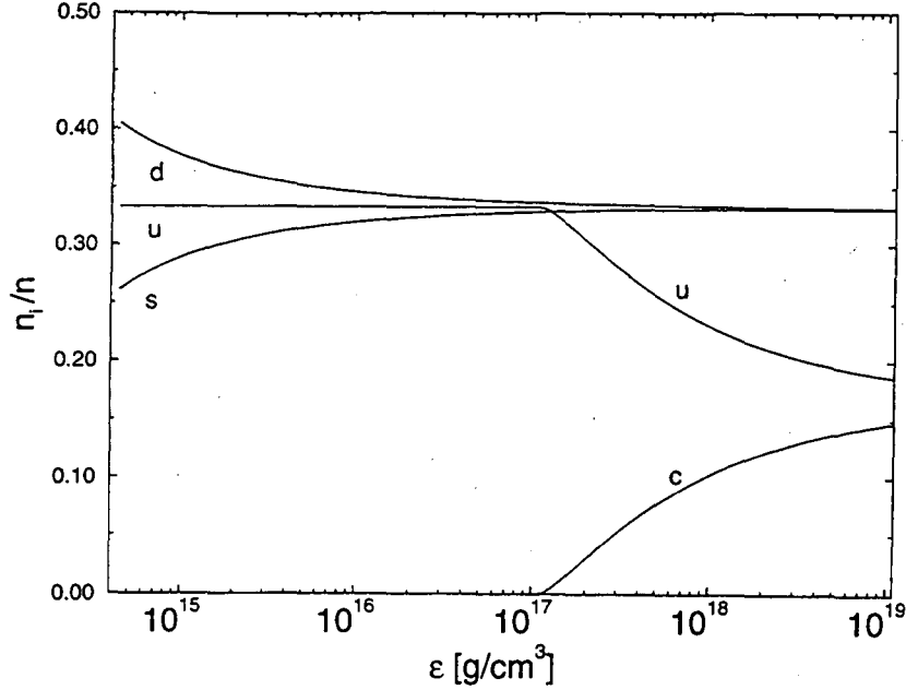
Figure 4: Enlargement of the upper portion of Fig. 3.
