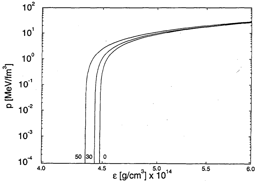
Figure 6: Enlargement of the left portion of Fig. 5. The numbers associated to these pressure isotherms refer to temperature (in MeV). The value of the bag constant (here and for all other calculations) is B = 1 \times 10^{14} \text{ g/cm}^3 (= 57 \text{ MeV/fm}^3) .
