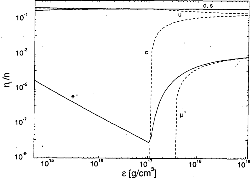
Figure 3: Relative densities of quarks ( q = u, d, c, s ) and leptons ( l = e^-, \mu^- ), n_i/n where n \equiv \sum_{i=q,l} n_i , in cold, beta-stable, electrically charge neutral quark-star matter as a function of energy density. (Here and in all subsequent calculations a bag constant of B^{1/4} = 145 MeV has been chosen.)
