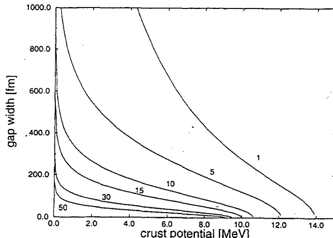
Figure 16: Gap width, R_{\text{gap}} , versus electrostatic crust potential, eV_{\text{crust}} . The labels refer to temperature (in MeV).
