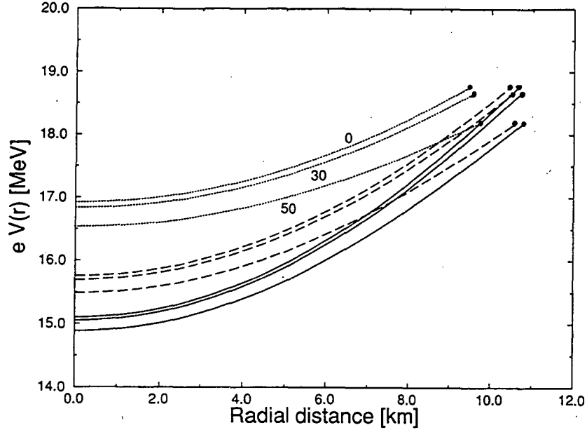
Figure 12: Electrostatic potential, eV(r) , of electrons inside ( r < R ) strange stars of masses M/M_\odot = 1 (dotted curves), 1.4 (dashed), and 1.6 (solid). The temperatures in each case are T = 0, 30 , and 50 MeV. Notice that the termination points of these curves, marked with solid dots, actually lie several hundred fermi inside of R (see Fig. 13).
