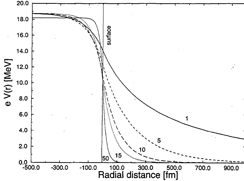
Figure 15: Same as Fig. 13, but for zero external electrostatic potential. The labels refer to temperature (in MeV).
