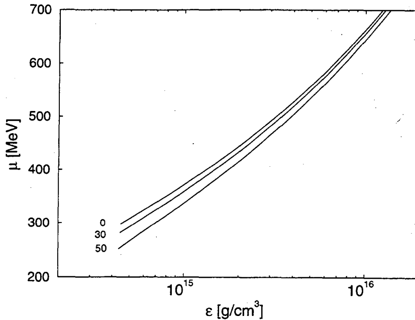
Figure 9: Same as Fig. 8, but for the chemical potential, \mu ( = \mu_d = \mu_s ), of d and s quarks (cf. Eq. (16)).
