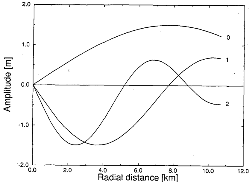
Figure 18: Amplitudes of the three lowest-lying eigenmodes of oscillation ( n = 0, 1, 2 ) of a strange star possessing a representative mass of M \sim 1.5 M_{\odot} . The associated periods of radial oscillation are \tau_0 = 0.334 ms, \tau_1 = 0.117 ms, and \tau_2 = 0.075 ms.
