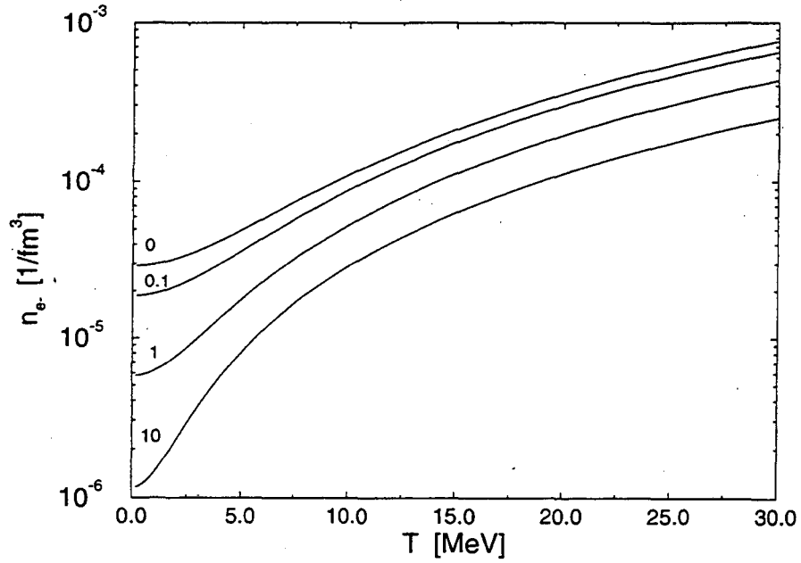
Figure 7: Density isobars of electrons, n_{e-} , versus temperature for different external pressure values, p/(10^{15} \text{ g/cm}^3) = 0, 0.1, 1, 10 , which are constant along each curve. The conversion of pressure from units of \text{g/cm}^3 to \text{MeV/fm}^3 is accomplished by dividing the former by 1.78 \times 10^{12} .
