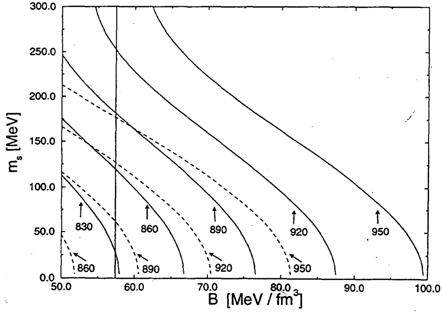
Figure 1: Contours of fixed energy per baryon number (figures attached to these curves) of strange quark matter at zero external pressure. The solid and dashed curves refer to T = 0 and T = 30 MeV, respectively. The strange quark mass is plotted on the y-axis and the bag constant, B , on the x-axis. The conversion of B from \text{MeV}/\text{fm}^3 into units of MeV is accomplished by means of multiplying the former with powers of 1 = 197.3 \text{ MeV fm} .
