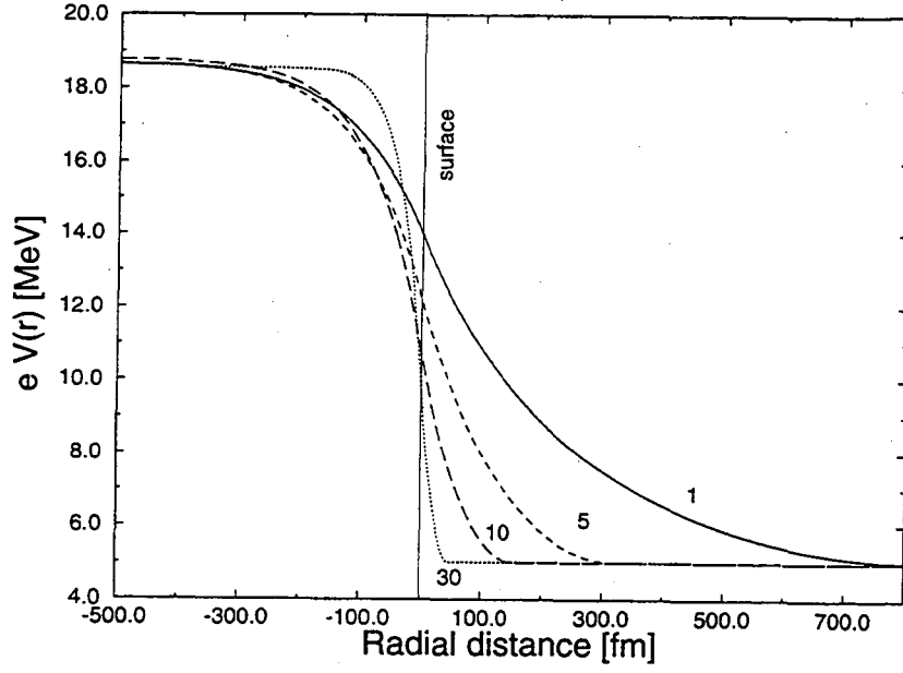
Figure 13: Electrostatic potential of electrons in the close vicinity inside and outside of the surface of a strange star. The location of its surface is indicated by the vertical line. The figures assigned to these curves refer to temperature (in MeV). A representative value for the electrostatic crust potential, eV_{\text{crust}} = 5 MeV (horizontal line), which is constant (see text), has been chosen. The gap width extends from \sim 40 fm to about 800 fm, depending on temperature.
