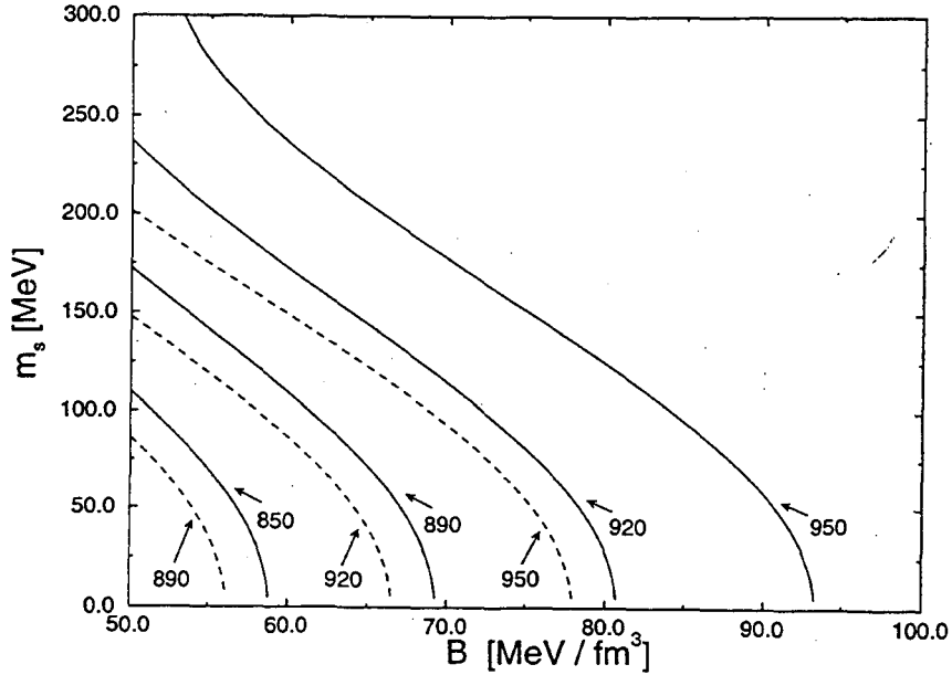
Figure 2: Same as Fig. 1, but for a finite external bag pressure of 50 \text{ MeV}/\text{fm}^3 .
