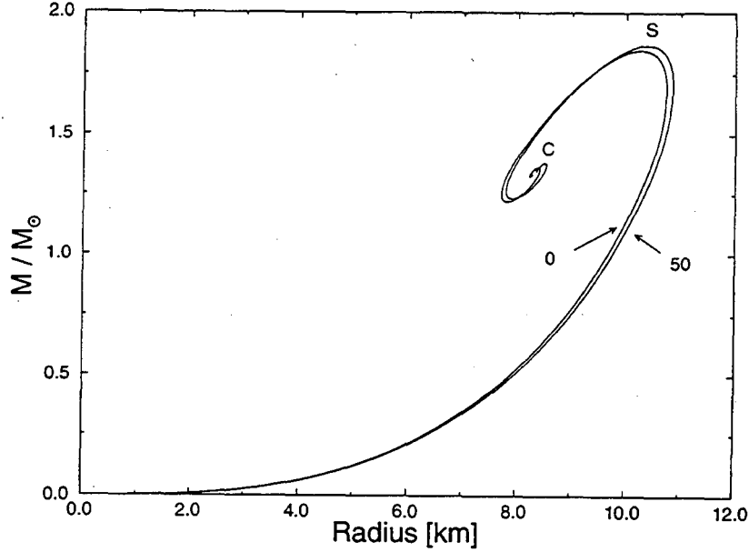
Figure 11: Gravitational mass (in units of solar mass) versus radius of the strange- and charm-quark star sequences exhibited in Fig. 10. The symbols ‘S’ and ‘C’ again denote the maximum-mass model of each sequence.
