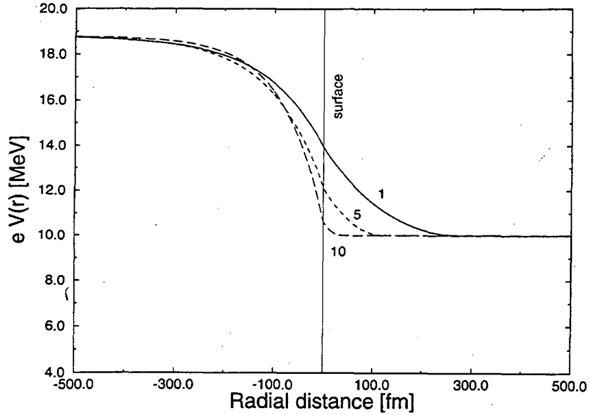
Figure 14: Same as Fig. 13, but for a electrostatic crust potential of 10 MeV.
