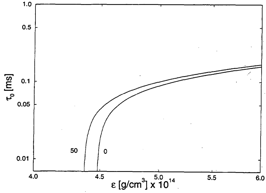
Figure 19: Lowest-lying periods of radial oscillation, \tau_0 , of strange stars versus central star density, for star temperatures T = 0 and 50 MeV.
