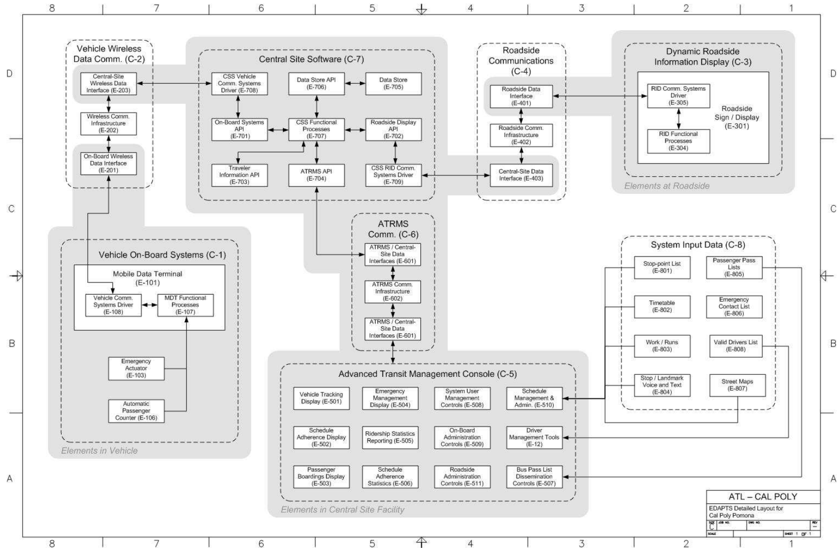
Figure 3 High-Level Design of the Bronco Express EDAPTS System
