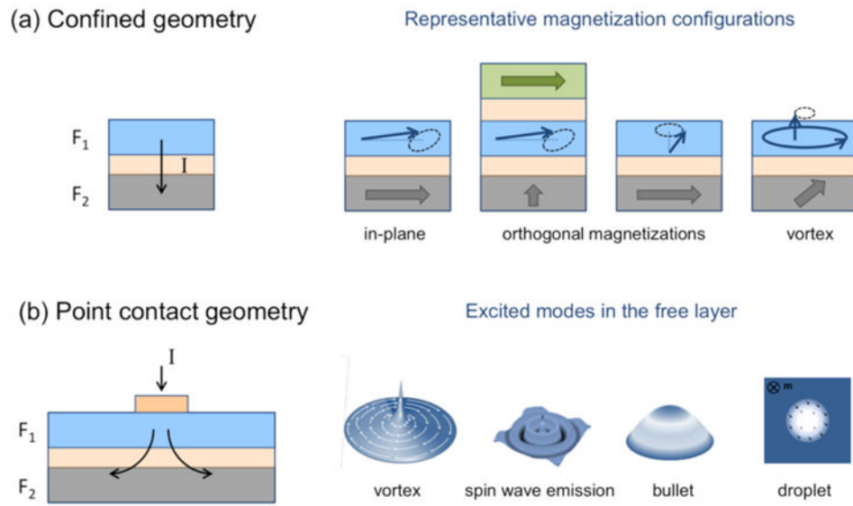
Figure 22. Different types of spin-torque nano-oscillators. Top: confined geometries with a pillar structure. Bottom: geometries in which current from a point contact excites magnetic dynamics in an unpatterned magnetic free layer.
