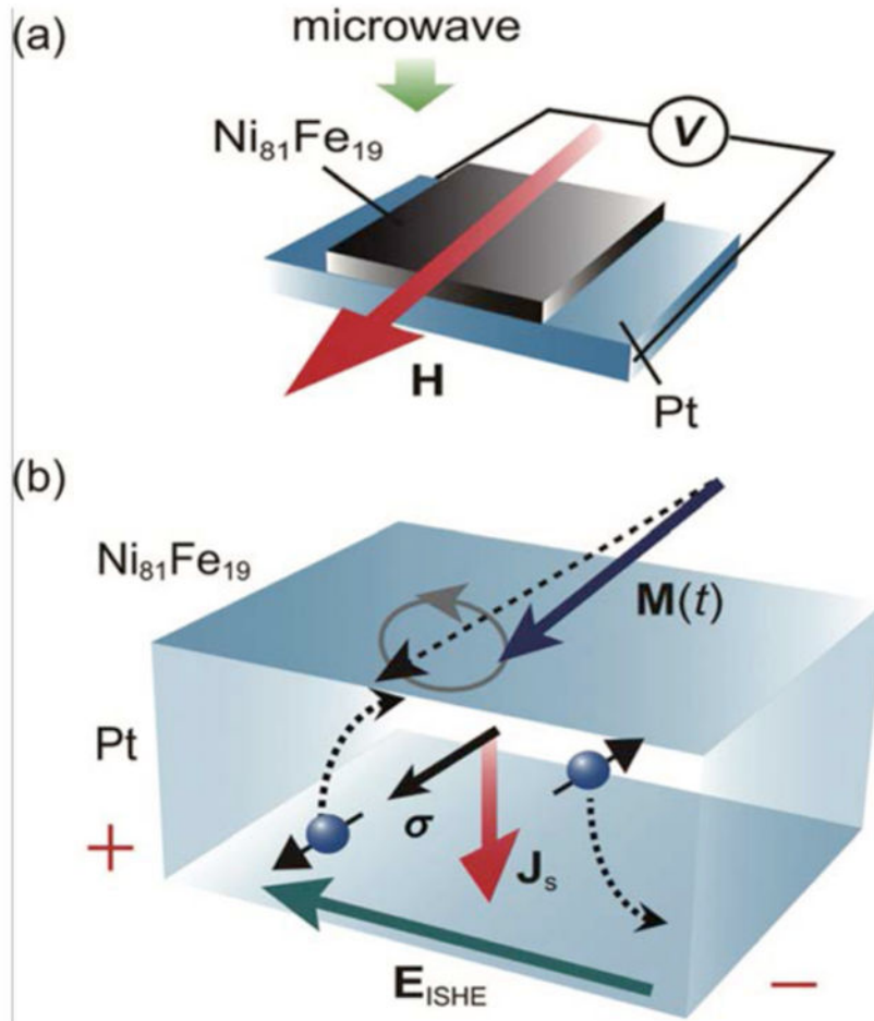
Figure 7. Schematic of spin pumping from a ferromagnet ( \text{Ni}_{81}\text{Fe}_{19} ) film into a nonmagnetic metal (Pt). (a) A microwave field causes precession of magnetization \mathbf{M}(t) around the applied external field \mathbf{H} , pumping spins into the nonmagnet and generating voltage V through the inverse spin Hall effect. (b) The precessing \mathbf{M}(t) pumps spins into the Pt causing spin current \mathbf{J}_s with spins \sigma , in the directions shown, equivalent to a net flow of moments (black arrows on electrons) oppositely directed to \mathbf{M} . The moving electrons are deflected (to the right, for Pt which has the opposite sign of SHE to Ta) by the inverse spin Hall effect which creates an emergent (effective) electric field \mathbf{E}_{\text{ISHE}} in the direction shown. In an open circuit, shown in (a), the resulting induced transient current causes charge to accumulate at the ends of the sample, indicated by the +/- , giving rise to a real electric field (equal and opposite to \mathbf{E}_{\text{ISHE}} ) and the measured voltage V . From [Ando et al. , 2011]
