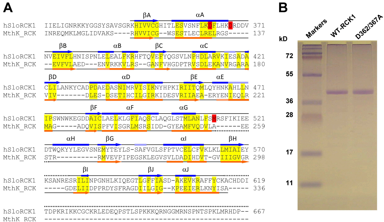
Figure 1. Purification of the RCK1 domain of the human BK Ca channel. (A) Structure-based sequence alignment of the BK Ca channel (GI, 507922) C terminus (encompassing the RCK1 domain) with the MthK (GI, 2622639) RCK domain. The \alpha helices are depicted as bars, and \beta strands are shown as arrows. The secondary structures (obtained from the DSSP reference set) above the sequences (blue) are obtained from the atomic structure of the BK Ca C-terminal domain (Protein Data Bank accession no. 3MT5) (Yuan et al., 2010) and below the sequences (orange) are obtained from the atomic structure of the MthK RCK domain (Protein Data Bank accession no. 2AEF) (Dong et al., 2005). Light blue and light orange bars correspond to _3 helices. Dotted lines are unresolved regions in the respective crystal structures. Semi-conserved residues within ordered structures are highlighted yellow. Residues known to be involved in high-affinity Ca^{2+} sensitivity in the BK Ca RCK1 domain (D362/D367 and M513) are highlighted red. (B) 12.5% SDS-PAGE of purified WT-RCK1 and D362/367A-RCK1 stained with Coomassie blue. Both proteins migrate as an \sim 40-kD band, consistent with their expected mol wt (41 kD).
