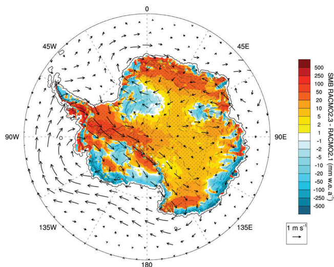
Fig. 4. Average (1979–2011) SMB difference (RACMO2.3 – RACMO2.1). Vectors show direction and magnitude of average 500 hPa wind speed difference (RACMO2.3 – RACMO2.1) ( \text{m s}^{-1} ). Areas where the difference exceeds one unit of standard deviation of the difference are stippled.
