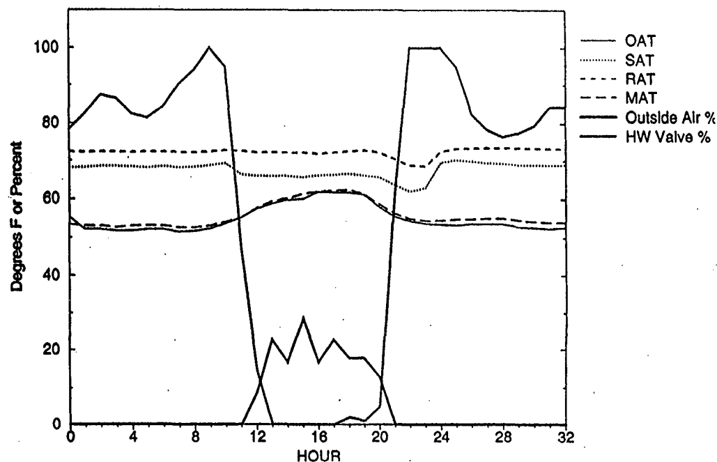
Figure VI-19. EMCS Operational Data: Economizer Control (cont.). One day of data, including the position of the heating control valve. At times when the economizer called for minimum outdoor air, the heating was almost fully on. This suggests that the building received significant outside air even when the economizer control called for minimum outside air. After reviewing this with the shared savings project manager, and reviewing the building's mechanical plans, it was discovered that the building is actually designed to operate with a large amount of outside air, because a large fraction of the floorspace is laboratories with their own exhaust system. The outdoor air intake and supply fan are sized for 100,000 cfm, while the return fan and recirculating dampers are sized for only 20,000 cfm. When the EMCS indicates "100% return," this actually means that the building is operating with 80% outside air. This illustrates the usefulness of having one day of hourly data collected automatically for all points, but also illustrates the difficulty in evaluating measured data, and the need to truly understand the particular building.
