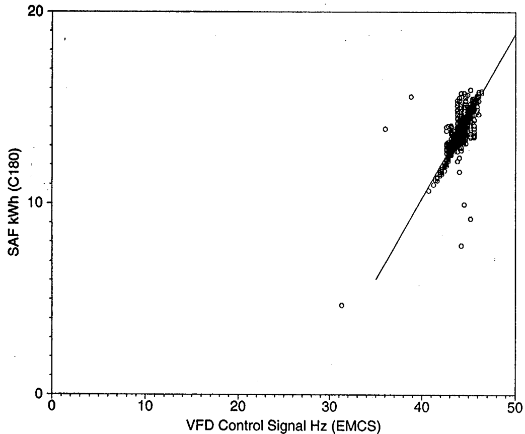
Figure VI-28. EMCS Proxy Measurement: Fan Speed Regression. As suggested in the previous graph, a simple scaling factor may not produce as good a proxy measure as a regression of fan kWh versus Hz, which is shown here. The best-fit line had a constant of -23.8 kWh, and a coefficient of 0.852 kWh/Hz. The R-squared of the fit was 0.76. A period of over 3000 hours of data collected by the dedicated monitoring were used to perform this regression. When only the first week of data were used, however, the best fit line was considerably different. When fewer data are used, therefore, one must make sure that a wide enough range of operation is included in the calculation.
