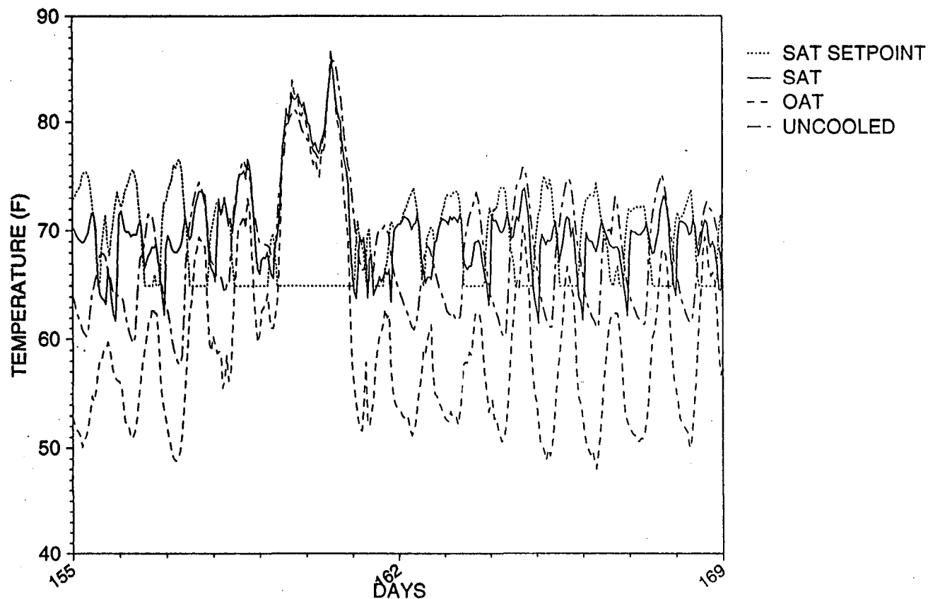
Figure VI-16. EMCS Operational Data: Supply Temperature Control. According to the Sequence of Operations, the supply air should be heated to maintain the coldest space temperature in an uncooled zone at or above 70°F during the day, and 68°F at night. The supply air is never cooled. The supply air temperature setpoint was a constant 65°F during the day, except for the very coldest days, when it rose during the day. At nights, the temperature setpoint rose to about 75°F. The actual supply air temperature was always between about 60°F and 70°F, except on the two very warm days, when it is expected to rise (since it is not cooled). The zone temperature (this is only one of the uncooled zones—not necessarily the coldest) was below 70°F on weekends, and sometimes went well below 68°F during weekdays as well.
