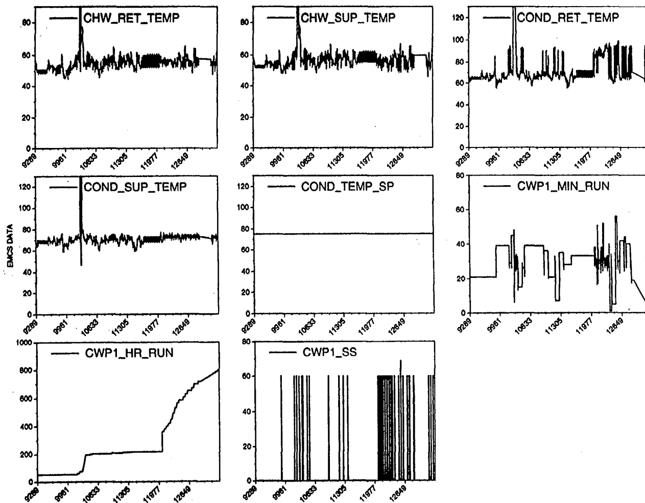
Figure VI-8. Data collected from EMCS in Case Study Building (cont.). The EMCS collected many different types of data, including both energy consumption and operational data.
