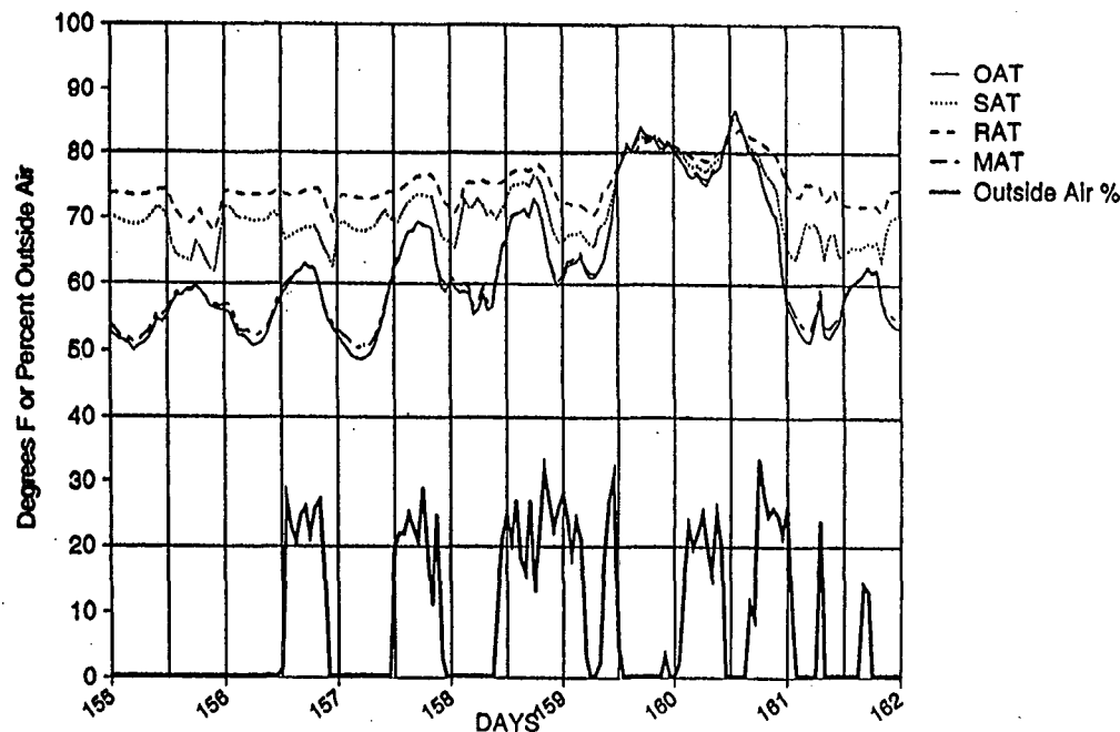
Figure VI-17. EMCS Operational Data: Economizer Control. Since there is no cooling, when there is no heating the mixed-air temperature (MAT) setpoint should track the supply-air temperature (SAT) setpoint. The economizer should be at the minimum outside air setting when the building is being heated, and when the outside air is warm enough, it should modulate open to maintain the mixed air temperature at the supply air temperature setpoint. When the outdoor-air temperature (OAT) is greater than the return air temperature (RAT), the outside air dampers should close, and again bring in minimum outside air. Since the supply air is not cooled, the outdoor air temperature will essentially never be above the supply temperature, and this is clearly seen for the two warm days, when the outdoor, mixed, supply and return air streams are all at about the same temperature. As expected, whenever the outdoor air is warm—above about 60°F—the fraction of outside air climbs. When the outdoor air is too hot—above about 80°F—the fraction again drops to the minimum, as expected. However, it is surprising that the mixed air and outdoor air temperatures are always so similar. This is not what one would expect for economizer operation, and may suggest operational problems.
