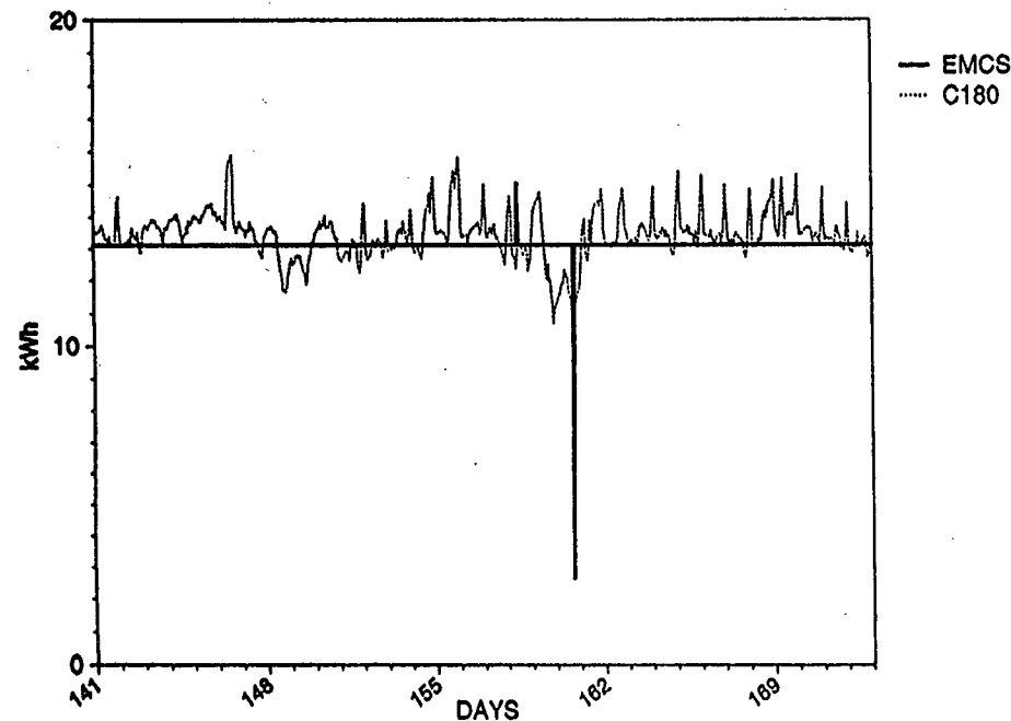
Figure VI-25. EMCS Proxy Measurement: Supply Air Handling Unit. A proxy calculation, similar to that shown in Figure VI-24, is here shown for the supply air fan. A scaling factor of 113.1 kWh was used. Although the fan has a variable-speed drive, it is used in a constant-volume distribution system, so the flow does not vary much. The proxy does represent the overall level of the consumption, but it misses the smaller variations in the consumption. Since the status variables are control outputs, they may be less reliable indicators of operation than actual measurements of operation. It is possible, for example, for the system to "think" it is turning the fan on and off, while in reality the relay is broken or the point is overridden. Can this type of point serve as a proxy for operation? This EMCS is equipped with "proof switches" for all major pieces of equipment, which should be more reliable indicators of whether or not a piece of equipment is on. Proof switches are often used with EMCSs to make absolutely sure that one piece of equipment is operating before another is turned on, for example making sure that a fan is running before opening a cooling valve, to prevent freezing of coils. In this example, the proof can either be current switches that make sure the fan is drawing current, or a flow sensor to ensure that there is actually flow. This EMCS used current switches as proof of fan operation. When status and proof points were compared for the return fan, the correlation was perfect. For the supply fan, however, there were two hours during which the system considered the supply fan to be operating, while the proof switch indicated that it was not operating. Where they exist, proof switches are more reliable for use in a proxy measurement.
