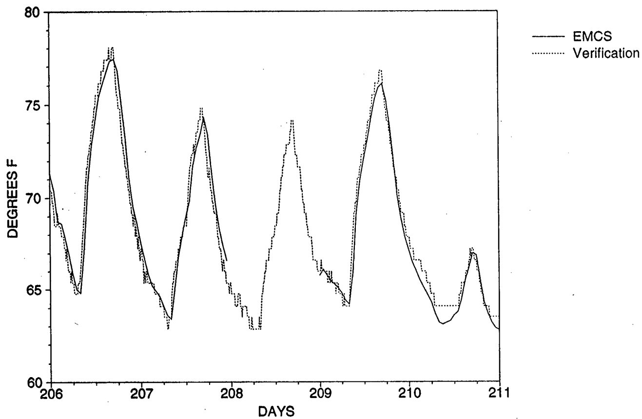
Figure VI-33. Verification of EMCS Temperature Data in an Uncooled Zone. The temperature as measured by the EMCS was quite close to that measured by a HOBO-XT microdata logger.
