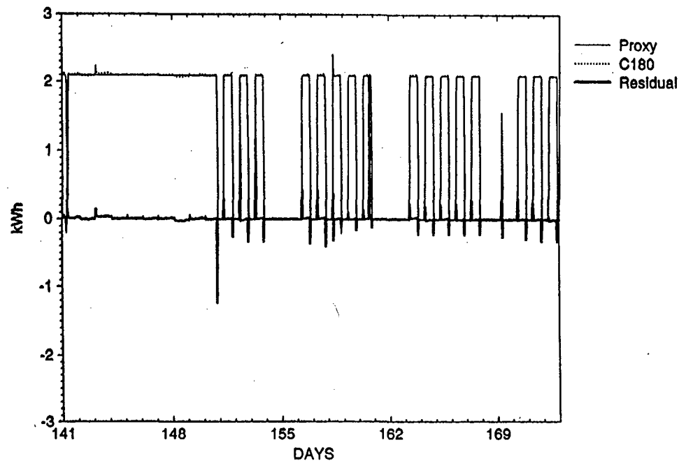
Figure VI-24. EMCS Proxy Measurement: Chilled Water Pump. If power consumption data are not available, it is sometimes sufficient to monitor a proxy for the consumption. Here, chilled water pump status is being used as a proxy for pump energy consumption. (Note that the pump status is an output signal, not an input signal). It is possible to use status as a proxy because the pumps are assumed to be a constant load. The first day of the dedicated monitoring was used to provide a scaling factor. Data collected while the pumps were running were used to calculate this scaling factor, which was 2.09 kWh for each hour of operation. After calculating this scaling factor from the dedicated monitored data for a short period of time, it was applied to the rest of the status data. Here, the consumption measured by the dedicated monitoring is marked "C180" and is indicated by a dotted line. The calculated proxy for the consumption is a thin, solid line. The error (or residual) resulting from using this proxy is indicated with the thicker line. This proxy was a very good indicator of energy consumption, except during the "shoulder" hours, during which the equipment turned on or off.
