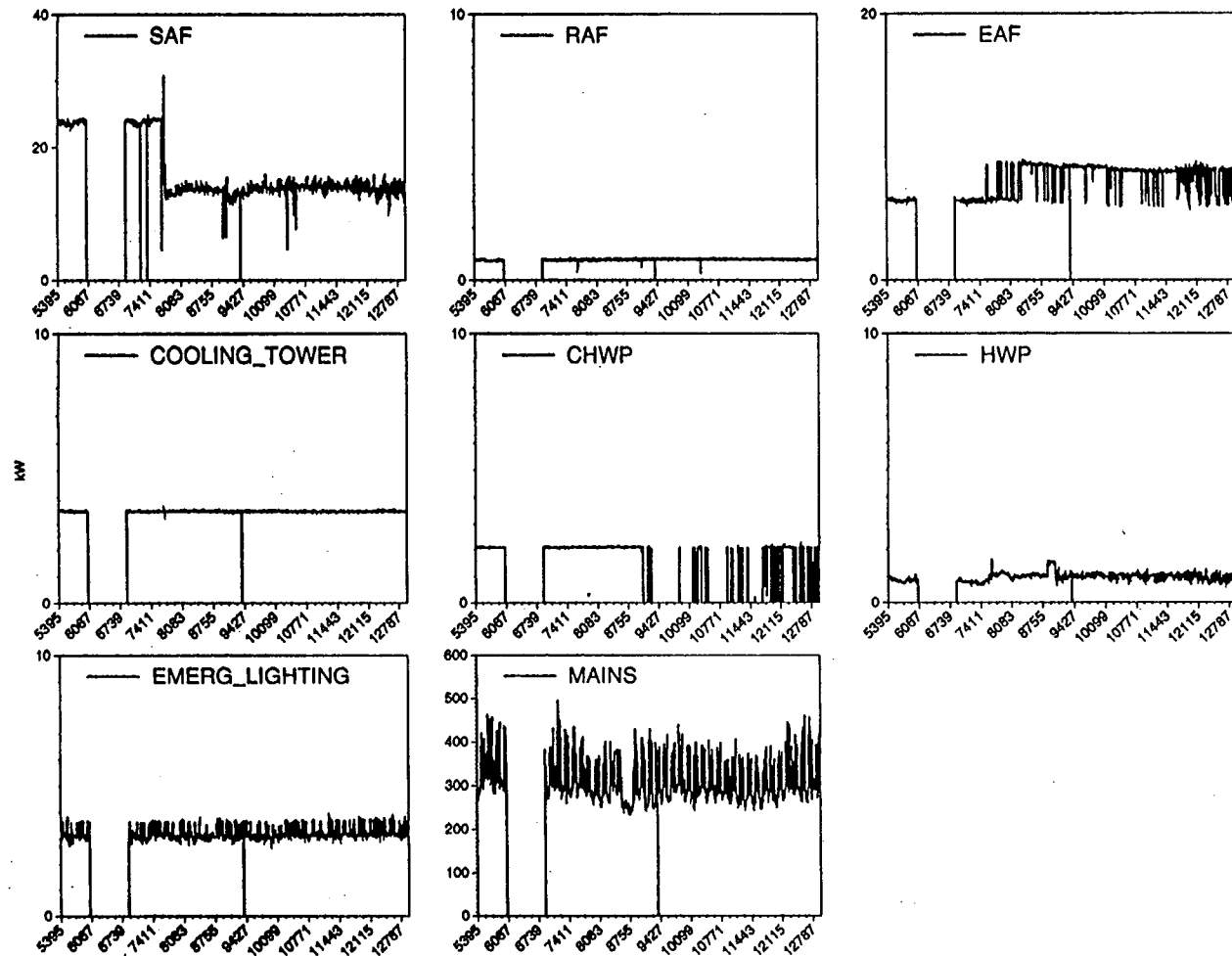
Figure VI-11. Data collected from Dedicated Monitoring in Case Study Building (cont.). The conventional monitoring was installed in parallel to the EMCS, to confirm EMCS data. 16 end-use energy channels were monitored.
