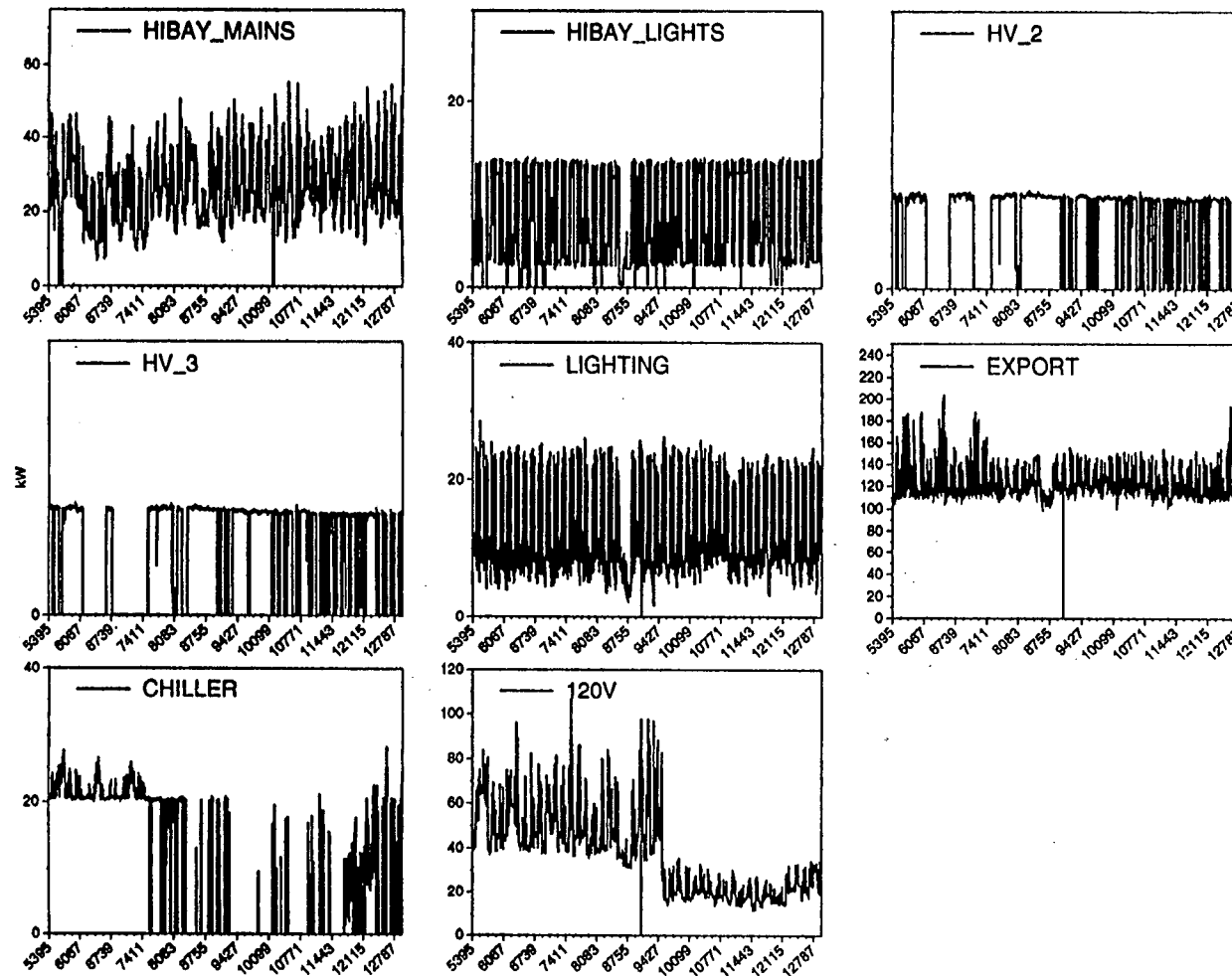
Figure VI-10. Data collected from Dedicated Monitoring in Case Study Building. The conventional monitoring was installed in parallel to the EMCS, to confirm EMCS data. 16 end-use energy channels were monitored.
