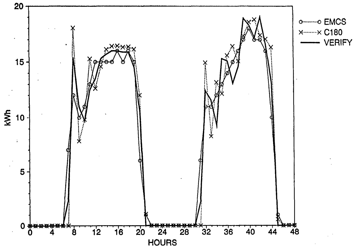
Figure VI-31. Verification of EMCS and Dedicated Monitoring for Chiller. A short-term datalogger was used to verify the data from the EMCS and the C180 dedicated monitoring. On the first day, the verification logger was a Dranetz Analyzer collecting 15-minute data. Thereafter, it was an Esterline Angus Load Surveyor collecting one hour data. The EMCS was not collecting reliable data.
