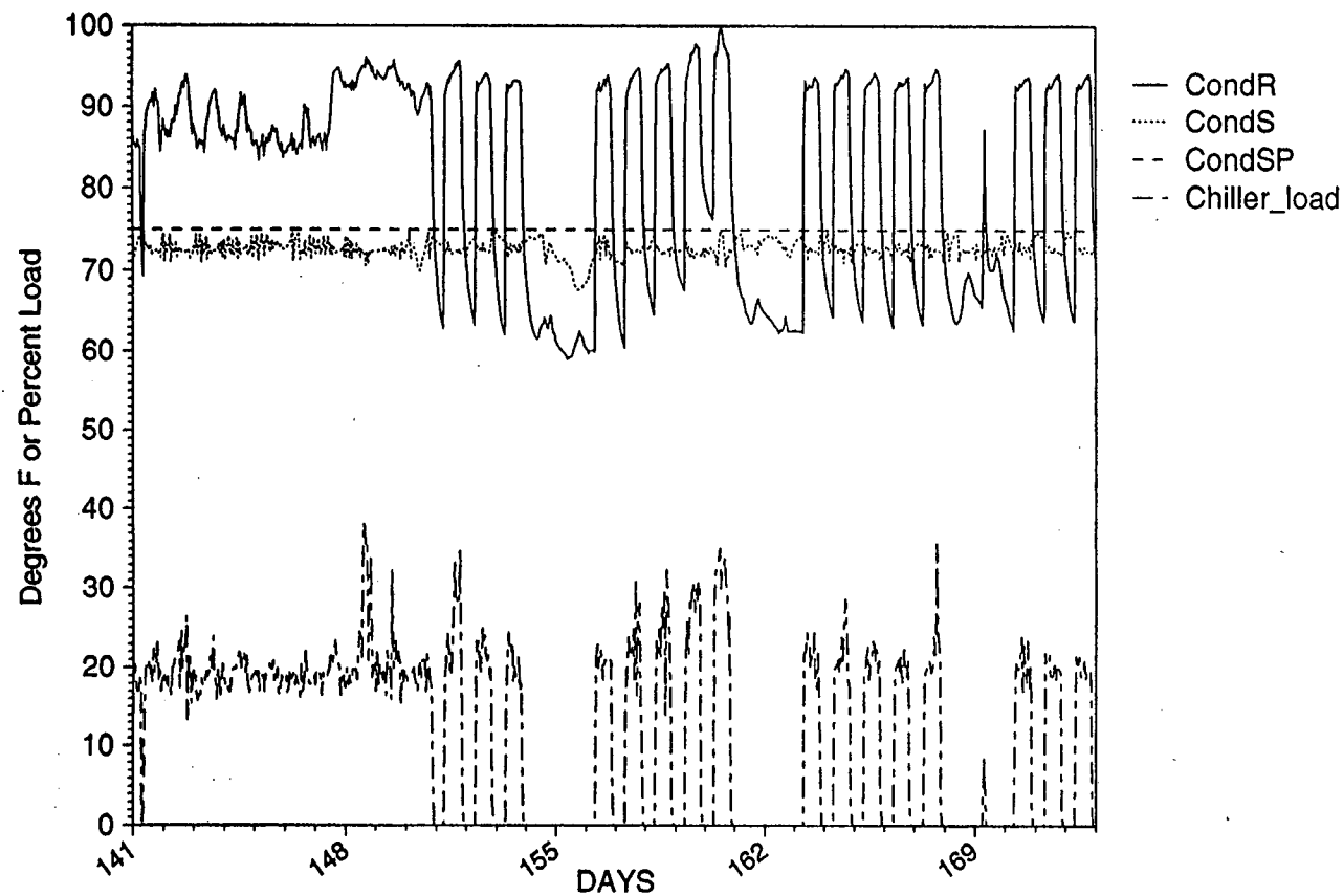
Figure VI-23. EMCS Operational Data: Cooling Tower Control. According to the Sequence of Operations, the cooling tower fan should maintain the condenser water supply temperature at 75°F. The condenser supply temperature appeared to be very well controlled, but it was always offset several degrees below the setpoint. In this figure, one week can be seen where the cooling system was overridden and left on for an entire week.
