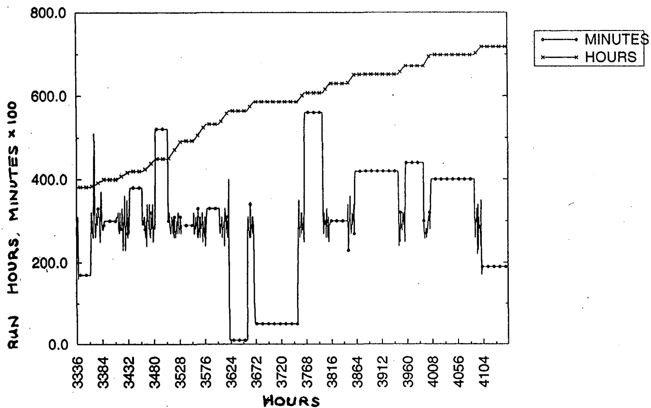
Figure VI-38. EMCS Cumulative Data for Chilled Water Pump Runtime. Runtime is also a cumulative point. The minute point was incremented by one whenever the pump had operated for a minute. The hour point was incremented by one whenever the minute point hit 60. Since both values are averaged over an hour for reporting, the minute data are very difficult to interpret.
