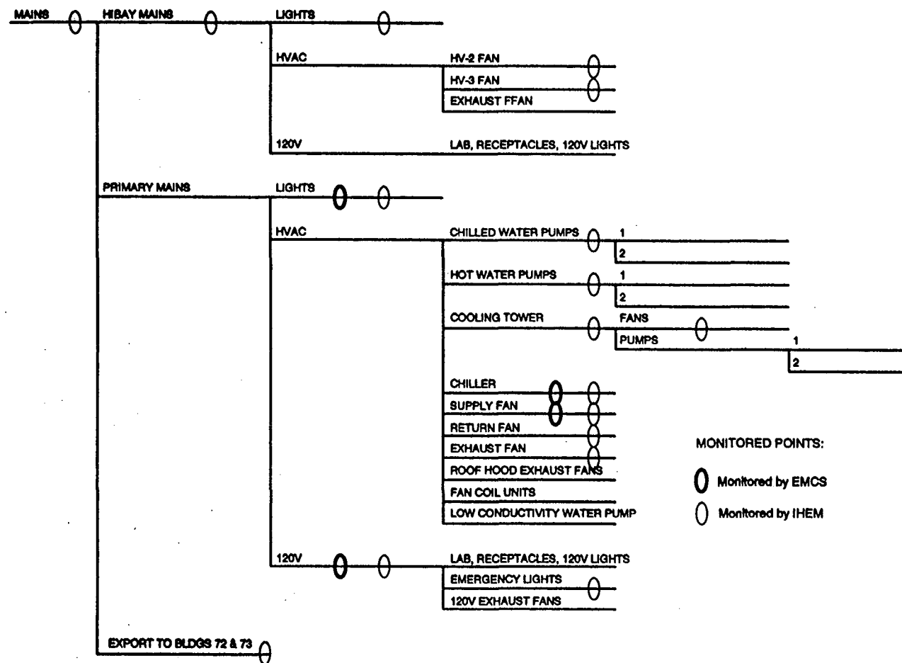
Figure VI-30. Measurement Points for EMCS and Dedicated Monitoring. The EMCS measured many of the same points as the dedicated monitoring, so a good comparison of the two methods was possible.
