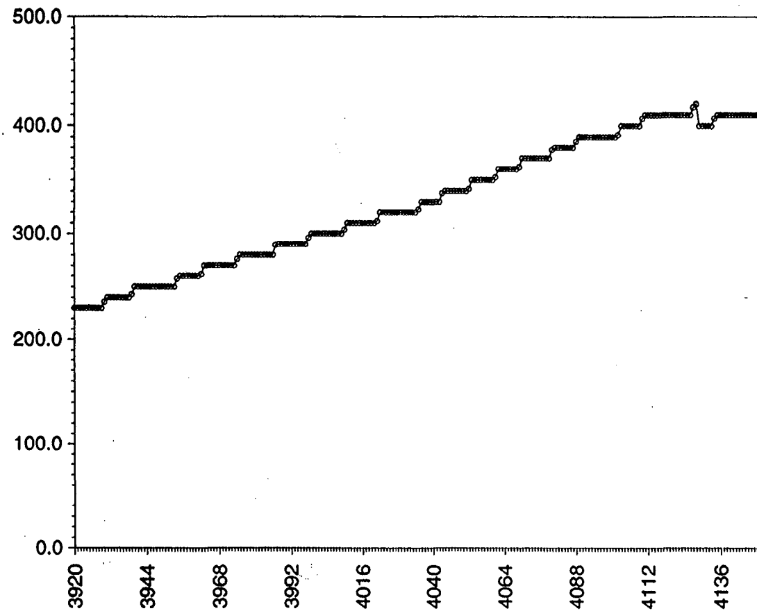
Figure VI-36. EMCS Cumulative Data for the Chiller KWH Point. The kWh points were averages of a cumulative value over an hour. The cumulative value was incremented by ten whenever ten kWh had been consumed. Whenever the kWh point reached 1000, it was reset, but this seldom occurred because the transducer was not operating correctly.
