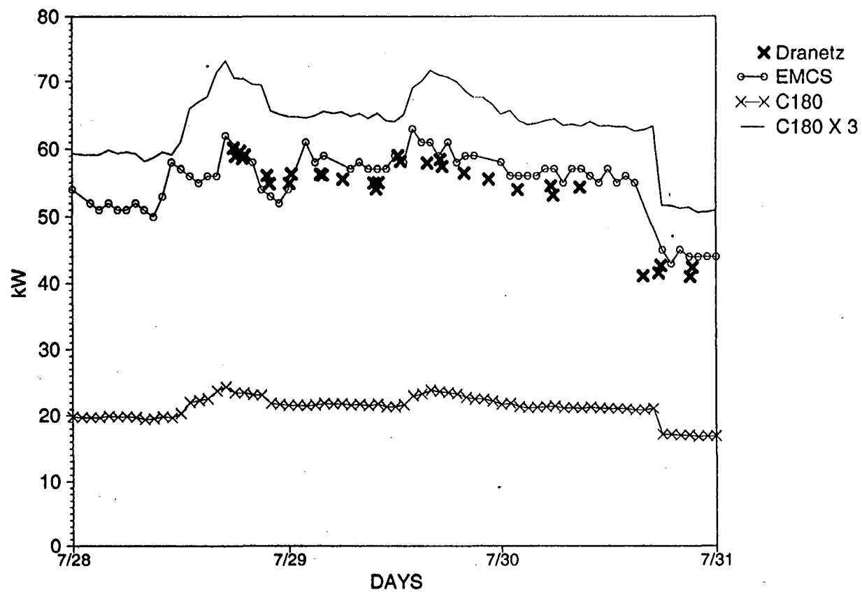
Figure VI-32. Verification of EMCS and Dedicated Monitoring for Miscellaneous. A Dranetz short-term datalogger was used to verify the data from the EMCS and the dedicated monitoring. The EMCS provided more reliable data than the C180 dedicated monitoring, because two CTs had been removed from the dedicated equipment. When scaled up by a factor of three, the C180 still was not correct.
