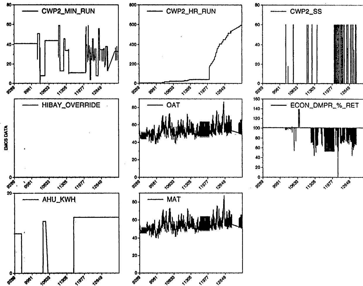
Figure VI-7. Data collected from EMCS in Case Study Building (cont.). The EMCS collected many different types of data, including both energy consumption and operational data.
