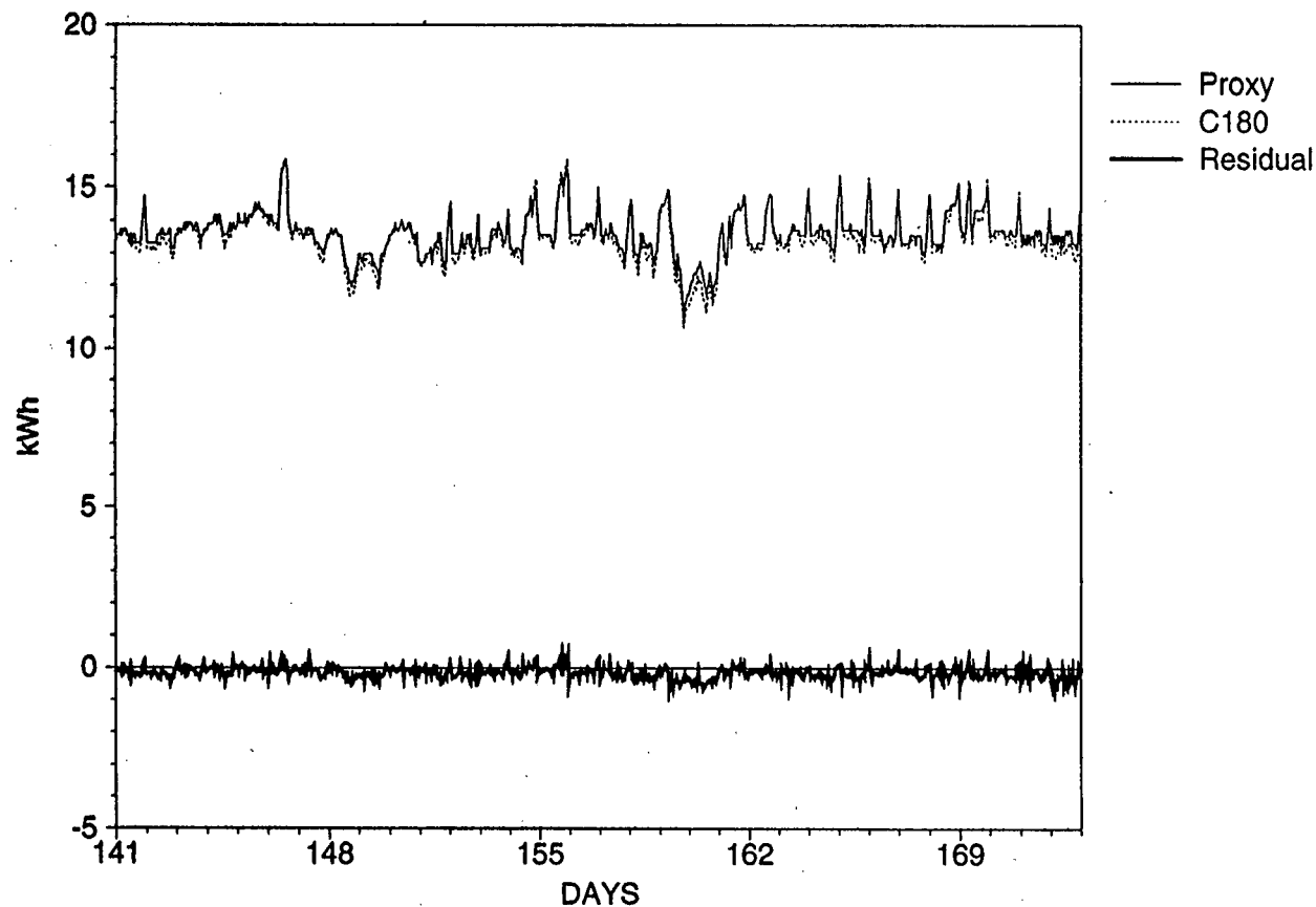
Figure VI-29. EMCS Proxy Measurement: Fan Speed Regression (cont.). The result of the proxy calculation with the regression based on the full data set, as shown in the previous figure. If the fan were operated over a wider range of speeds, one would probably want to perform a polynomial fit to the data, since fan power should vary with the cube of the flow (nominally). There is very good correspondence between the proxy and the measured quantities, although this must be traded off with the need for a large amount of data to perform the regression.
