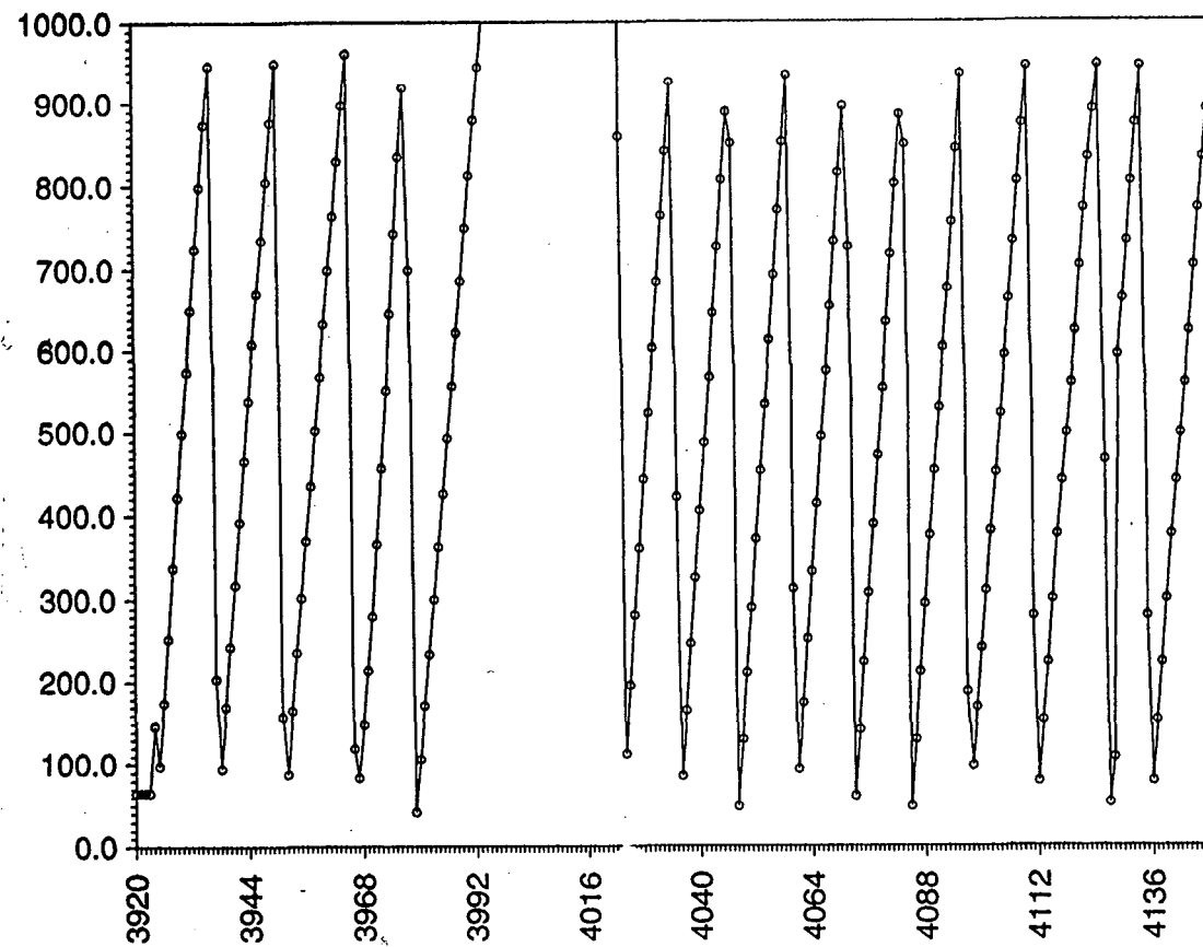
Figure VI-35. EMCS Cumulative Data for the Miscellaneous KWH Point. The kWh points were averages of a cumulative value over an hour. The cumulative value was incremented whenever one kWh has been consumed. Whenever the kWh point reached 1000, it was reset. This occurred one to two times a day. It was difficult to interpret the data during the hour that the counter is reset.
