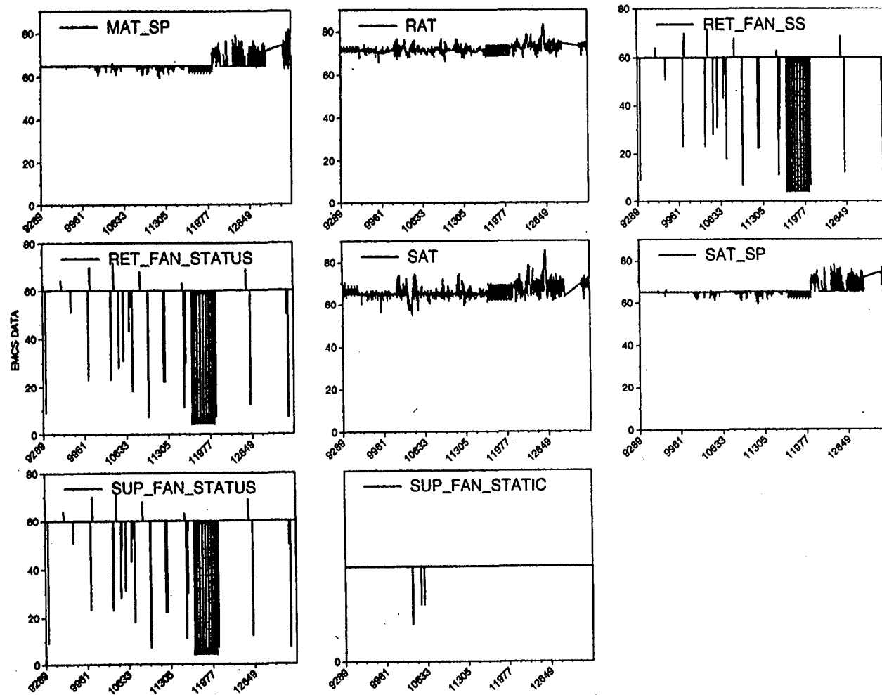
Figure VI-6. Data collected from EMCS in Case Study Building (cont.). The EMCS collected many different types of data, including both energy consumption and operational data.
