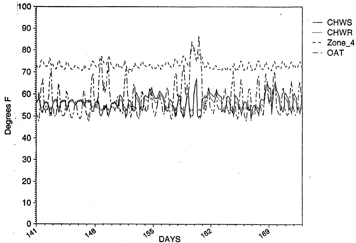
Figure VI-22. EMCS Operational Data: Chilled Water Supply Temperature Control. According to the Sequence of Operations, the setpoint should maintain the lowest cooled zone temperature below 76°F, and the chilled water temperature should not go below 45°F. The figure confirms this, as the chilled water supply temperature was never below 45°F, and the zone temperature was almost always below 76°F. It rose to almost 80°F during the warmest day.
