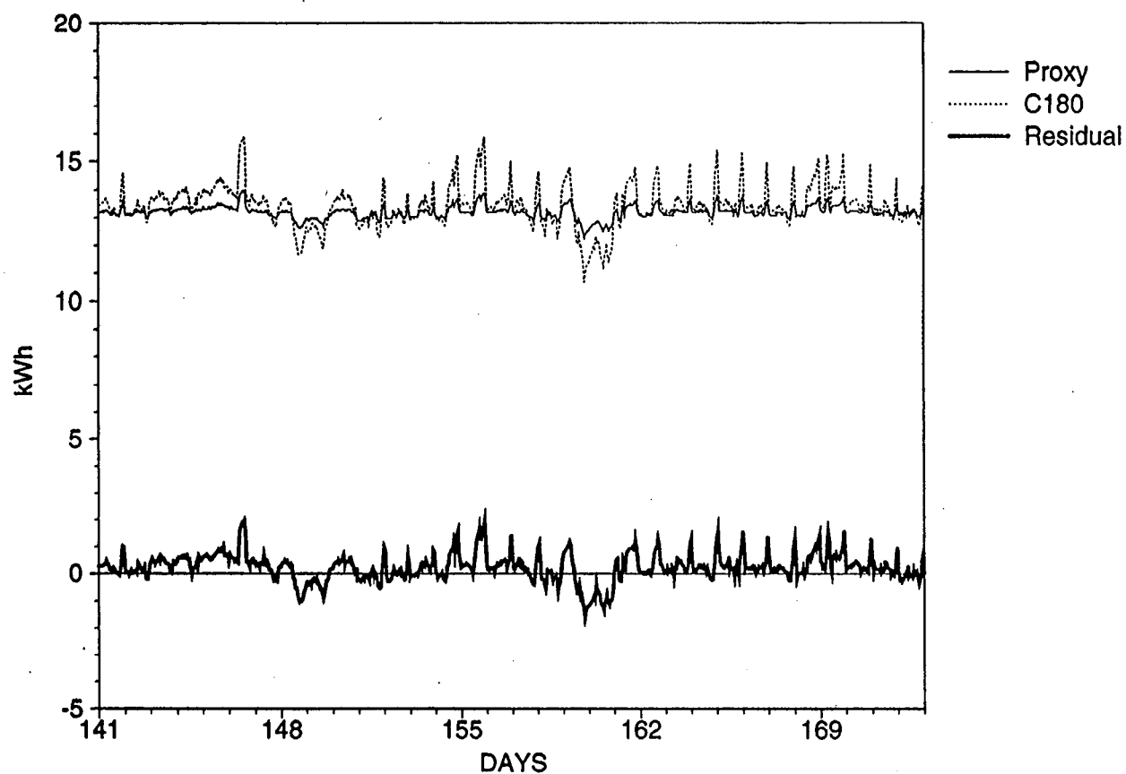
Figure VI-27. EMCS Proxy Measurement: Fan Speed Scaling. Another proxy that could be used to substitute for monitoring the supply fan consumption is speed control. This figure shows the result when the output speed control to the variable frequency drive (in Hertz) is scaled according to one day of monitored data, collected by the dedicated monitoring. Averages for the day were 13.0 kWh and 43.2 Hz, for a factor of 0.30 kWh/Hz. This does a much better job of capturing fluctuations than simply using the fan status. On average, the error was low, but when the consumption is much different from the mean, the error was largest. This suggests that a linear or polynomial regression may provide a better fit.
