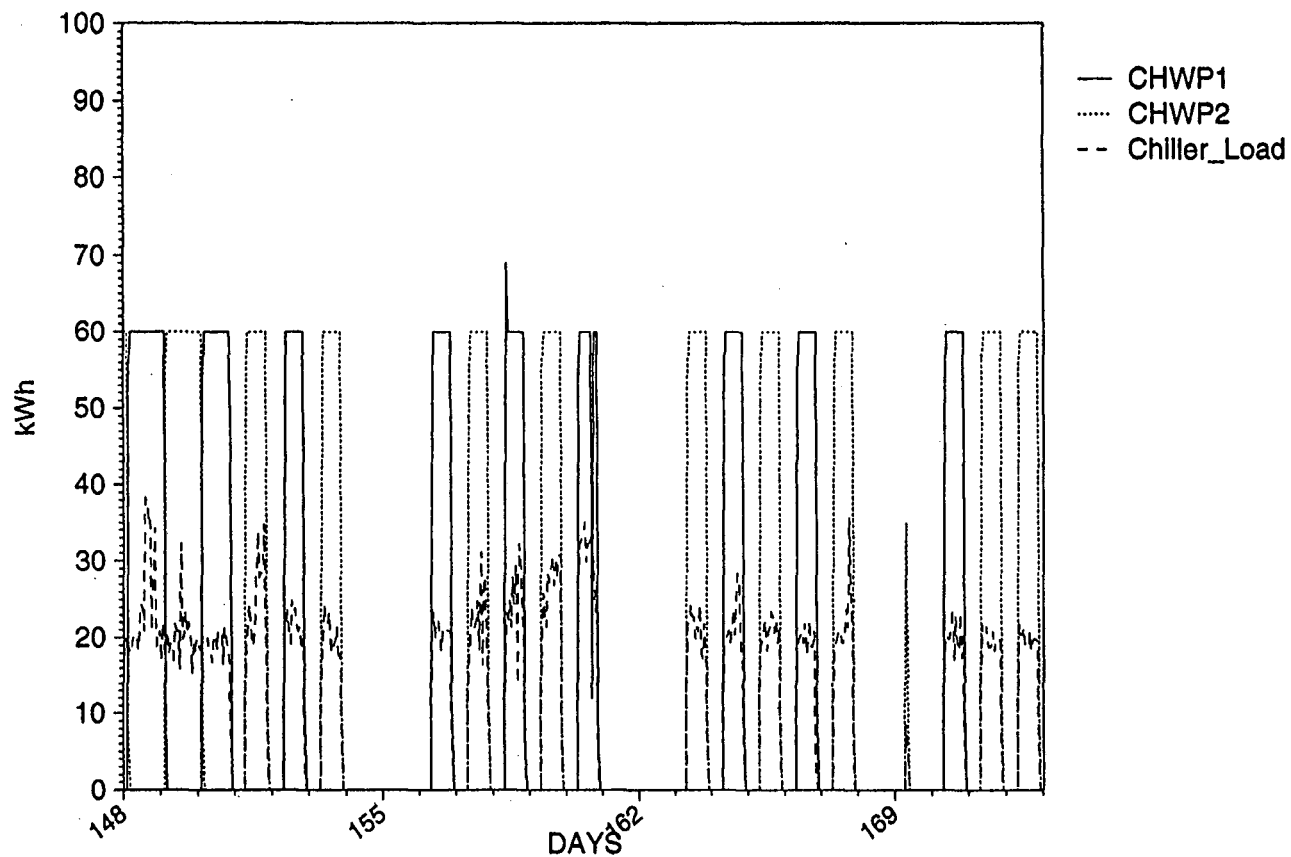
Figure VI-21. EMCS Operational Data: Chilled Water Pump Control. According to the Sequence of Operations, the pumps should operate only when cooling is required, and the two pumps should alternate daily. The figure confirms both characteristics of operation, as the pumps never operate when there is no call for cooling, (indicated by the chiller load point), and they alternate daily.
