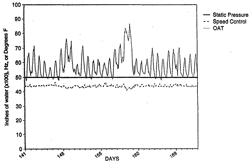
Figure VI-15. EMCS Operational Data: Fan Control. It may be easier to diagnose operational problems from EMCS-collected operational data than from consumption data. For example, many of the monitored points can be compared with the expectations from the Sequence of Operations (shown in Figure VI-14). This figure shows control of the supply fan. Although a variable frequency drive was installed, the system is constant volume, and the drive is used simply to reduce the flow of an oversized fan. According to the Sequence of Operations, the fan should run continuously, and maintain a static pressure of 0.8 inches of water. As the graph shows, the static pressure is a constant 0.5 inches, rather than 0.8 inches. This is because the pressure reduction from removing the fan inlet vanes was greater than expected, resulting in the ability to operate at with a lower static pressure setpoint, and more savings from the retrofit than anticipated. The monitored value of the static pressure was always 0.5 inches, although it varied somewhat around that value. The system did not report sufficient significant digits to determine static pressure more accurately. After this was pointed out to the EMCS operator, the format was changed for the point to show more significant digits. This does not affect the operation at all, just the output format. The speed control to the VFD on the supply fan was fairly constant.
