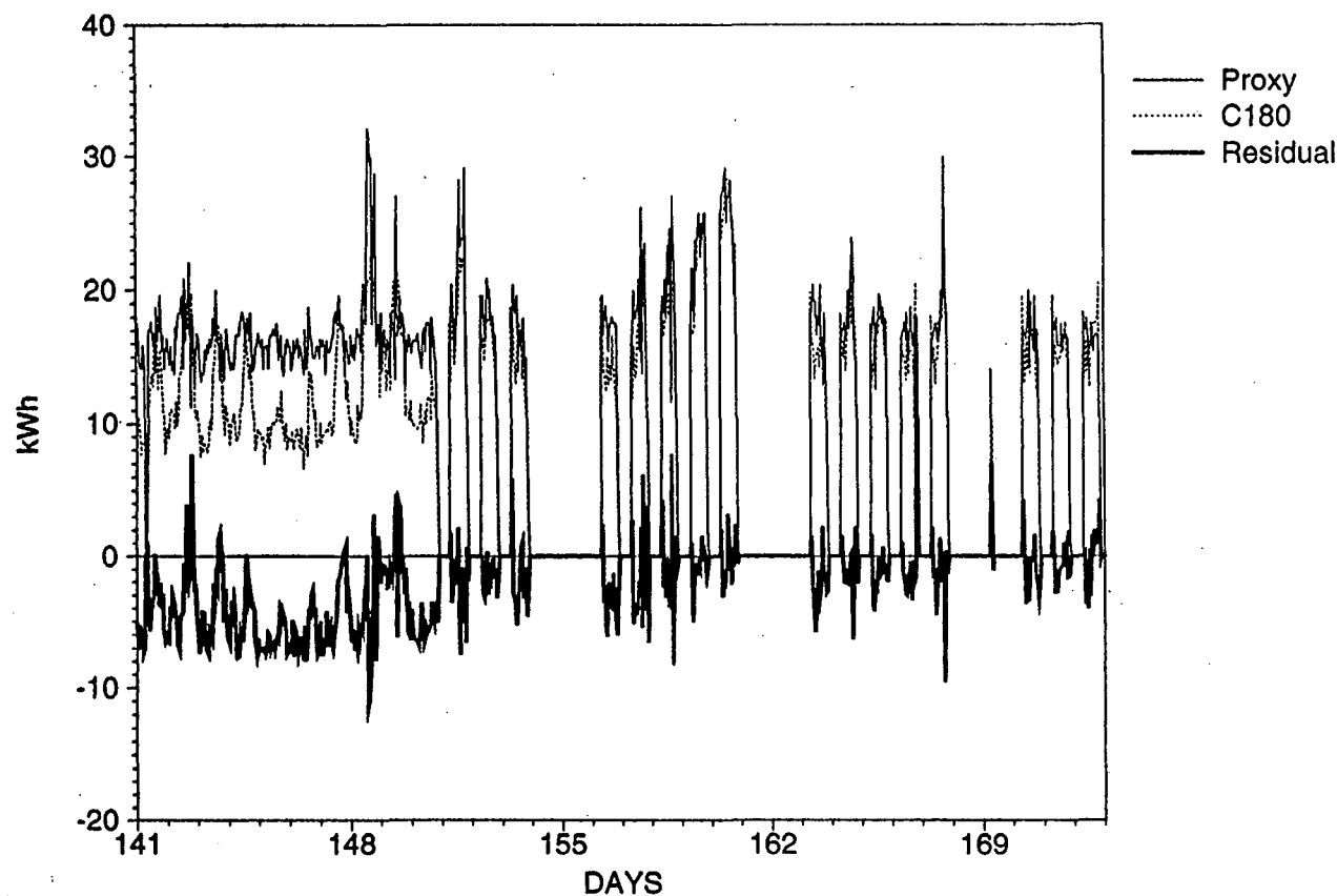
Figure VI-26. EMCS Proxy Measurement: Chiller. This figure shows a proxy for chiller energy consumption. The chiller is operated with a PID (Proportional-Integral-Differential) control loop, where the output control signal is based on the difference between the chilled water return temperature, and its setpoint. The output of this PID loop is the "chiller loading" signal, which goes out to the chiller (the chiller has a Honeywell controller of its own, and only required this chiller loading signal). This load signal might serve as a proxy for chiller consumption. This proxy should be multiplied by the chiller status variable, since it is possible for the PID loop to calculate a load while the system is actually turned off. The proxy was calculated by using one day of data collected by the dedicated monitoring to calculate a scaling factor. The averages used were 16.7 kWh, and 19.9% chiller loading, for a factor of 0.84kWh/%. As the residual indicates, the error in using this proxy is quite large during some hours.
