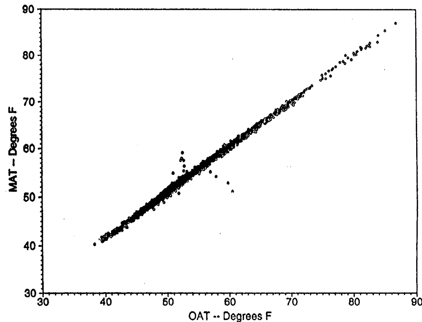
Figure VI-18. EMCS Operational Data: Economizer Control (cont.). This graph shows the striking correlation between mixed air and outside air temperatures throughout the monitoring period, over a wide range of temperatures. This indicates some sort of problem: the mixed air temperature should equal the outside air temperature when the economizer is on full outside air operation. However, when the economizer is off—when the it is cold outside and outside air is at a minimum—the mixed air temperature should be somewhere between the outside air temperature and the return air temperature (since it should be a mixture of the two). Two possible problems that could cause data such as these are incorrect sensor placement—perhaps the mixed air sensor is placed in the wrong run of duct—or faulty operation of the economizer dampers. Recall that the outside air fraction is a control signal sent to the dampers, not a verification of actual outside air fraction, so that it is not known for sure that the dampers are responding to the signal. Unfortunately, no data on the heating side had been collected, and with the existing data it was impossible to determine whether the fault was in the sensor or the economizer. However, since this EMCS always has access to hourly data for all points, for the previous 24 hours, it was possible to go back and review the previous day's operation.
