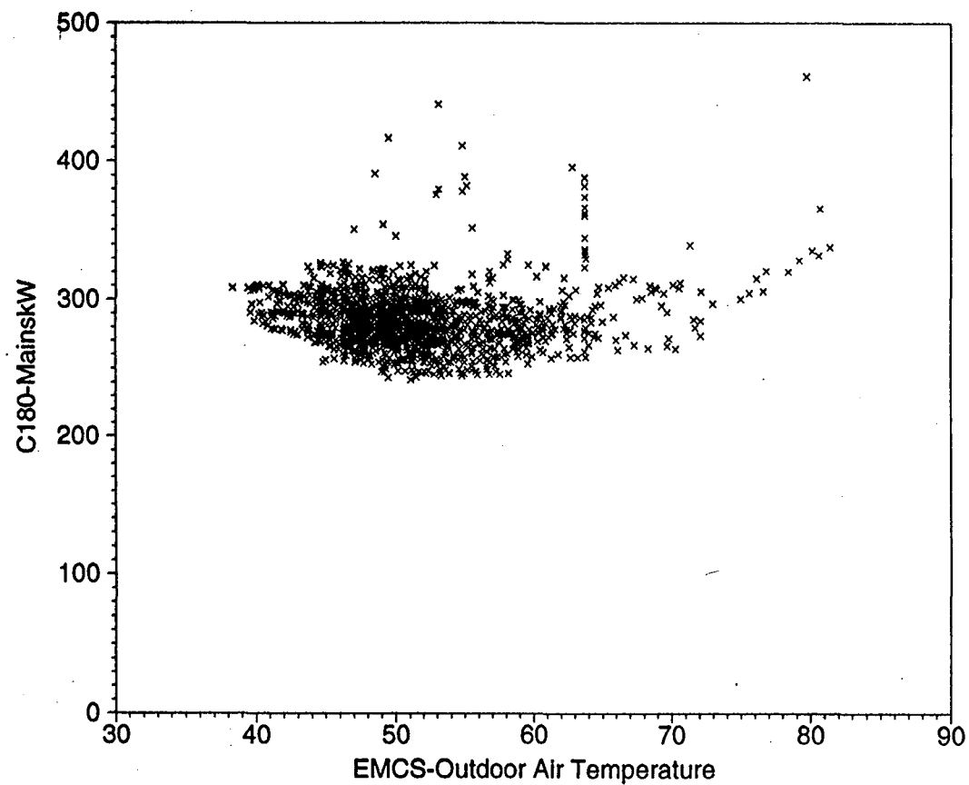
Figure VI-13. EMCS Occupancy Data (cont.). This figure shows the whole-building consumption (measured by the dedicated monitoring) as a function of outdoor temperature (measured by the EMCS), for "Unoccupied" hours. Clearly there is a very different pattern of consumption during the unoccupied hours—for example, there is much less scatter—although the consumption is still quite high.
