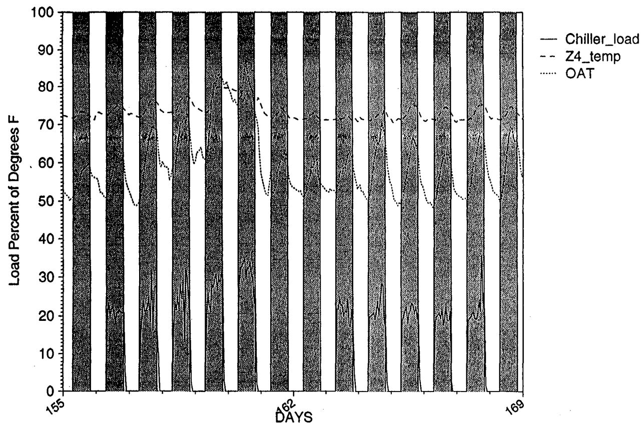
Figure VI-20. EMCS Operational Data: Optimal Stop and Start Control. According to the Sequence of Operations, the chilled water system should operate between 7am and 8pm. Optimal start should ensure that the temperature in the warmest zone (1, 4, 8 or 9) is below 76°F by 7am. The shaded periods in the figure correspond to the occupied period, as indicated by the "Occupied" variable. The chiller loading, (a calculated output), and one of the zone temperatures are shown, as is the outdoor air temperature. The temperature in the occupied zone is above 76°F in the morning only on one day, when the nighttime temperature was unusually high. The temperature that morning was about 79°F. The chiller did not turn on any earlier that morning, indicating that optimal start was not invoked, or that it was not dynamically invoked to start earlier when an unusually warm night occurred. The call for cooling was always zero during unoccupied hours.
