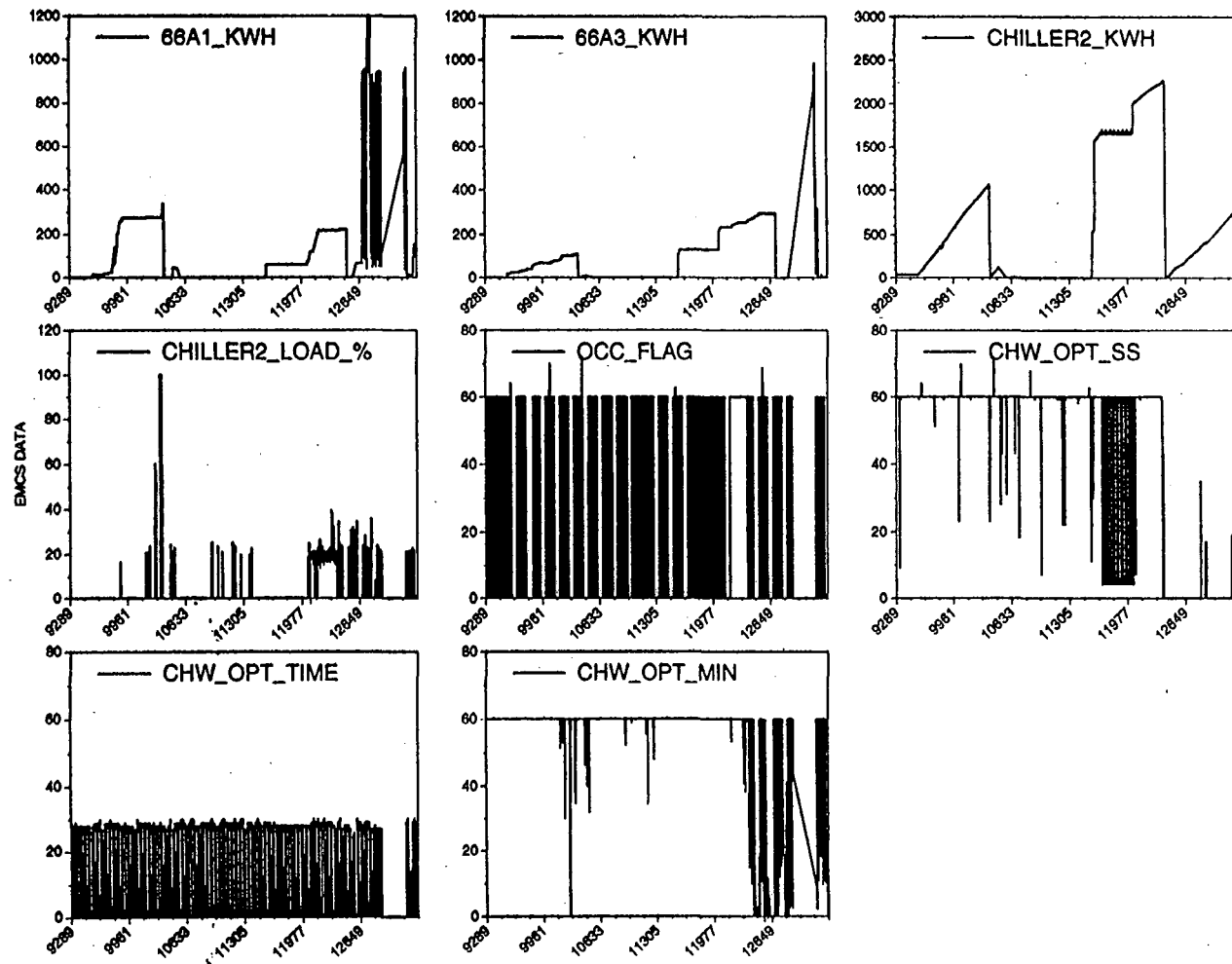
Figure VI-9. Data collected from EMCS in Case Study Building (cont.). The EMCS collected many different types of data, including both energy consumption and operational data.
