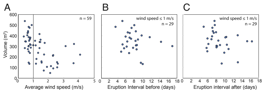
Fig. 8. (A) Volume of erupted water estimated from the Tantalus Creek streamgage and wind speed for 59 eruptions. This plot shows that lower volumes are related to higher wind speed. (B) Volume of erupted water and preceding interval for 29 eruptions occurring under low wind speed ( \leq 1 m/s; line in A marks this threshold). (C) Volume of erupted water and interval after eruption for the same population as in B.
