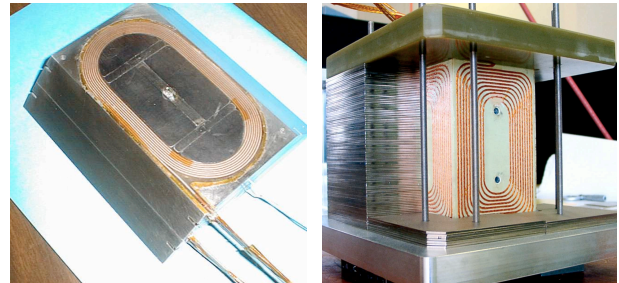
Fig. 1: Coil layout. LLNL (left), AML (right).
