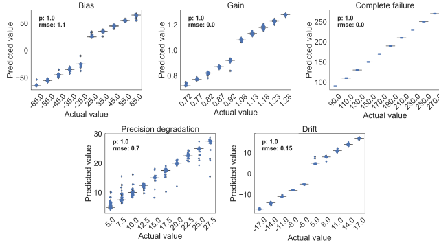
Figure 9: Fault reconstruction (airflow)
