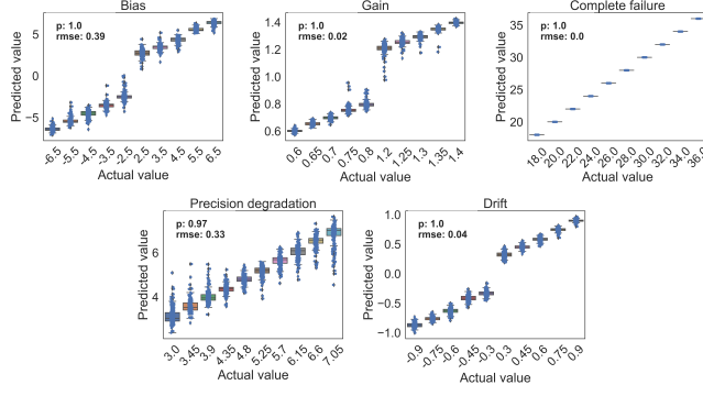
Figure 8: Fault reconstruction (supply temperature)
