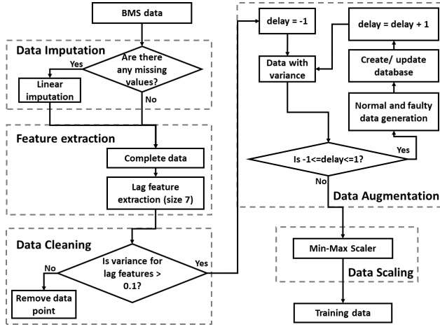
Figure 3: Training Data Generation
