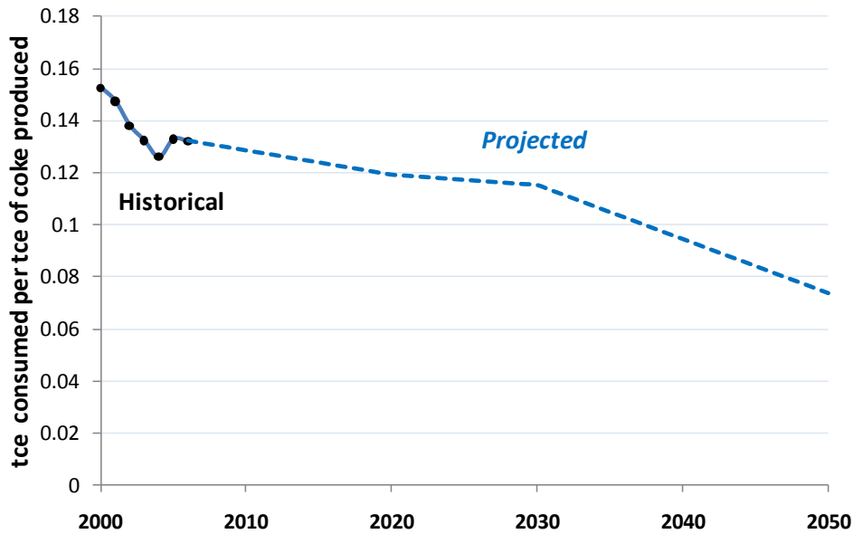
Figure 31 Final Energy Intensiveness of Coking, 2000 - 2050
