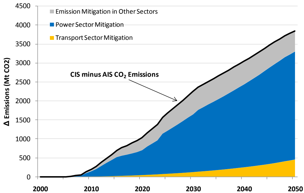
Figure 66 CO 2 Emission Mitigation under AIS by Source
