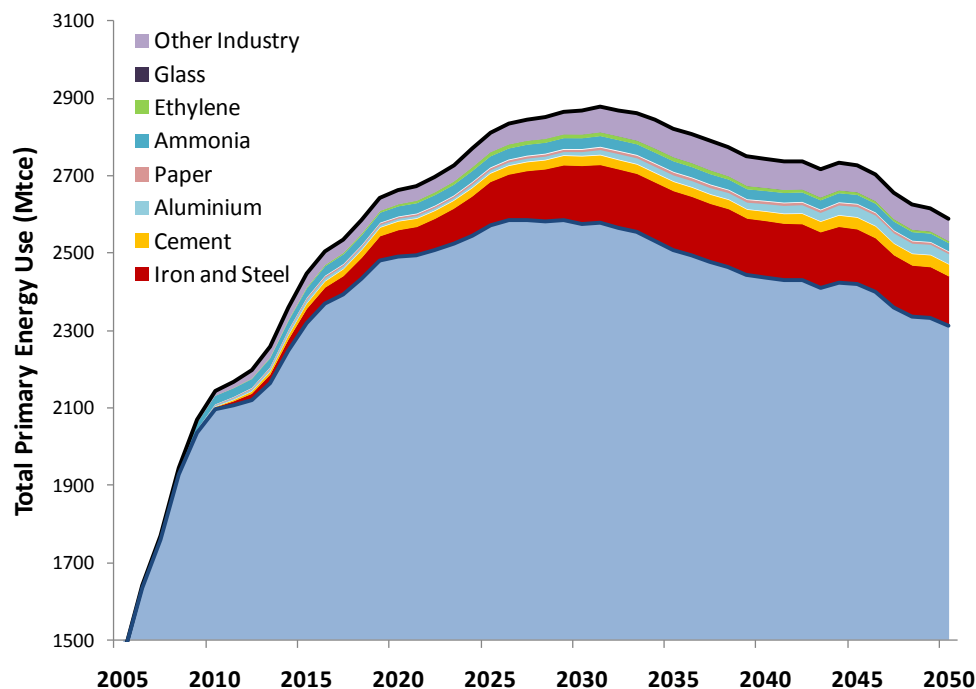
Figure 54 Industrial Energy Savings Potential by Subsector
