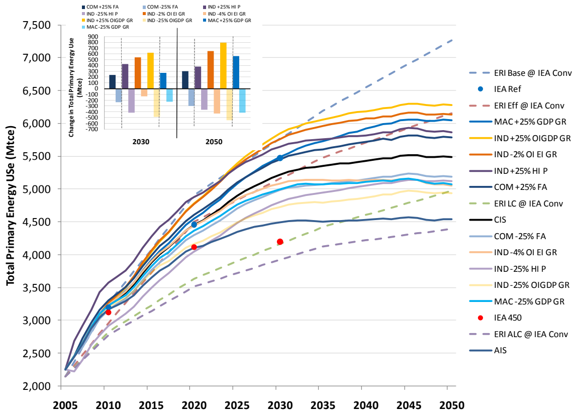
Figure ES-5: Sensitivity Analysis Scenario Results with Greatest Uncertainty
