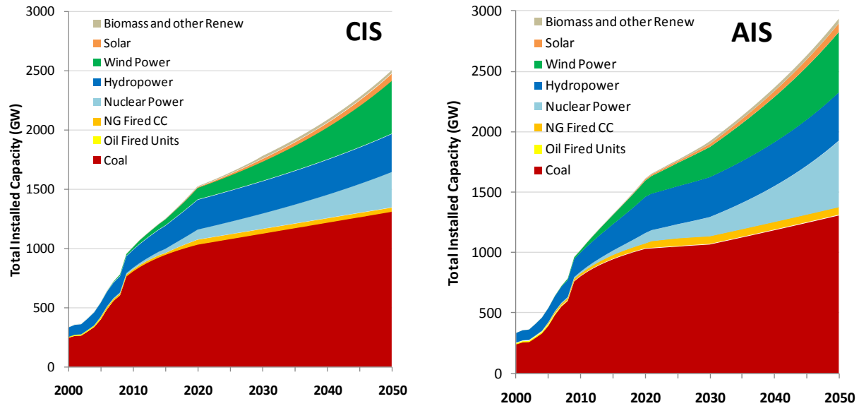
Figure 25 Power Generation Capacity (Excluding Coal) by Fuel Source, CIS and AIS Scenarios
