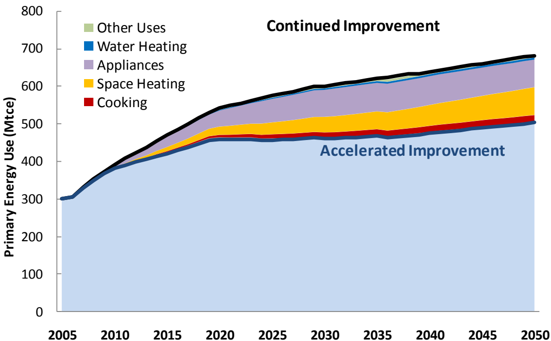
Figure 49 Residential Primary Energy Use and Potential Reductions by End-Use
