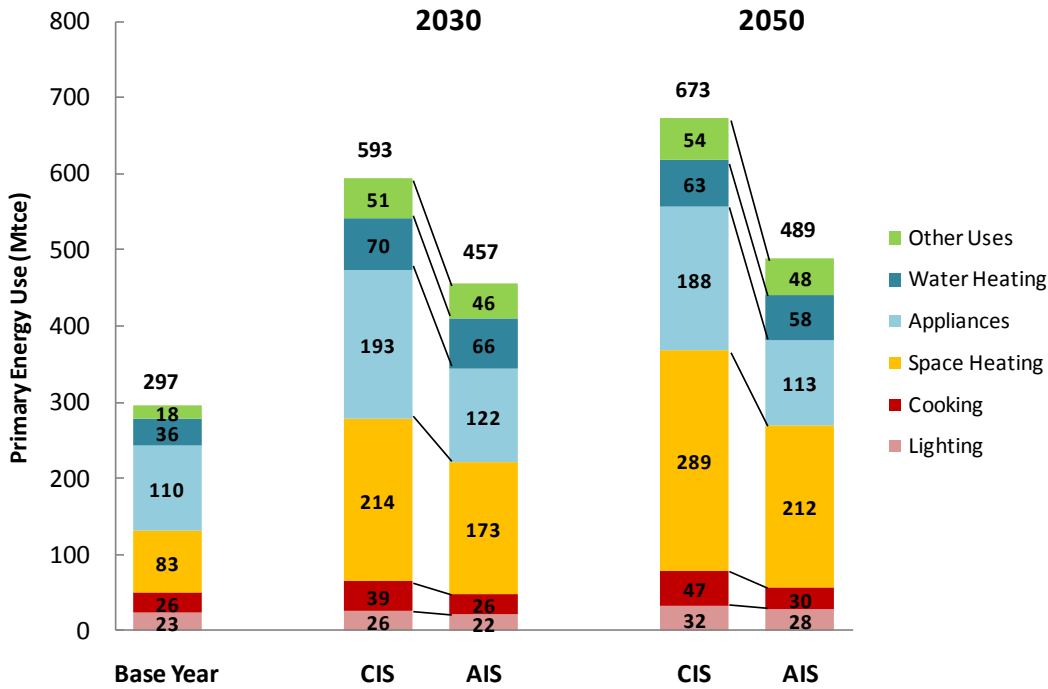
Figure 47 Residential Primary Energy Consumption by End-Use
