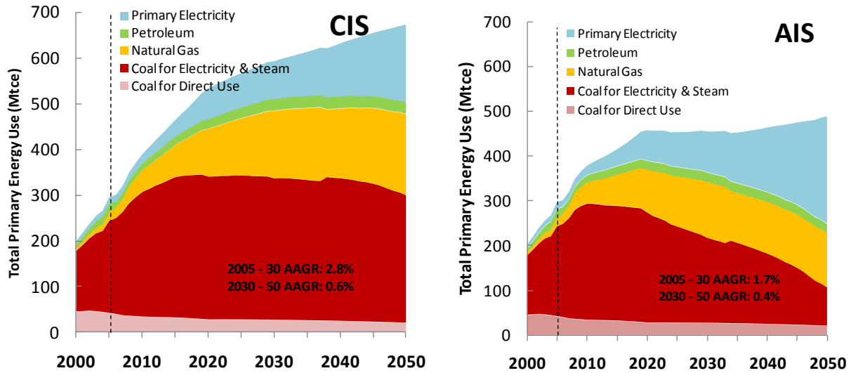
Figure 48 Residential Primary Energy Consumption by Fuel, CIS and AIS
