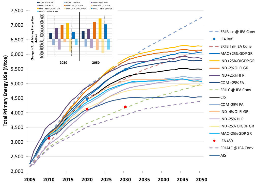
Figure 69 Sensitivity Analysis Scenario Results with Greatest Uncertainty
