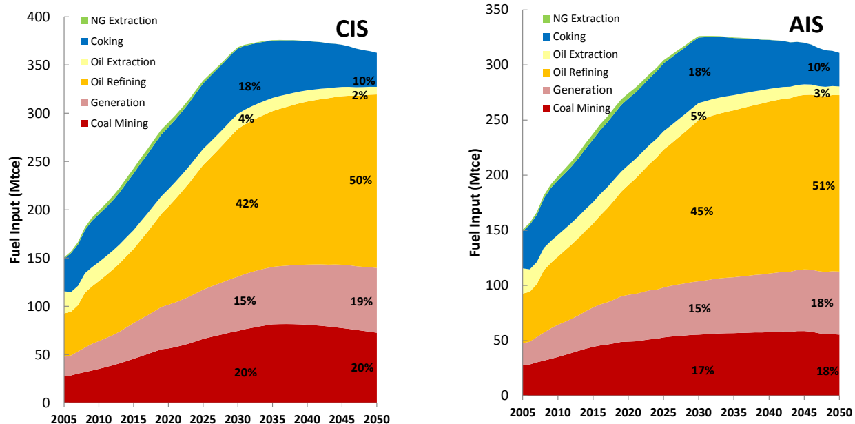
Figure 68 Fuel Input to Energy Extraction and Processing, CIS and AIS Scenarios
