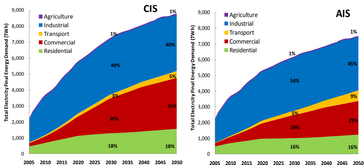
Figure 46 CIS and AIS Electricity Final Demand by Sector, 2005-2050
