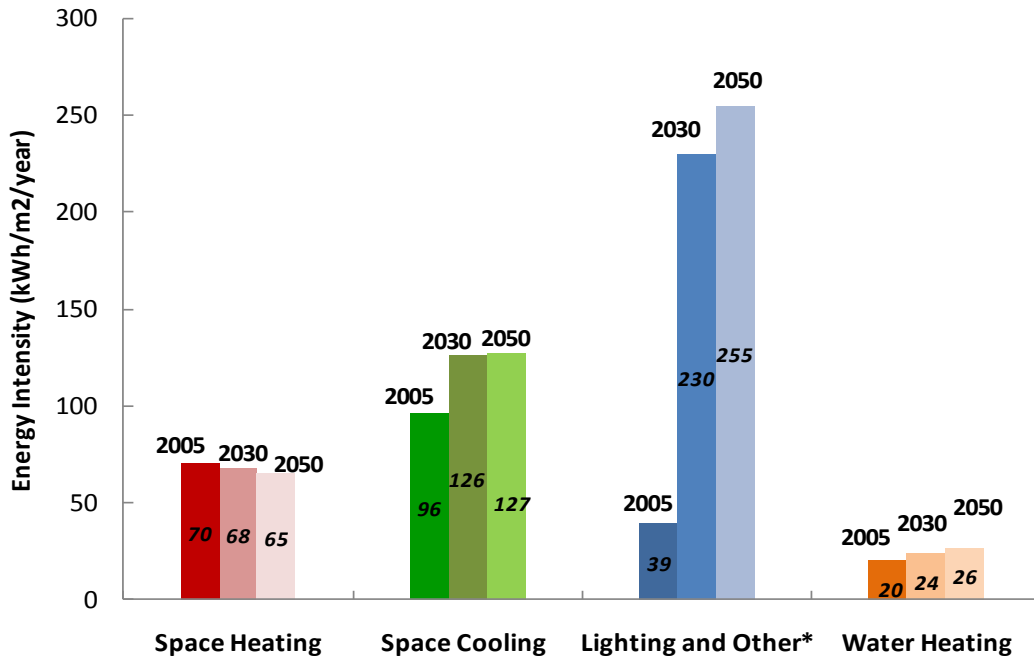
Figure 9 Retail Buildings Energy Intensity by End-Use
