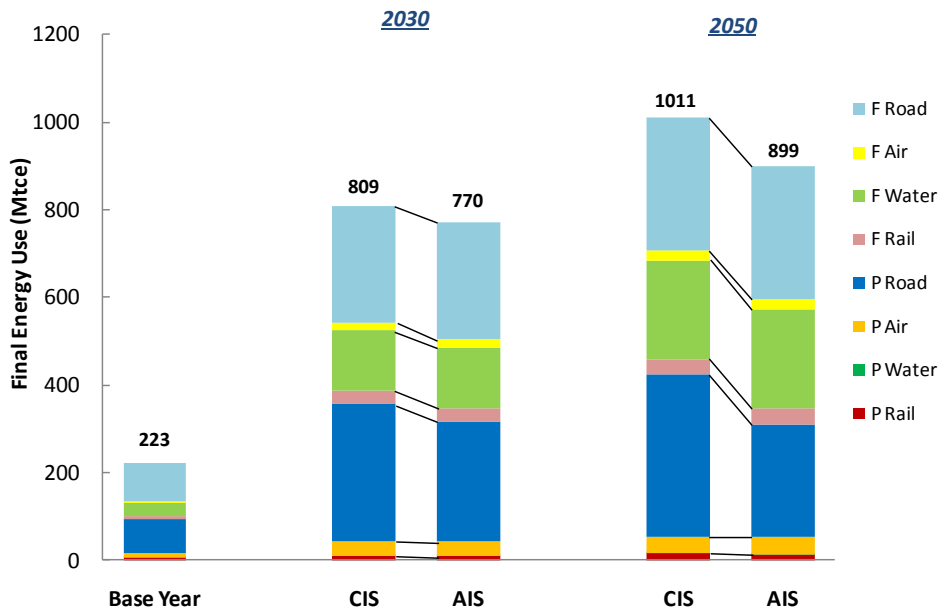
Figure 56 Transport Final Energy Consumption by Mode
