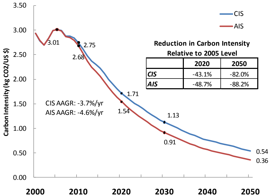
Figure 37 Carbon Intensity Reductions by Scenario, 2000 - 2050
