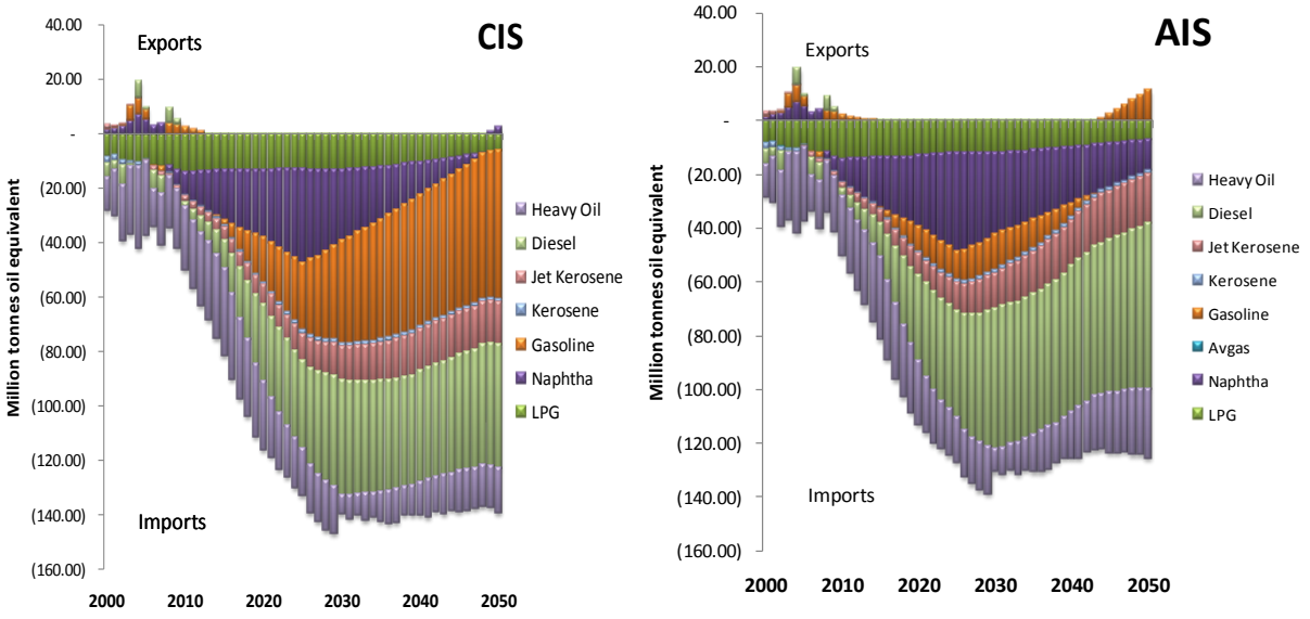
Figure 60 Major Oil Product Imports and Exports
