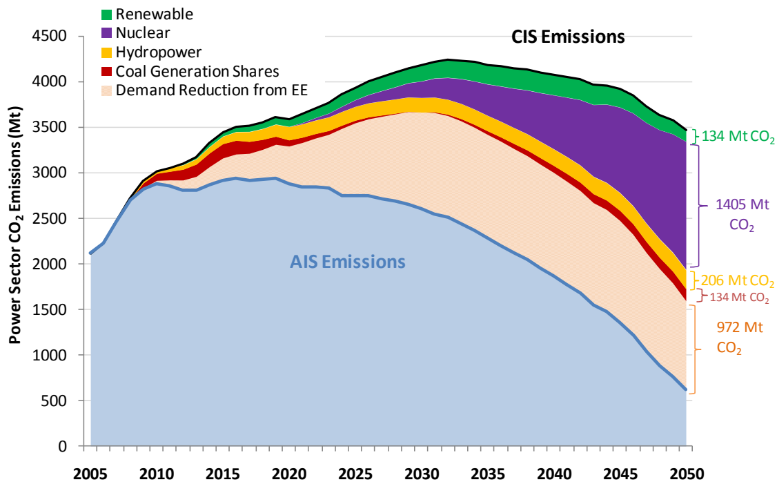
Figure 67 AIS Power Sector CO 2 Emissions Reduction by Source
