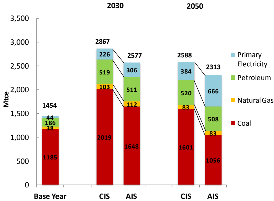
Figure 52 Industrial Primary Energy Use by Fuel
