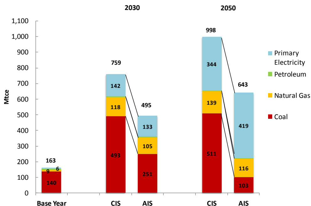
Figure 51 Commercial Primary Energy Use by Fuel
