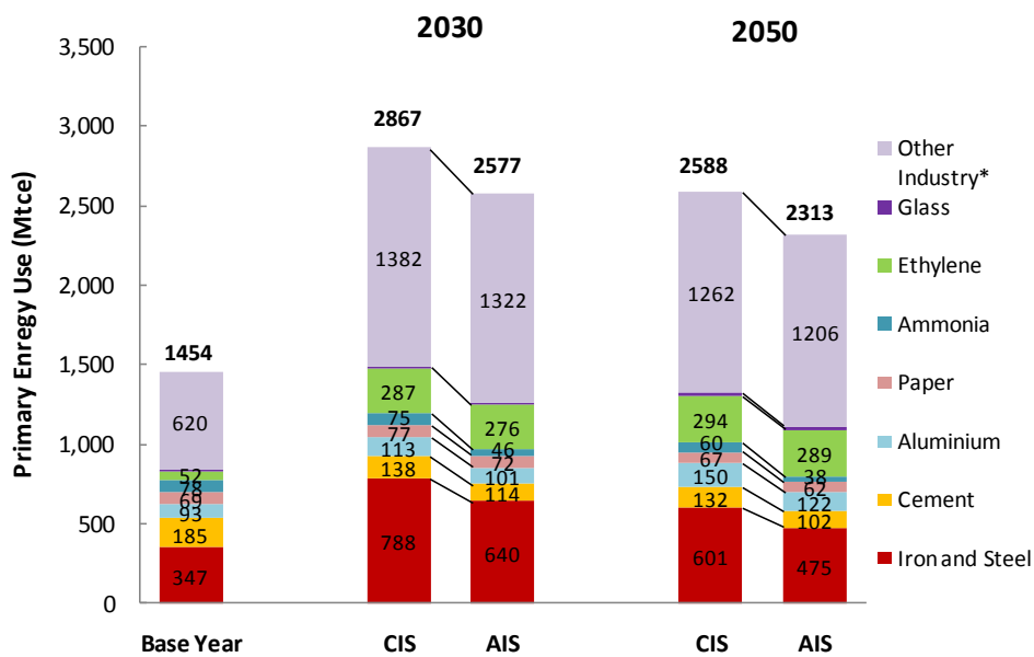
Figure 53 Industrial Primary Energy Use by Subsector
