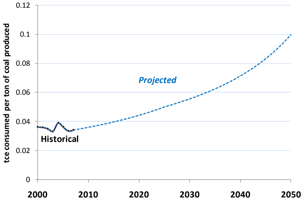
Figure 29 Final Energy Intensiveness of Coal Mining
