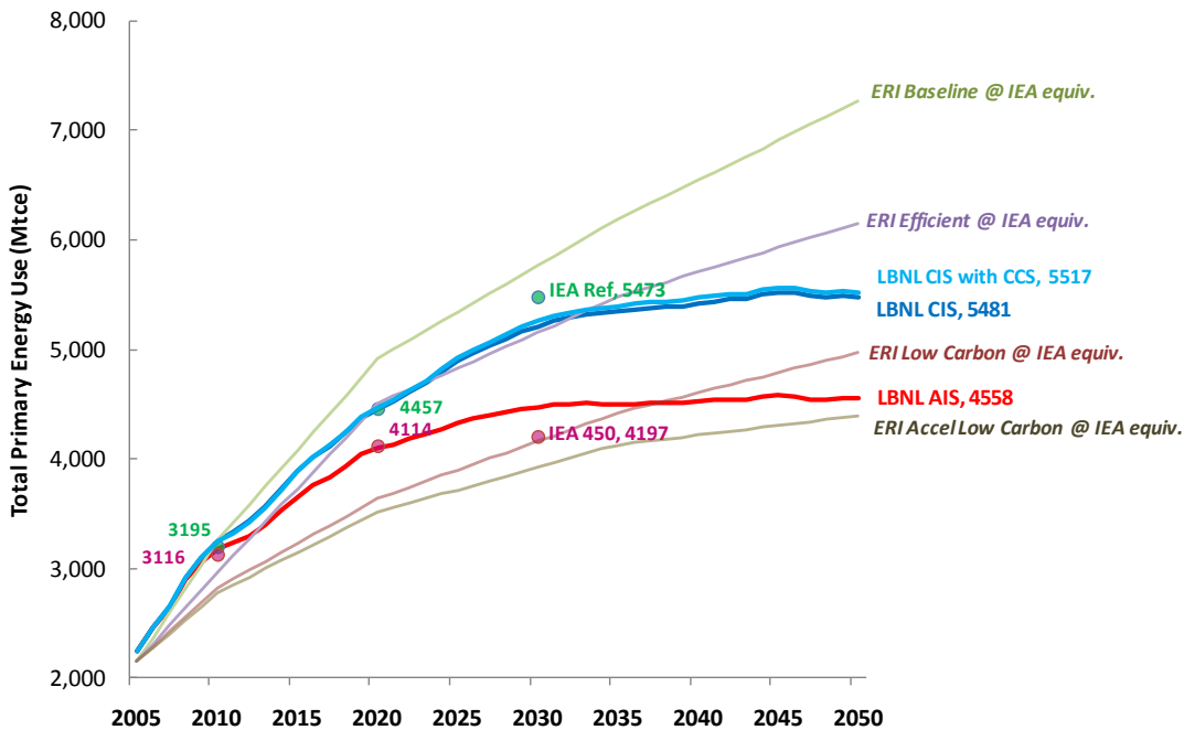
Figure 33 Primary Energy Consumption in Different Scenarios
