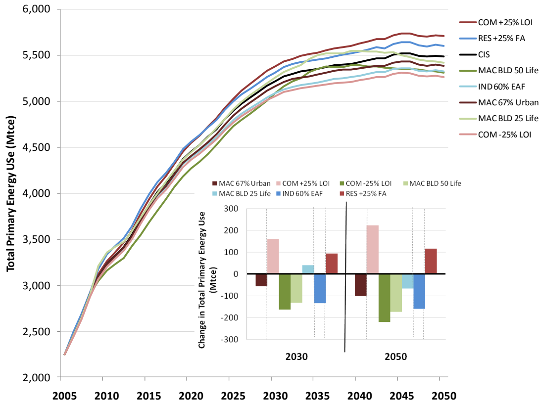
Figure 70 Sensitivity Analysis Scenario Results of Medium Uncertainty
