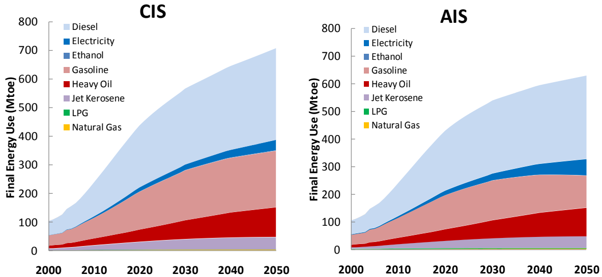
Figure 57 Transport Energy Consumption by Final Fuel, CIS and AIS Scenarios
