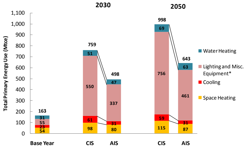
Figure 50 Commercial Primary Energy Consumption by End-Use
