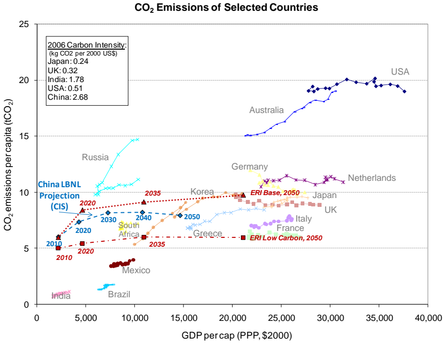
Figure ES-2: International trends in CO 2 emissions and GDP per capita, with China scenarios to 2050
