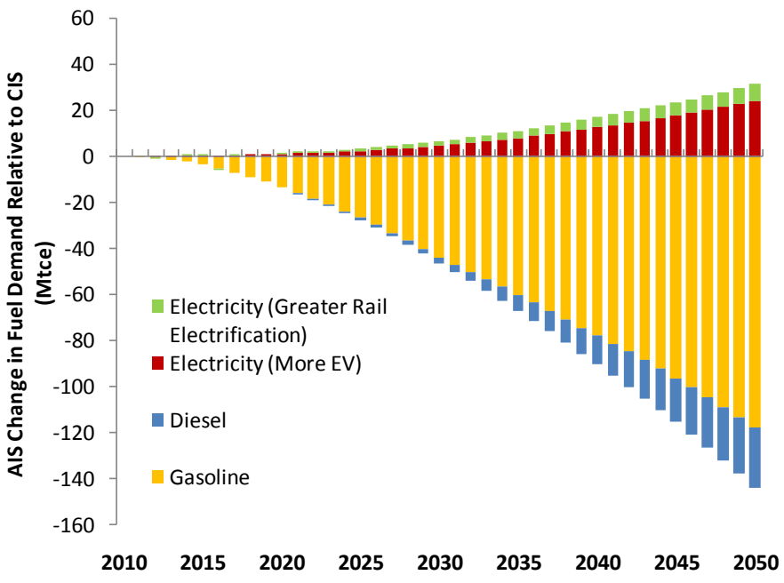
Figure 61 AIS Change in Transport Final Energy Demand Relative to CIS
