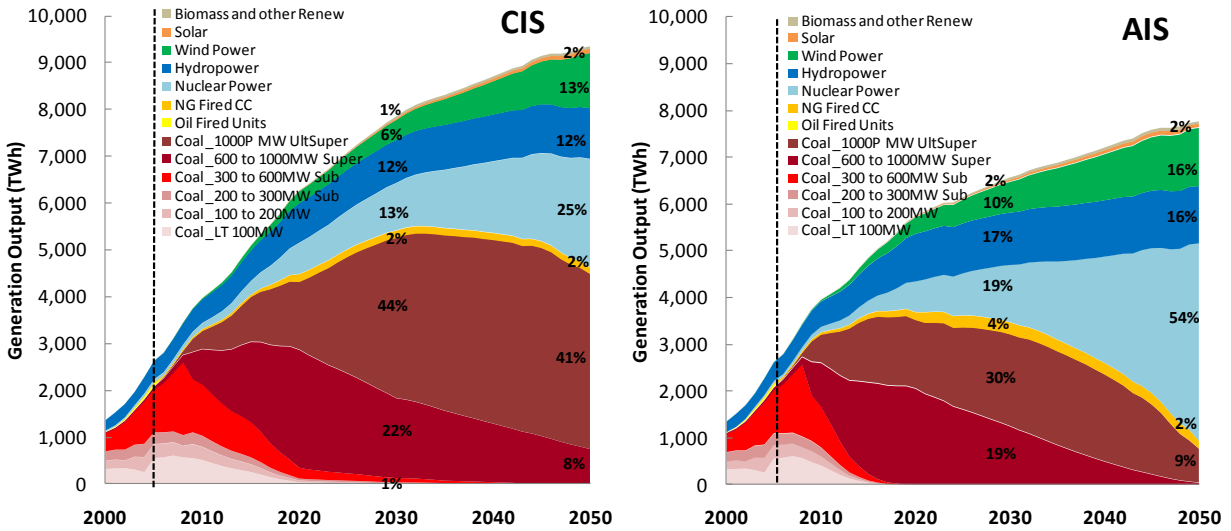
Figure 64 Electricity Generation by Fuel, CIS and AIS Scenarios
