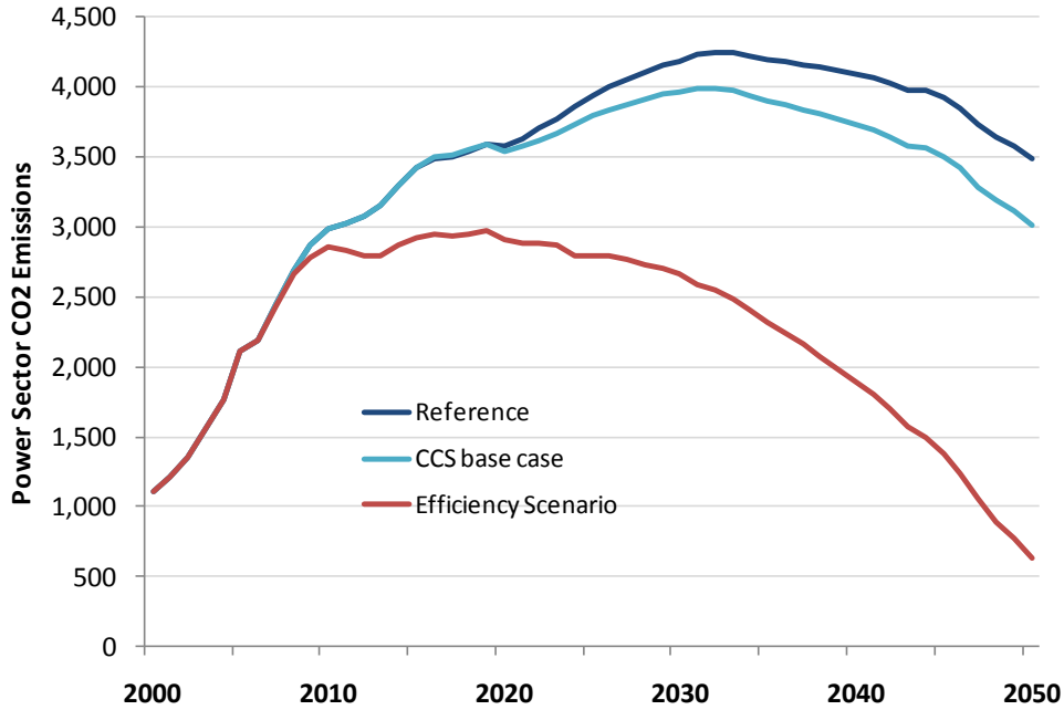
Figure 65 Power Sector CO 2 Emissions under Three Scenarios
