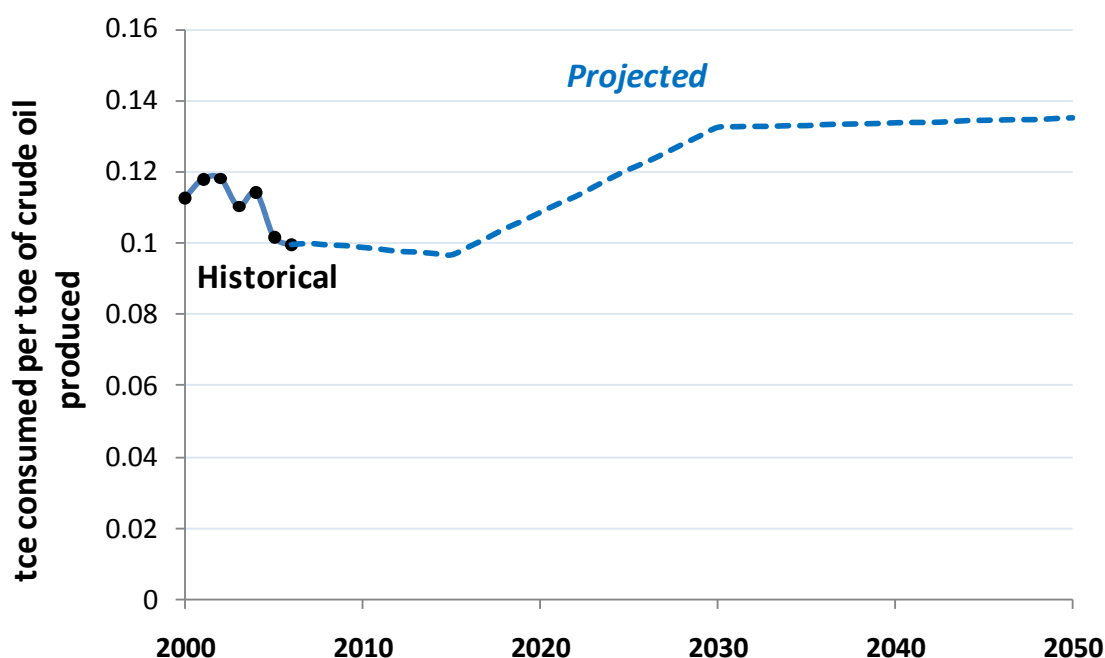
Figure 32 Final Energy Intensiveness of Oil Refining, 2000-2050
