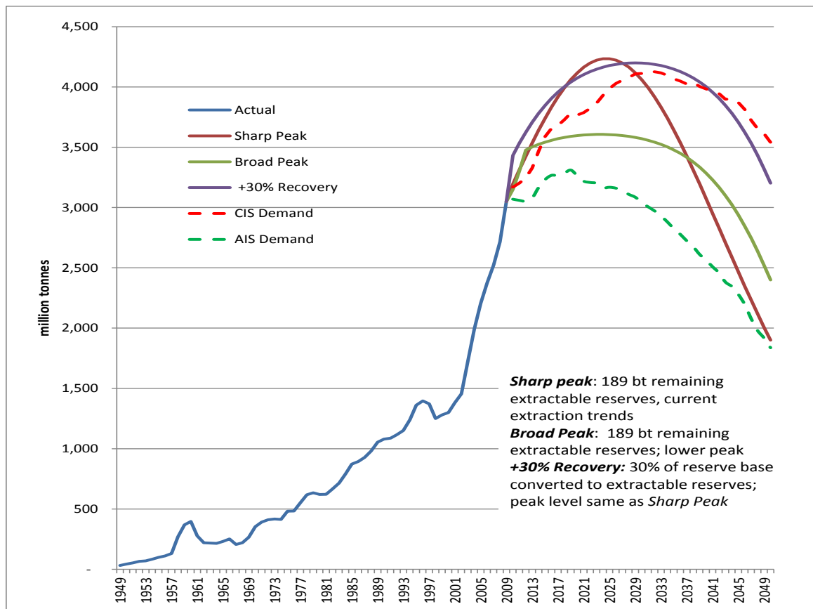
Figure 71 Coal Demand and Extraction Profiles
