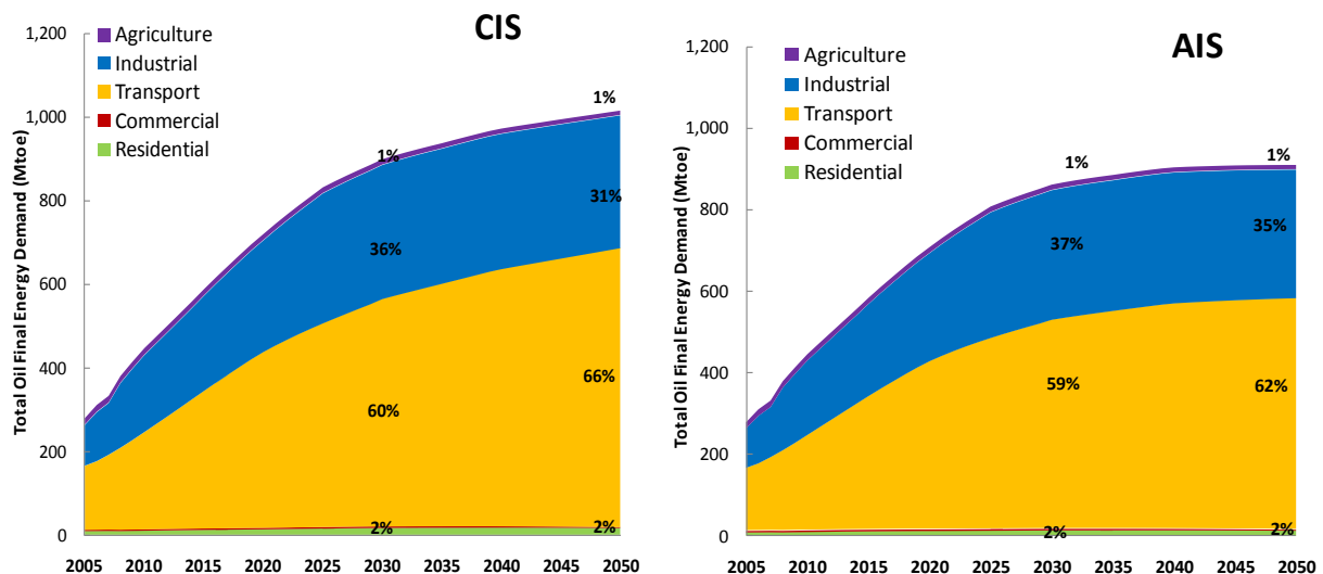
Figure 45 CIS and AIS Oil Final Demand by Sector, 2005 - 2050
