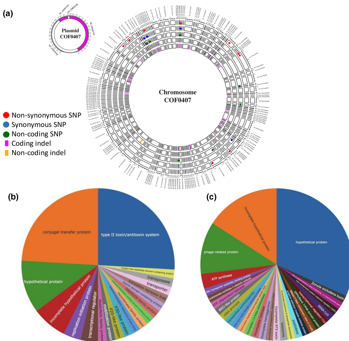
Fig. 2. Mutations shared by the entire Apulian population. The types (one circle corresponding to one mutation type) and positions of the shared mutations are shown on the Costa Rican coffee strain genome, COF0407 (a). The names appearing outside the circle correspond to the names of COF0407 contigs (a). Functions of the proteins with mutations (SNPs or indels) encoded in the plasmid (b, n=54 ) and chromosome (c, n=63 ).
