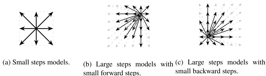
Figure 1.2: Models of walks.
