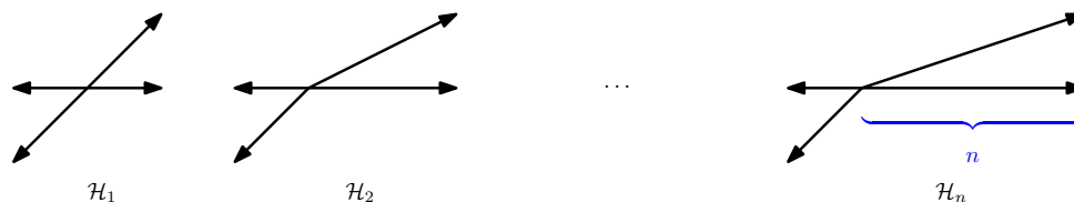
Figure E.1: The stretched Gessel models.
