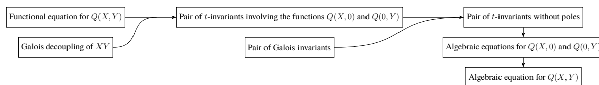
Figure 2.1: Summary of the strategy for proving algebraicity.
