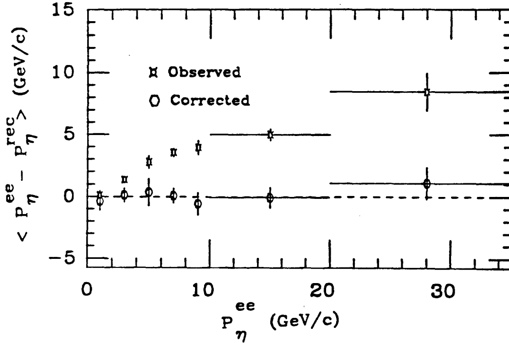
Figure 4.9: The average difference, P_{\eta}^{ee} - P_{\eta}^{rec} , for different ranges of P_{\eta}^{ee} . The quantity is shown before and after the energy corrections were applied.
