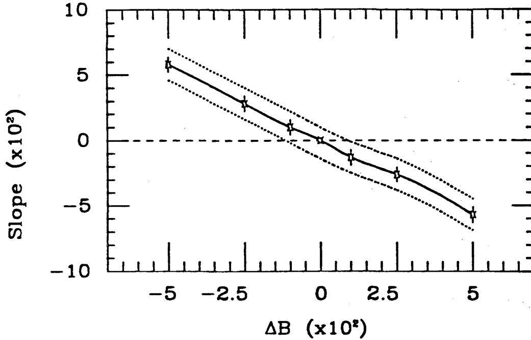
Figure 4.14: The slope variation of a fit to the conversion sample (Figure 4.4) as a function of the change of the linear coefficient of the clustered energy correction (Eq. 4.4.)
