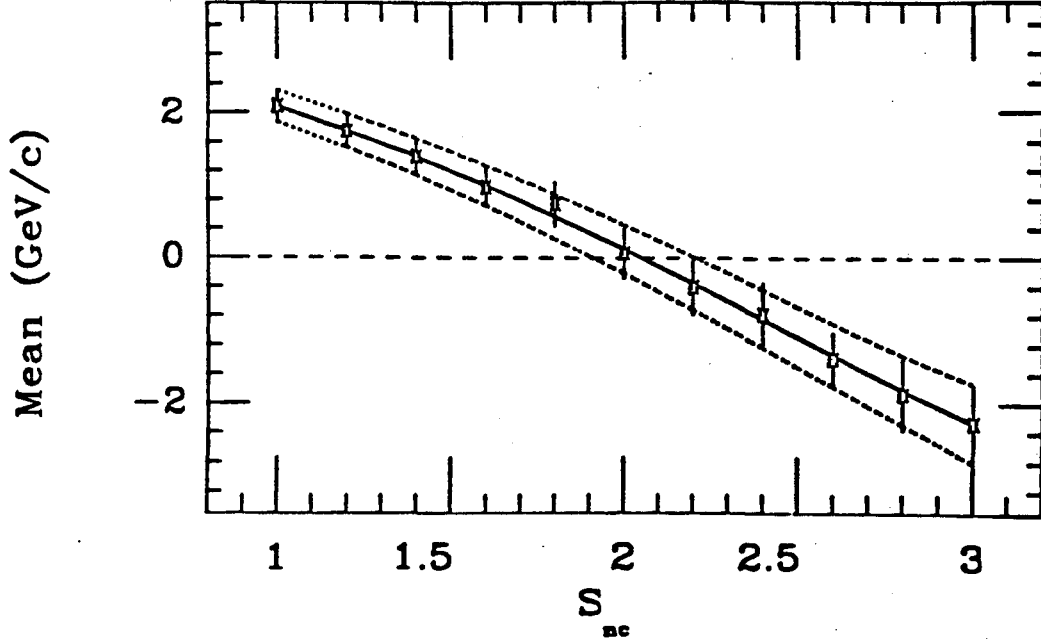
Figure 4.16: The mean P_{\eta}^{ee} - P_{\eta}^{rec} for different values of S_{nc} . The sample of Z events used does not contain any clusters with E_T > 10 GeV so the entire \cancel{E}_T correction comes from the S_{nc} scale factor. The dotted lines are the 1\sigma limits.
