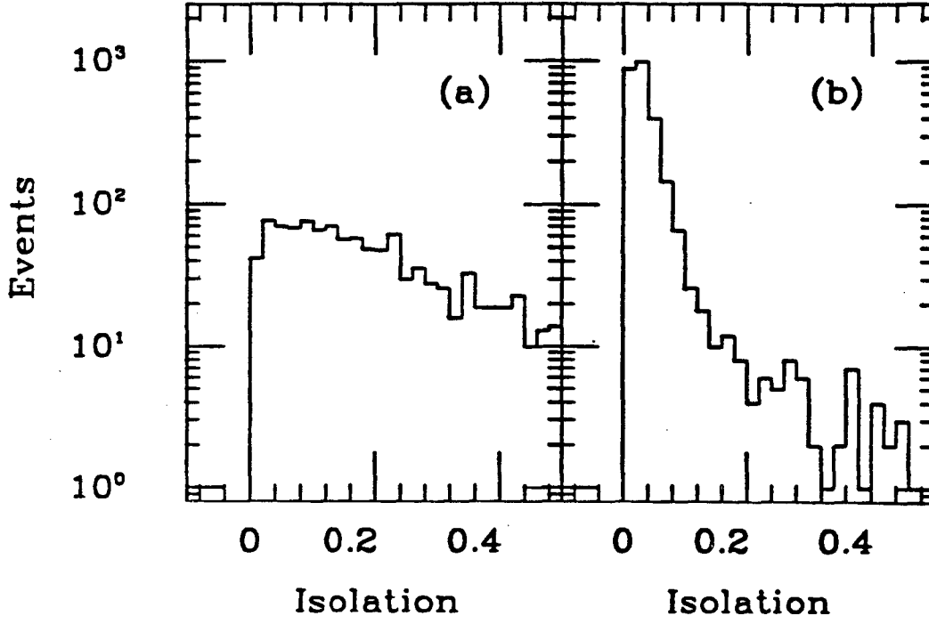
Figure 3.7: Electron Isolation for the (a) Background sample and (b) Signal sample without an isolation cut.
