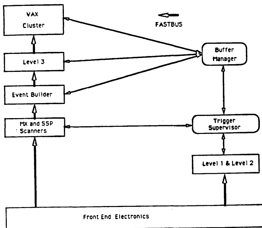
Figure 2.8: A schematic diagram of the data acquisition system. The system is based primarily on a FASTBUS network.
