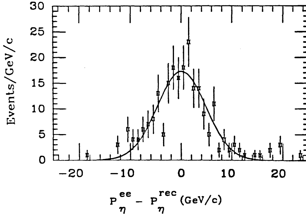
Figure 4.10: The difference, P_{\eta}^{ee} - P_{\eta}^{rec} , fit to a Gaussian distribution after calorimeter energy corrections is shown. The mean is 0.09 \pm 0.32 GeV/c and \sigma = 4.8 GeV/c. The width of the distribution is a measure of the resolution for the P_T measurement (see Section 4.4.3).
