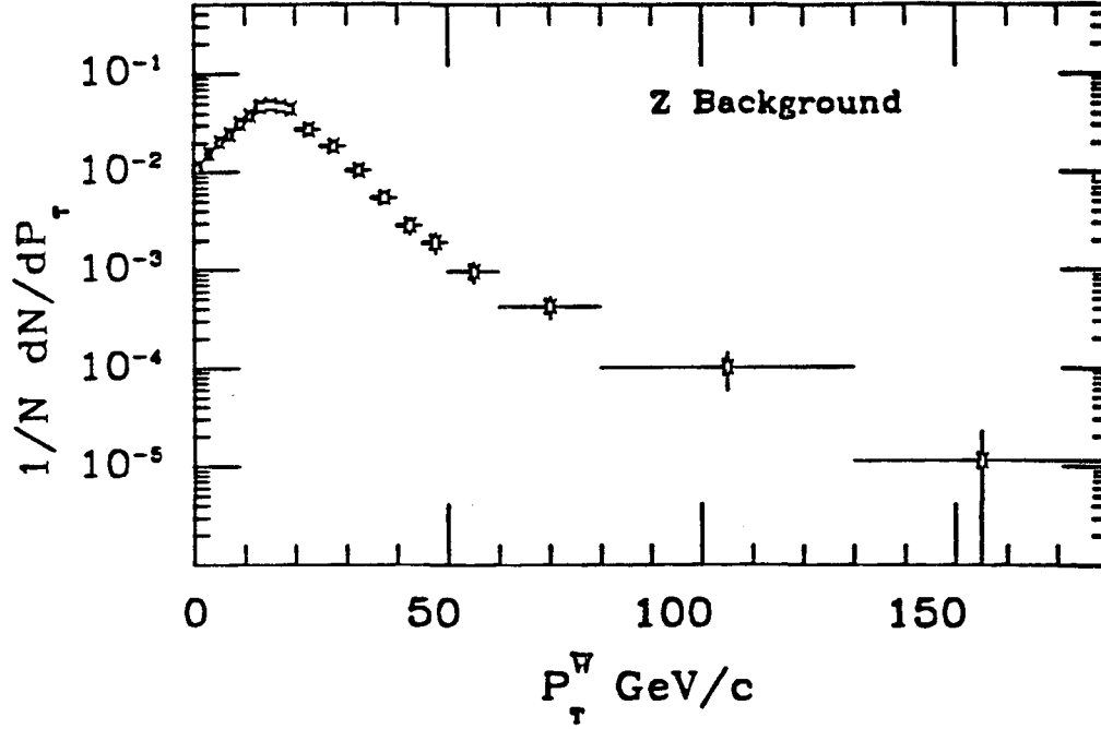
Figure 3.9: The P_T^W spectrum for Z background. The P_T^W is found with the highest E_T electron and the \cancel{E}_T . The spectrum is different from the P_T^Z of standard Z events. The distribution was determined from a Monte Carlo program with detector simulation.
