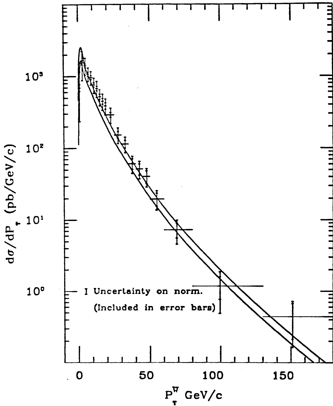
Figure 6.1: The differential cross section, d\sigma/dP_\tau . The data points are fully corrected. The solid band is a next-to-leading order prediction [20] with HMRS(B) structure functions and \Lambda_{QCD} = 190 MeV. The width of the band represents the theoretical uncertainty of the prediction.
