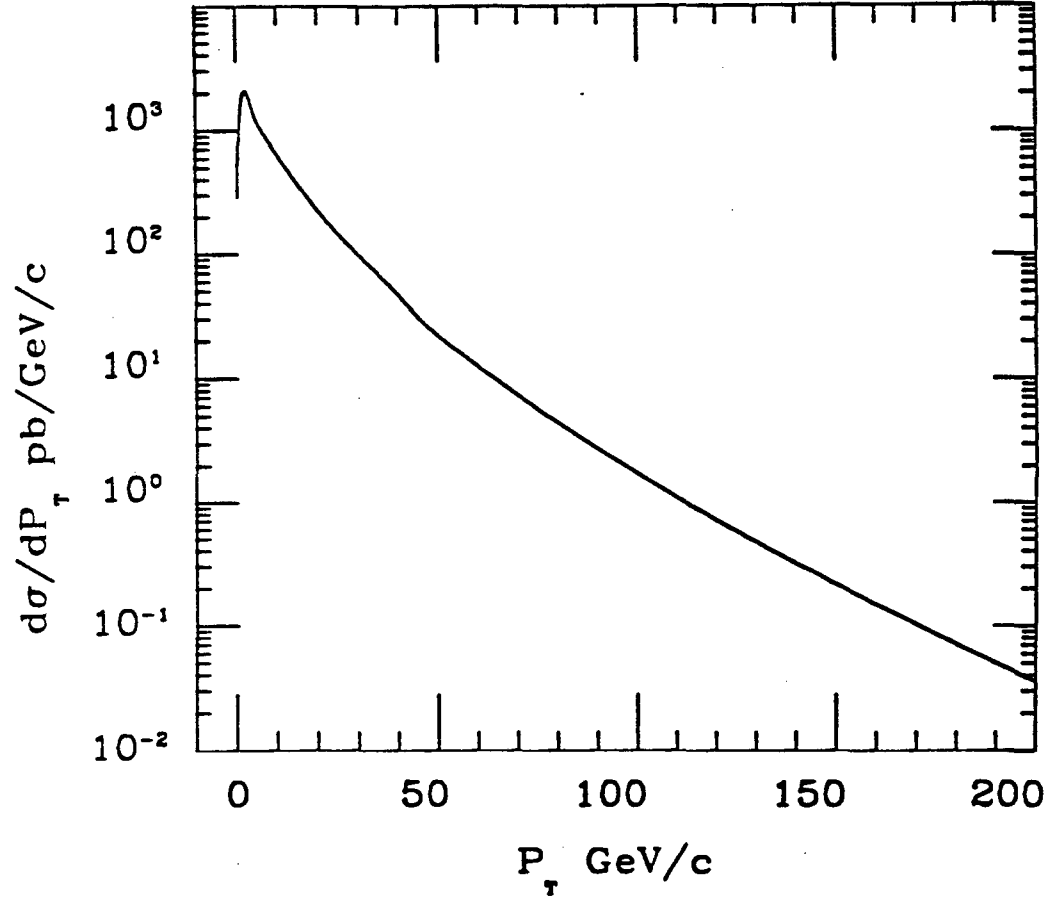
Figure 1.4: The next-to-leading order prediction for W production at Tevatron energies with HMRS(B) structure functions and \Lambda_{QCD} = 190 MeV. The roll over at low P_T is caused by phase space.
