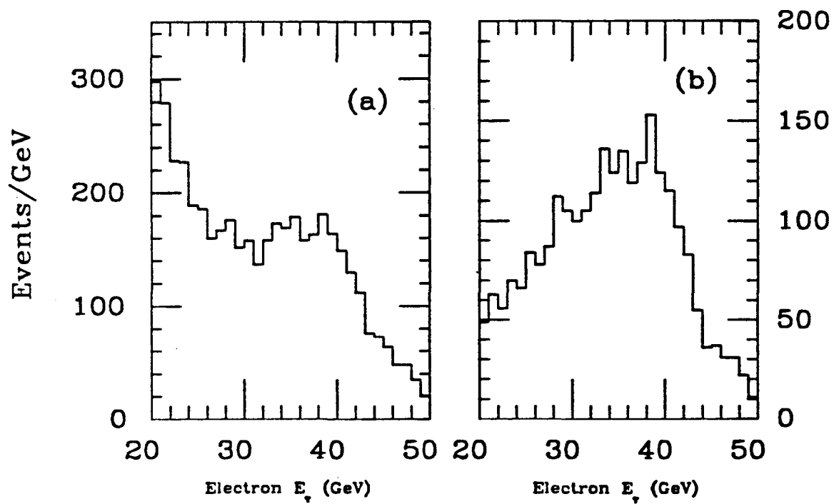
Figure 3.5: The electron E_T spectrum before and after the E_T cut. Plot (a) shows the spectrum before the E_T cut. The peak near 40 GeV contains both W and Z events. Plot (b) shows the spectrum after the E_T > 20 GeV requirement.
