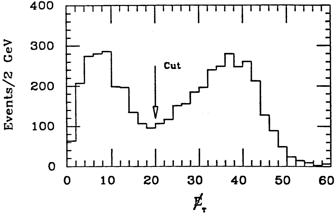
Figure 3.4: The E_T^{\text{miss}} distribution for the high E_T electron sample. The low E_T^{\text{miss}} peak contains Z events and background. The peak near 40 GeV is consistent with what would be expected from W events.
