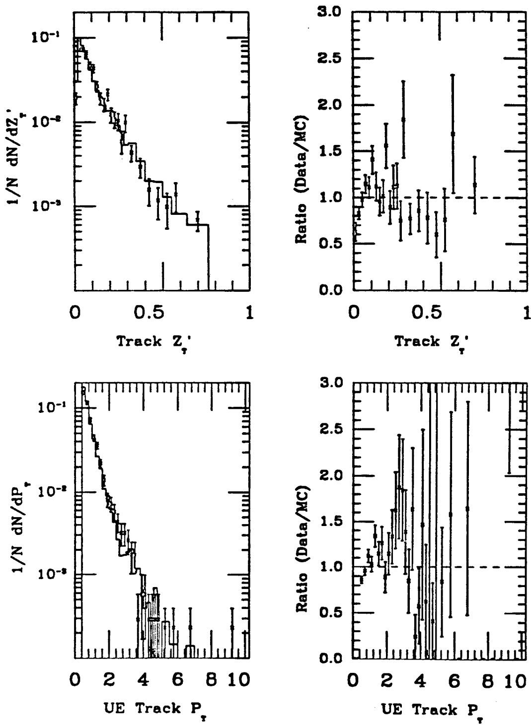
Figure B.4: A comparison between the data and the Monte Carlo fragmentation quantities for the Z_T' and the underlying event Track P_T . The points are the data and the histogram is the prediction from the Monte Carlo program.
