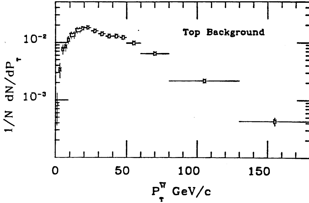
Figure 3.10: The background shape from a heavy top quark decay. The W is real; however, the P_T^W is not created by a process described by QCD. The shape was determined from a Monte Carlo program with detector simulation.
