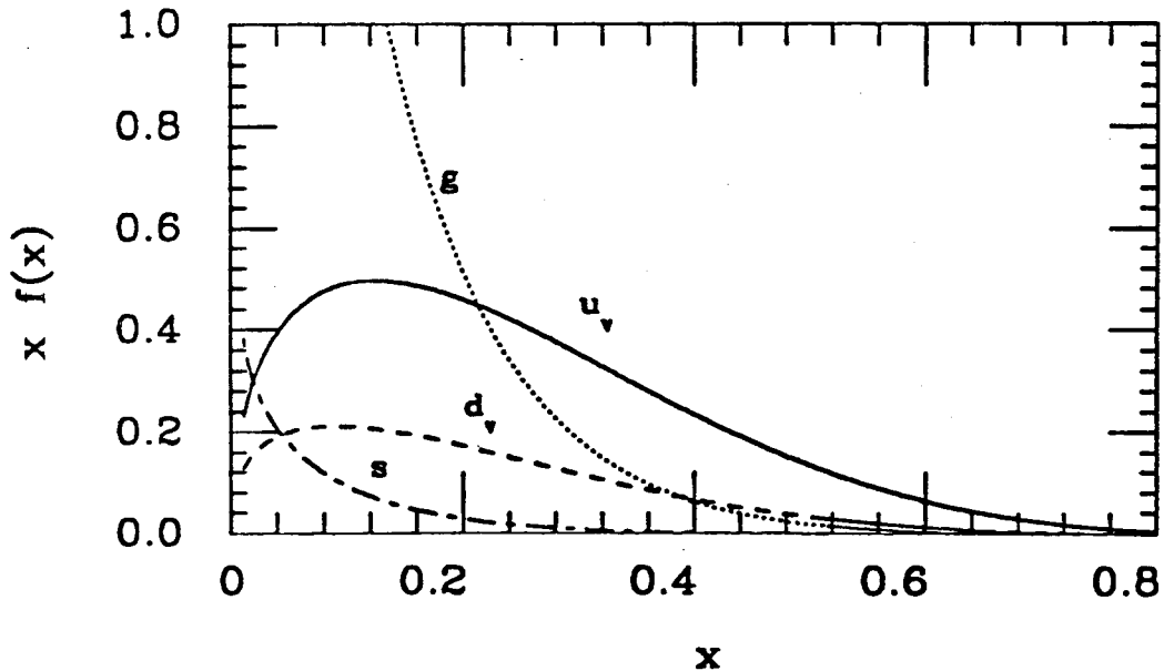
Figure 1.2: The distribution functions, f(x) , represent the probability of finding a quark with momentum fraction x = p/P_{proton} between x and x + dx . The distribution functions are shown for the up, down and strange quarks along with the gluon. EHLQ1 structure functions were used.
