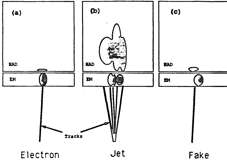
Figure 3.1: Topology of typical electron (a) and typical jet in CDF (b). Unusual jets can mimic an electron topology (c). The shaded areas represent energy deposition in the calorimeters.
