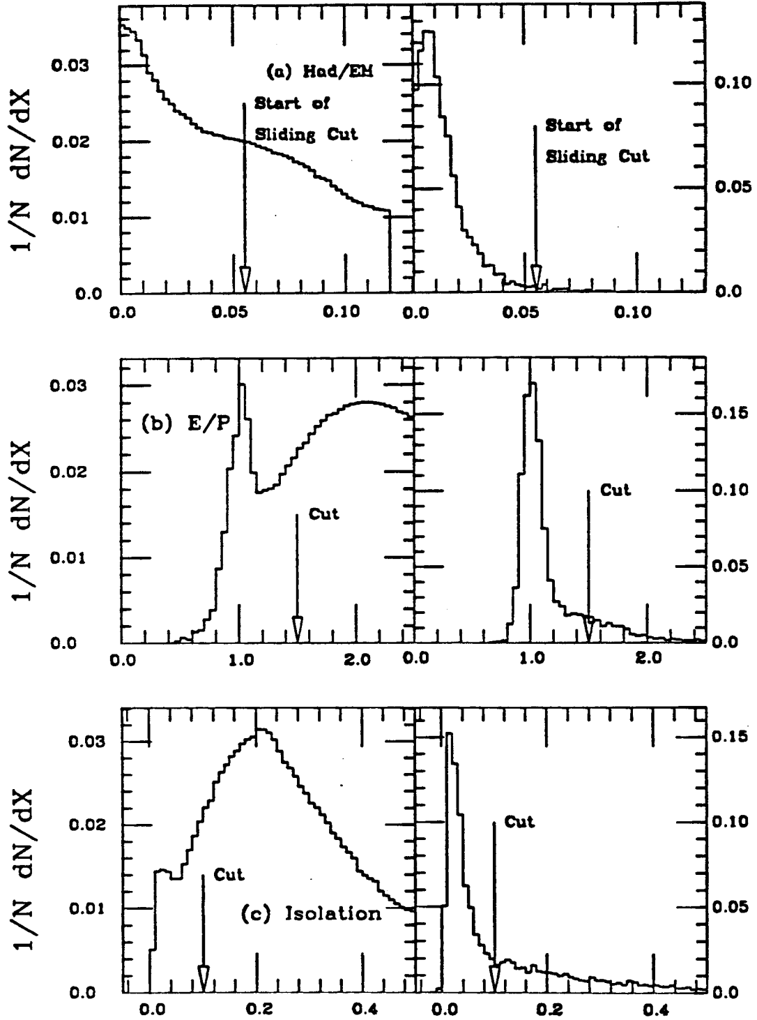
Figure 3.2: Electron Identification Quantities: Each is shown after the Electron trigger requirement and Electron E_T cut and also shown after all identification cuts except the cut specified. The quantities are (a) Had/EM, (b) E/P, (c) Isolation.
