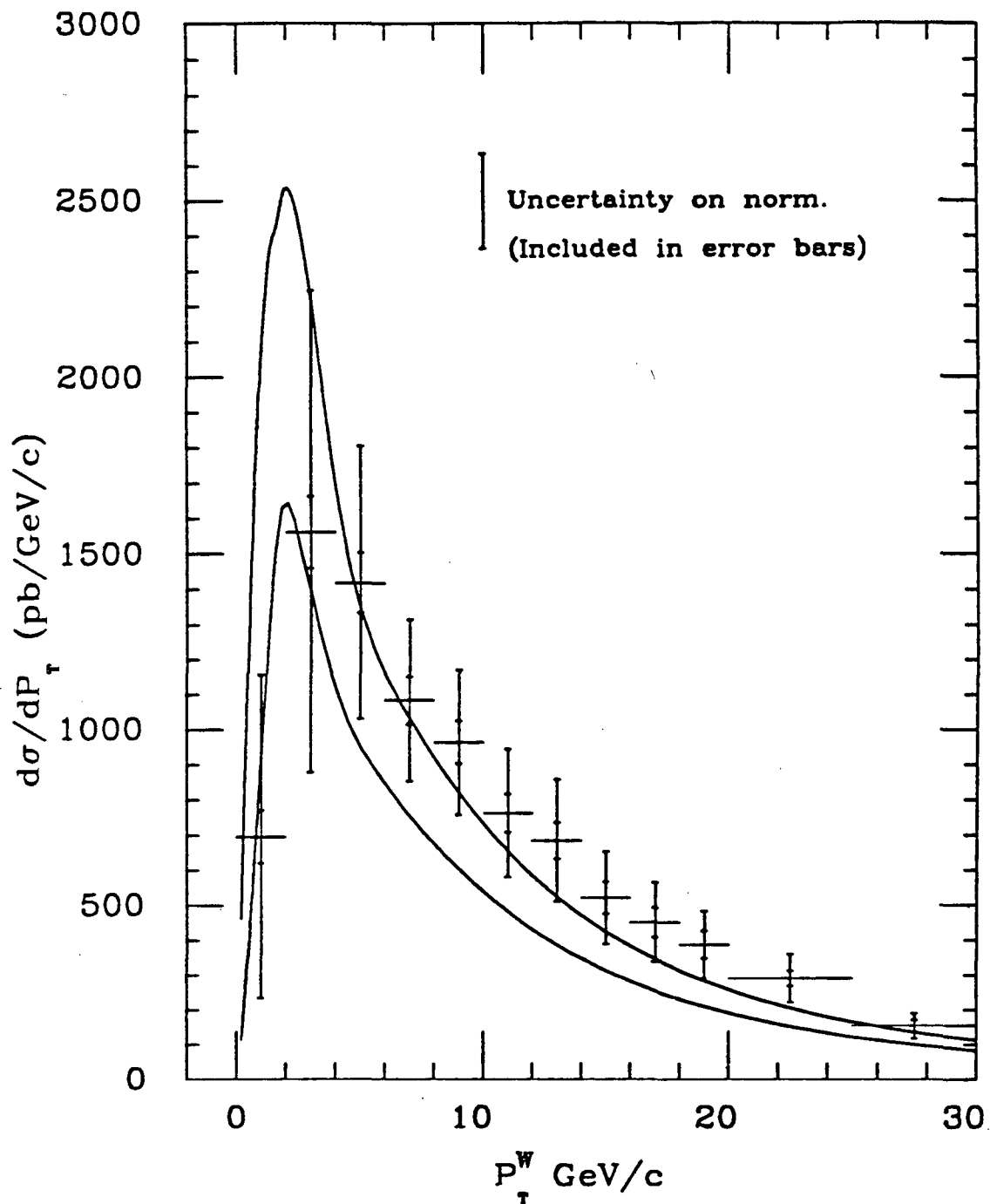
Figure 6.2: Same as Figure 6.1 except for the low P_T range. The low P_T bins are highly correlated and therefore should fluctuate as a unit (see text for more).
