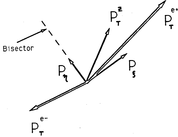
Figure 4.8: Definition of components for the Z analysis. The component P_\eta is less sensitive to mismeasurement of the electrons' E_T than the component P_\xi .
