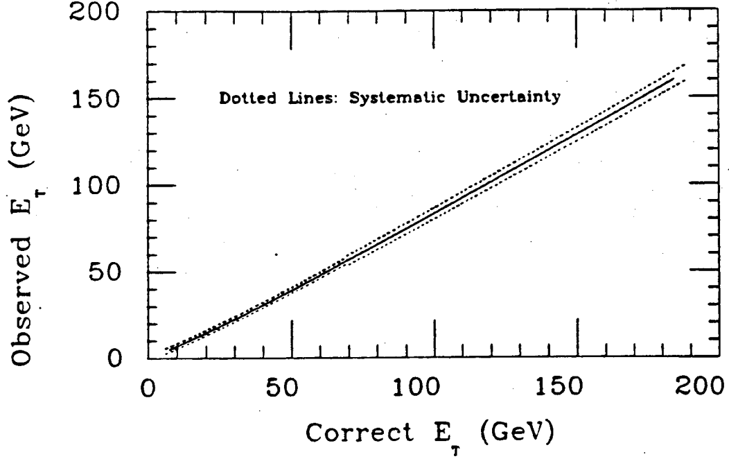
Figure 4.15: Observed Cluster E_T versus Correct E_T with systematic error bands.
