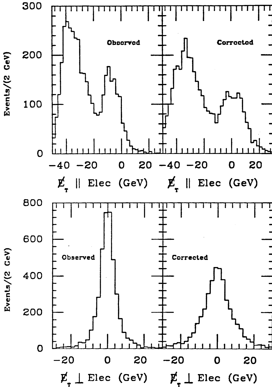
Figure 4.12: The distribution of the \cancel{E}_T perpendicular ( \perp ) and parallel ( \parallel ) to the electron direction for the inclusive electron sample.
