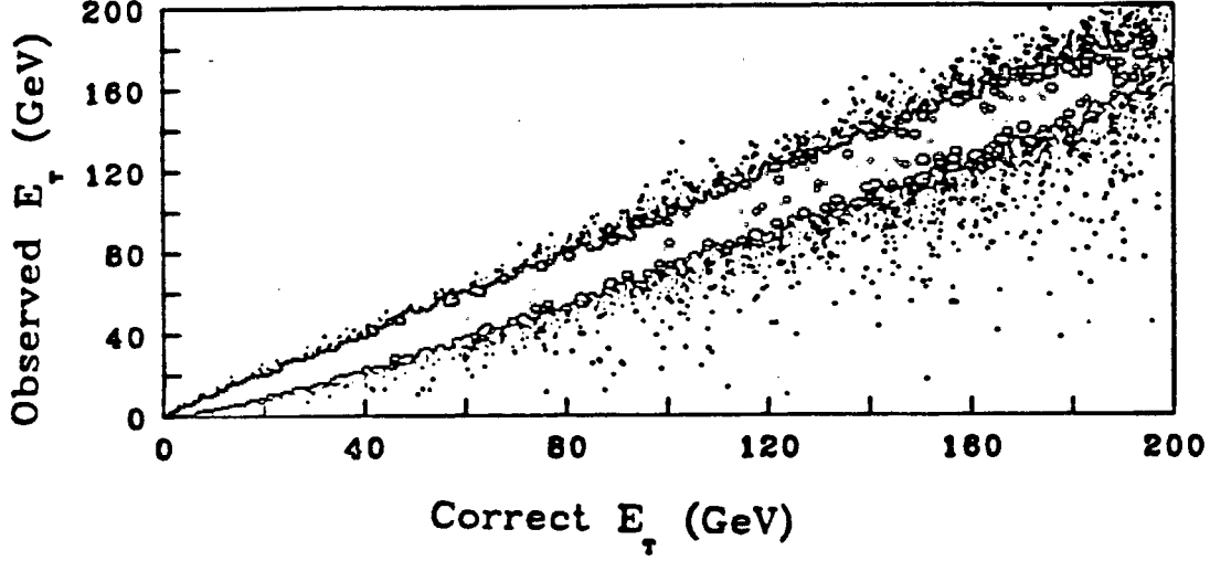
Figure 4.1: A scatter plot of the observed Cluster E_T versus energy generated inside the clustering cone.
