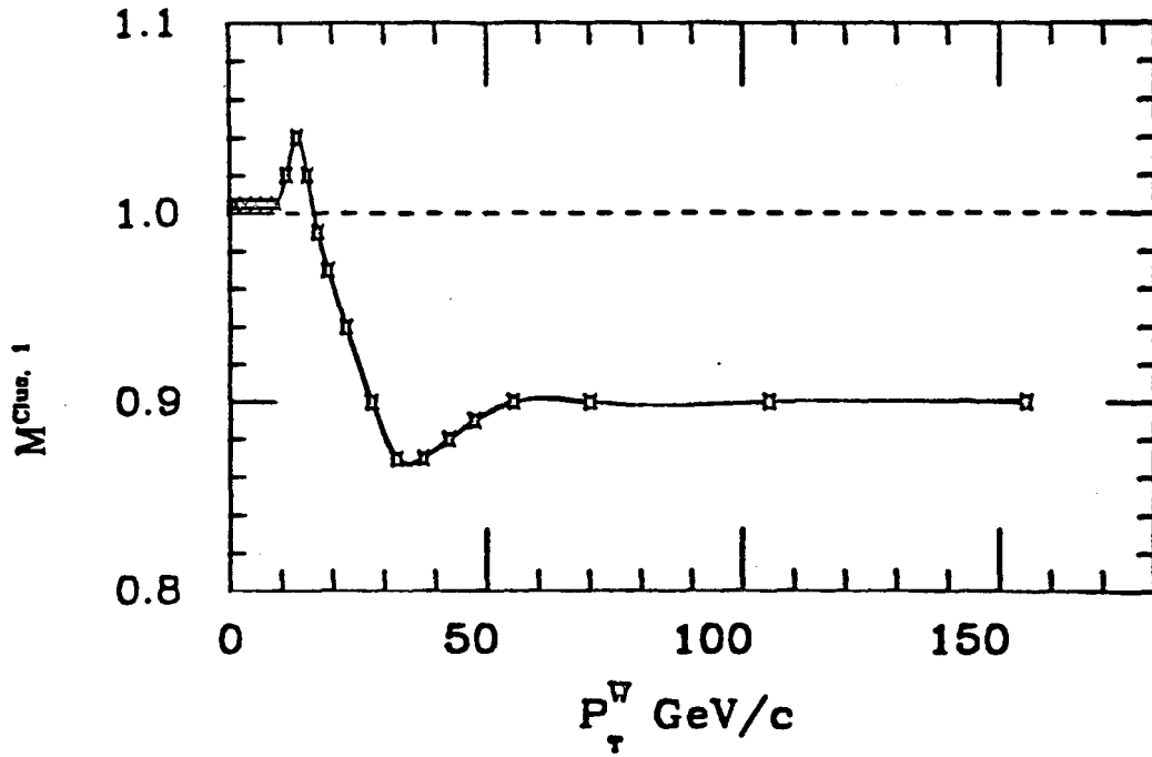
Figure 5.4: Scale factor from the systematic uncertainty of the clustered energy correction offset parameter (C) (see Eq. 4.4).
