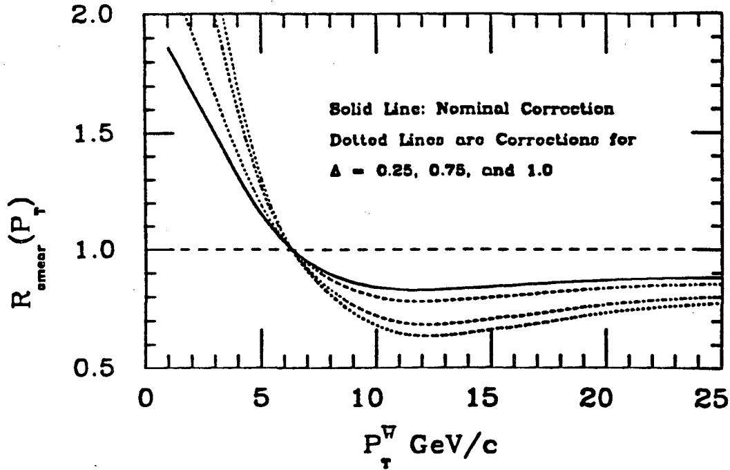
Figure 5.1: Different smearing corrections for different systematic fluctuations of the resolution function.
