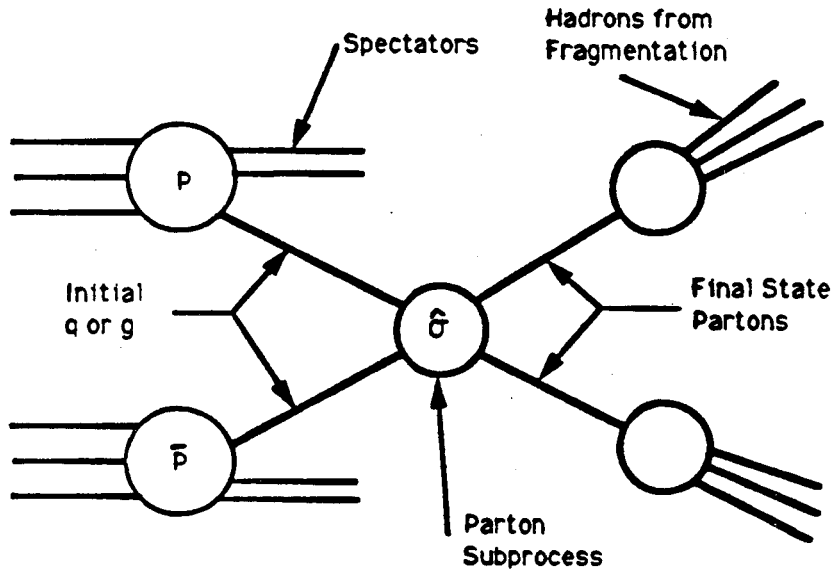
Figure 1.1: At the Tevatron the most interesting events involve an energetic interaction between two constituents of the proton and antiproton. The other partons are called spectators. The products of the interaction fragment into hadrons or in the case of the W boson decay into leptons.
