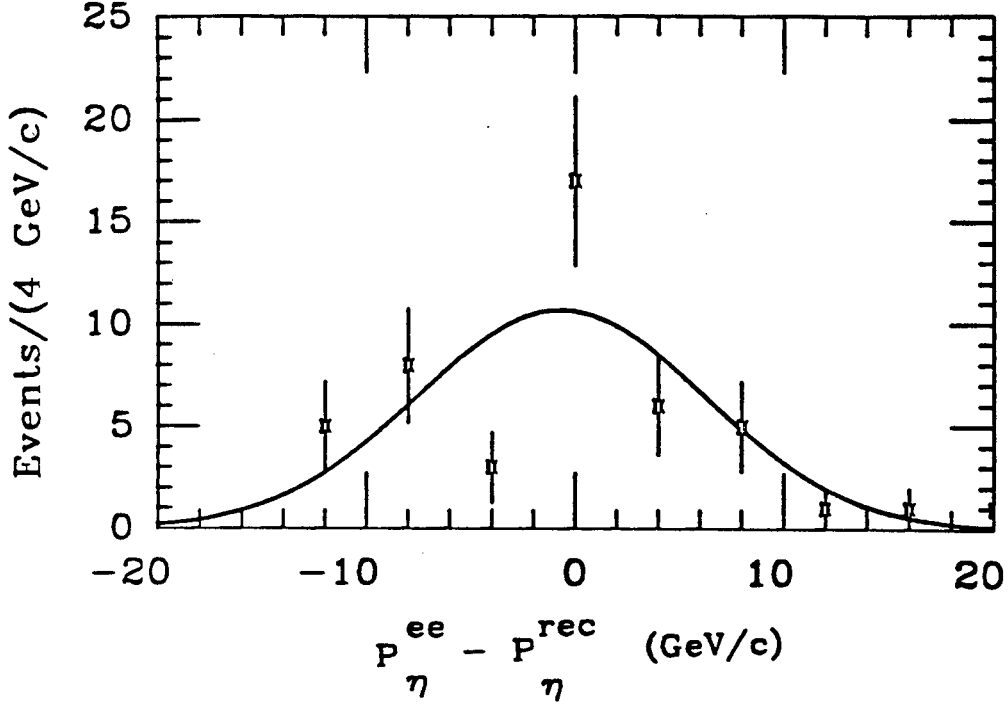
Figure 4.11: Same as Figure 4.10 except the sample contains only Z events with a cluster with E_T > 10 GeV. The mean of the fit is -0.45 \pm 0.97 GeV/c and \sigma = 6.6 GeV/c.
