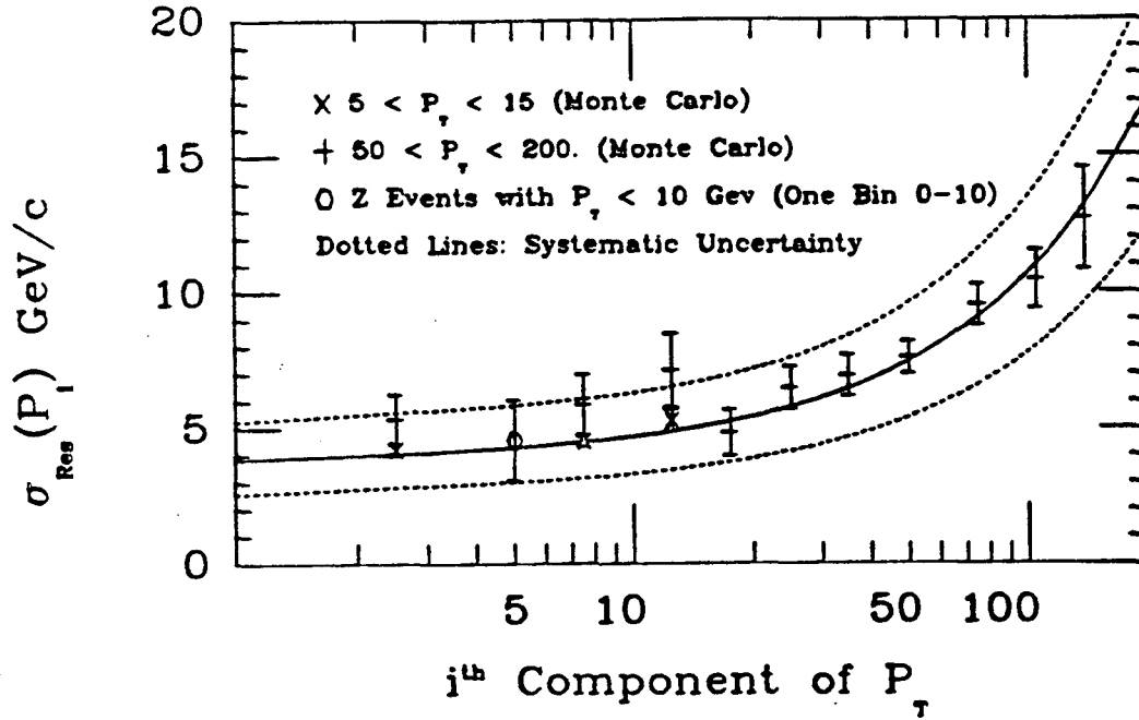
Figure 4.18: The resolution on the component for events in different P_T^W ranges. The resolution on small P_i components for high P_T^W events is slightly worse than low P_T^W events. Also shown is the resolution measured from Z events. It is in good agreement with the simulation.
