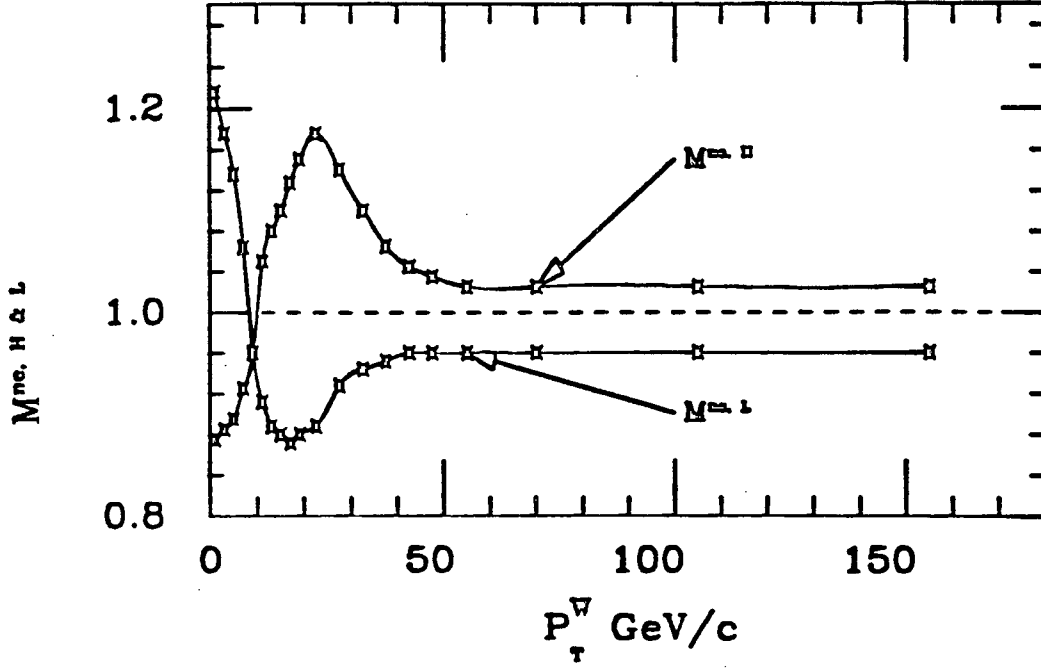
Figure 5.3: Scale factor from systematic uncertainty of non-clustered correction factor cross point to be similar in magnitude to the adjacent points (see Figure 5.2).
