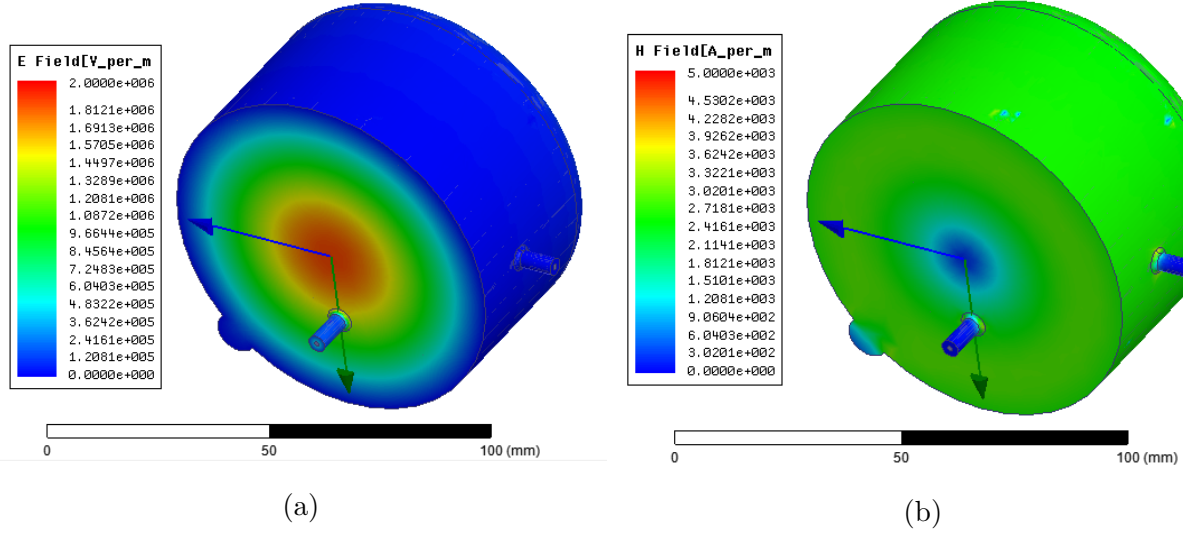
Figure 3.19: Surface electric and magnetic TM_{010} fields of the S-band cavity. Fields are normalized to 1 mJ stored energy.
