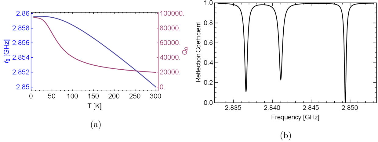
Figure 3.26: (a) Expected temperature dependence of f_0 (blue) and Q_0 (purple) for the \pi mode frequency in the S-band cryogenic single cell structure. (b) Expected results from a frequency scan for the S-band single cell cavity from a network analyzer. Expected Q_0 is adapted from the S-band cryogenic pillbox results. Expected f_0 is from the expected thermal expansion of copper.
