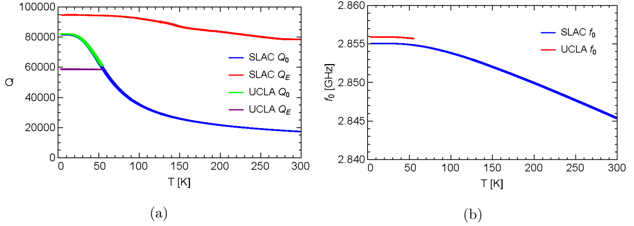
Figure 3.21: Rf parameter measurements from the temperature scan. (a) shows the Q_0 and Q_E for both the SLAC and UCLA cavities. (b) shows the f_0 . The thickness of the lines are the error bars from fitting to the VNA data.
