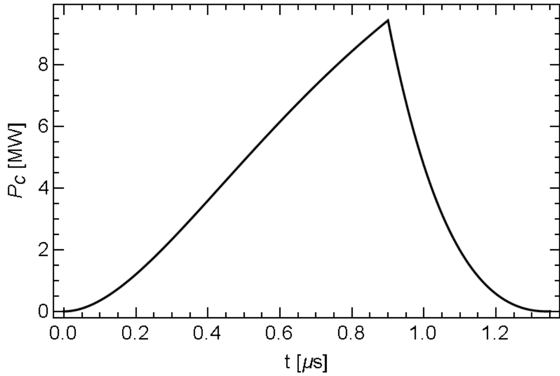
Figure 5.8: Power deposited inside the cavity for a single rf pulse, with pulse length 1.35\mu s , where the phase flip occurs at 0.9\mu s , and a power of 50 MW.
