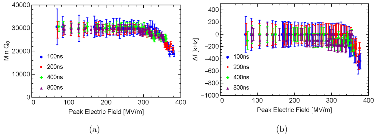
Figure 4.5: (a) final Q_0 and (b) frequency shift for T=45 K, repetition rate 30 Hz for multiple pulse lengths. There is no obvious difference between the four data sets.
