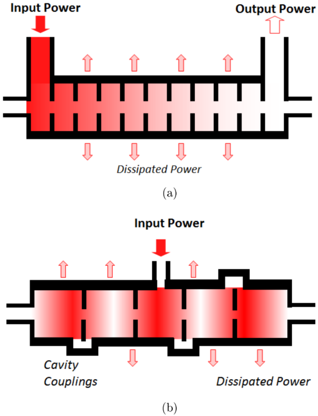
Figure 1.4: Conceptual diagrams of a (a) TW and (b) SW linac. In a TW linac the rf power flows from the input to the output, and is attenuated along the structure. In a SW linac, the input rf power creates a stationary wave. Power is lost to resistive losses in the walls or is reflected out of the input port. Image courtesy [13].
