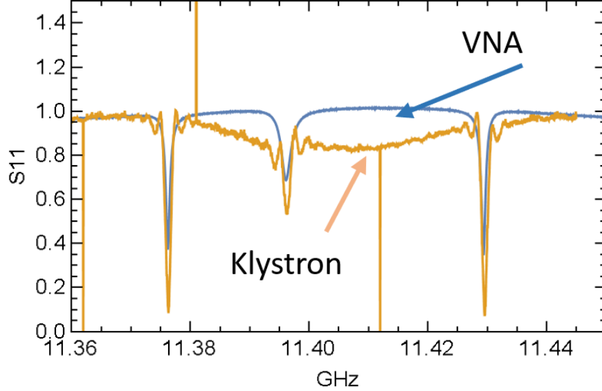
Figure 3.15: Frequency scan of the reflection coefficient using the klystron and VNA.
