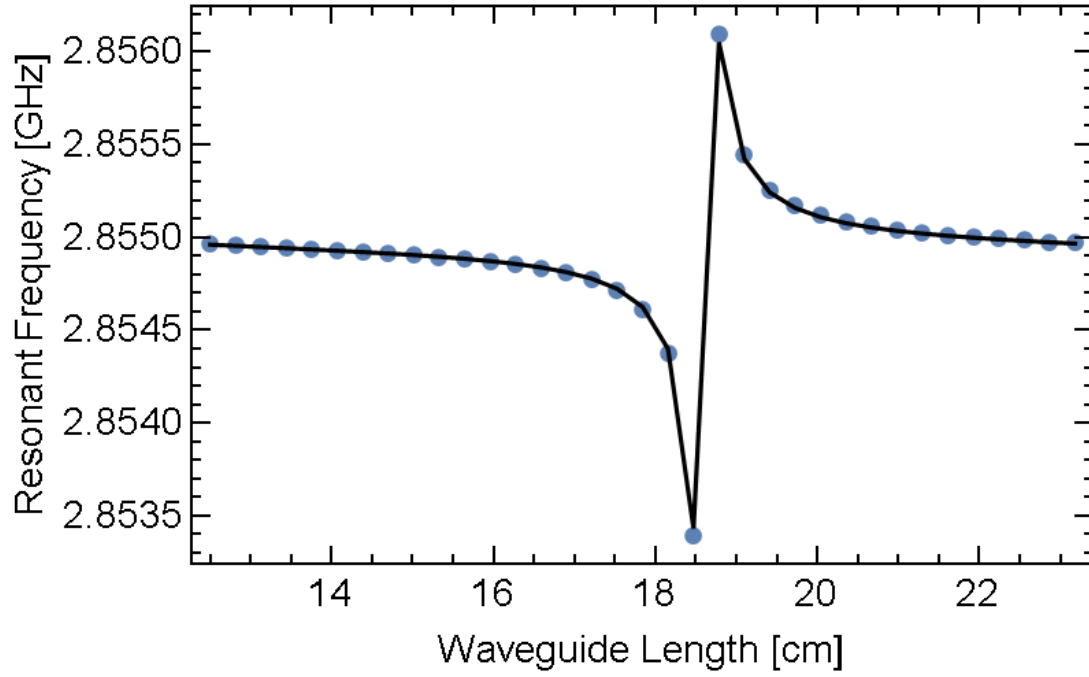
Figure 5.3: Graph shows resonant frequency versus waveguide length, with data from simulations as the blue points. The line is a fit to the data, used to find the Q_E of the system. The parameters for this example are Q_E = 19,400 , f_0 = 2.855 GHz, and \phi = 4.38 rad.
