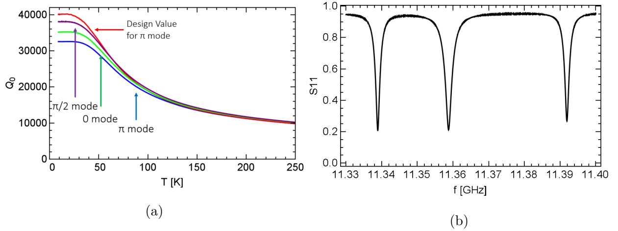
Figure 3.13: (a) Q_0 for the three modes of 1C-SW-A2.75-T2.0-Cryo-Cu-SLAC-#2, and the design value for the \pi mode. (b) Measured S_{11} for all three modes of 1C-SW-A2.75-T2.0-Cryo-Cu-SLAC-#2 at room temperature measured by a VNA.
