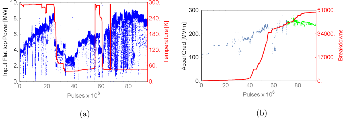
Figure 4.13: The processing history for 1C-SW-A2.75-T2.0-Cryo-Cu-SLAC-#2. (a) Blue is the input flat power and red is the temperature. (b) Red is the cumulative number of recorded breakdowns. Blue is the gradient from the linear model at a breakdown while the structure is processing, and the green shows the calculated gradient from the nonlinear model during measurements of the rf breakdown rate, with 150 ns flat gradient
